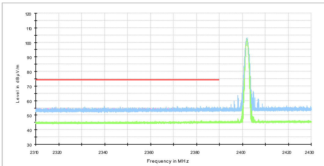
— FCC PART 15 BE_PK — Preview Result1-PK+ - - - FCC PART 15 BE_AVG — Preview Result2-RMS
