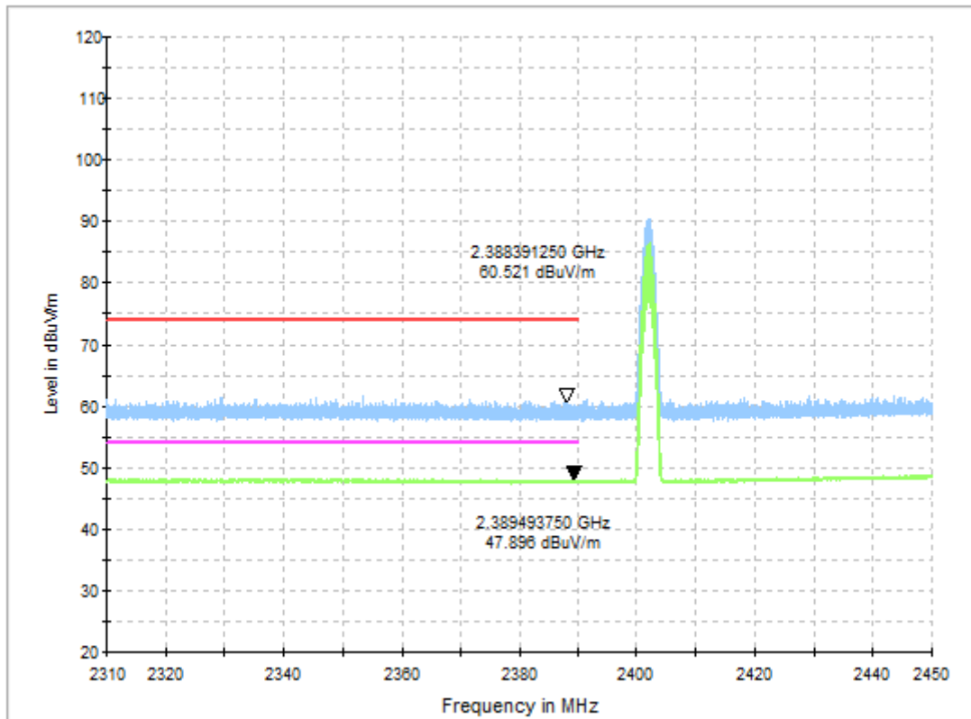
Fig.62. Frequency Band Edges: 8DPSK, Channel 0, 2.31 GHz - 2.45GHz
