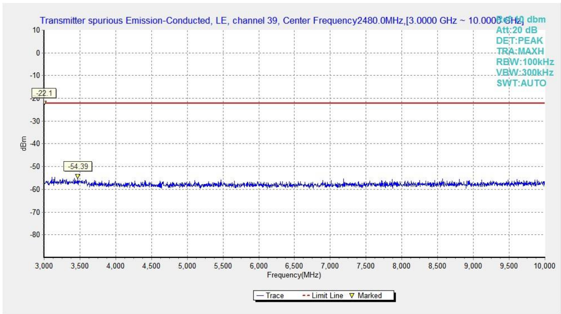
Fig.22. Transmitter Spurious Emission - Conducted: GFSK, 2480 MHz, 3GHz - 10GHz
