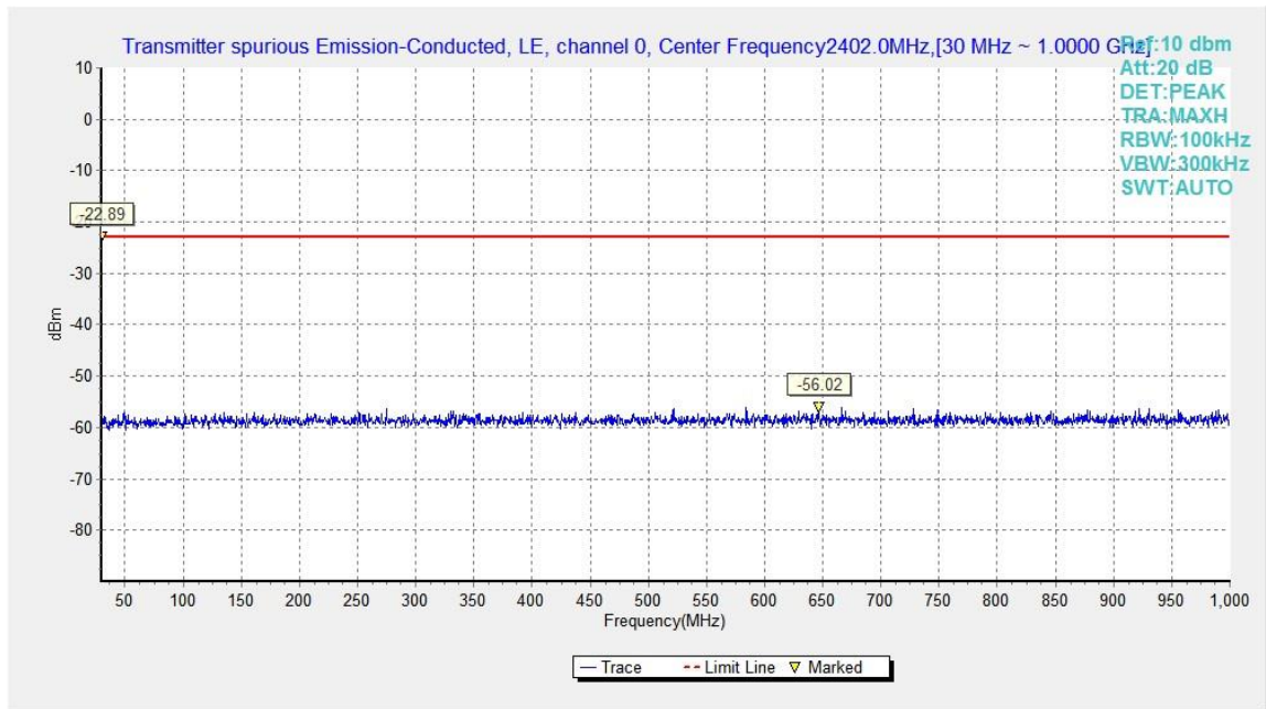
Fig.10. Transmitter Spurious Emission - Conducted: GFSK, 2402 MHz, 30MHz - 1GHz
