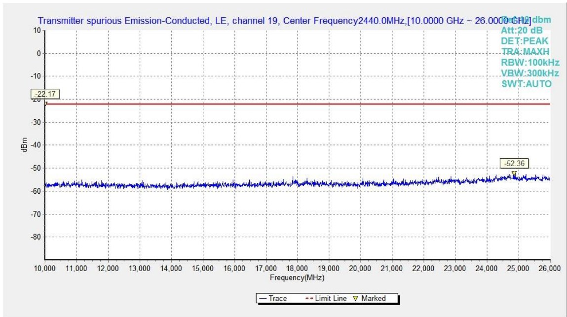
Fig.18. Transmitter Spurious Emission - Conducted: GFSK, 2440 MHz, 10GHz – 26GHz
