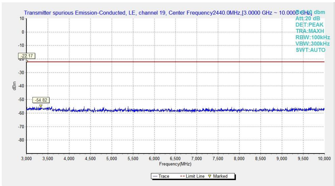
Fig.17. Transmitter Spurious Emission - Conducted: GFSK, 2440 MHz, 3GHz – 10GHz
