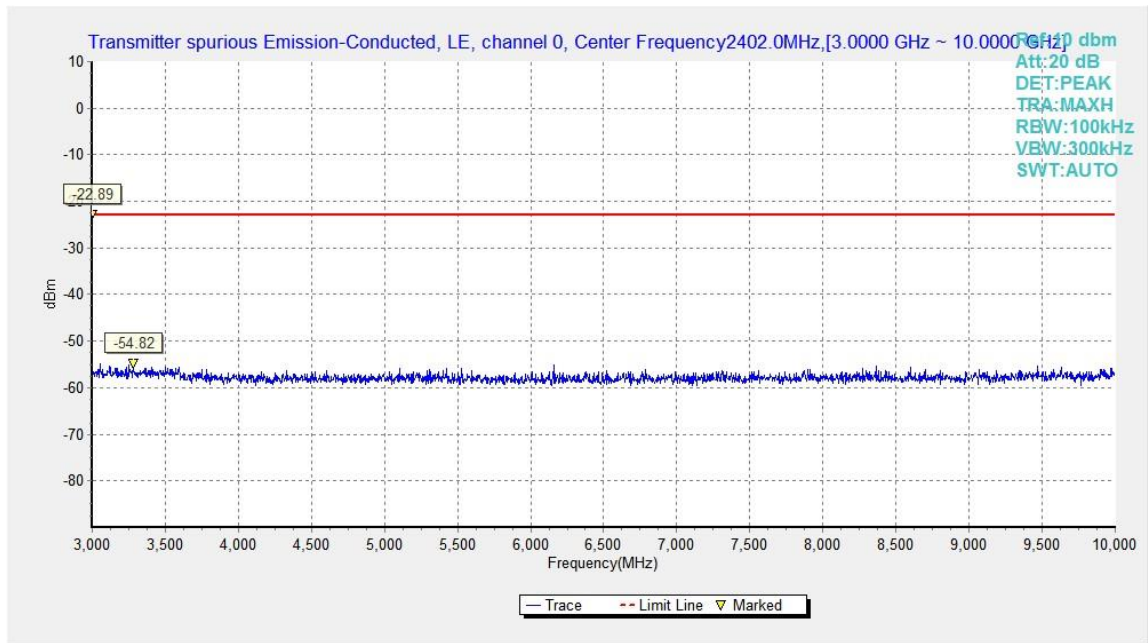
Fig.12. Transmitter Spurious Emission - Conducted: GFSK, 2402 MHz, 3GHz - 10GHz
