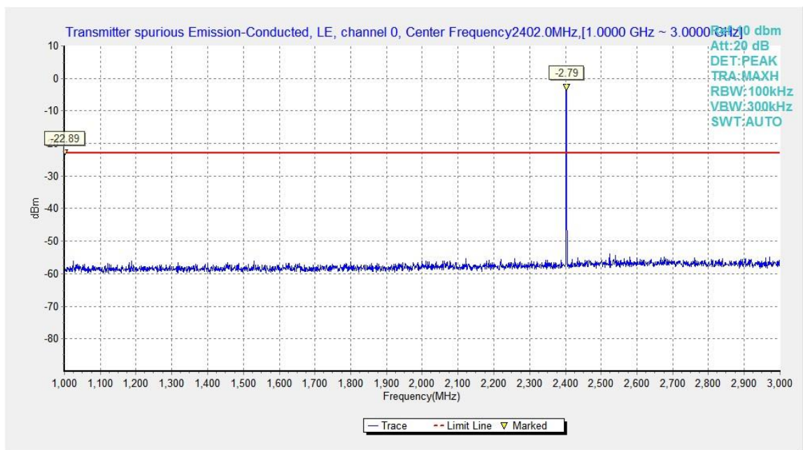
Fig.11. Transmitter Spurious Emission - Conducted: GFSK, 2402 MHz, 1GHz - 3GHz
