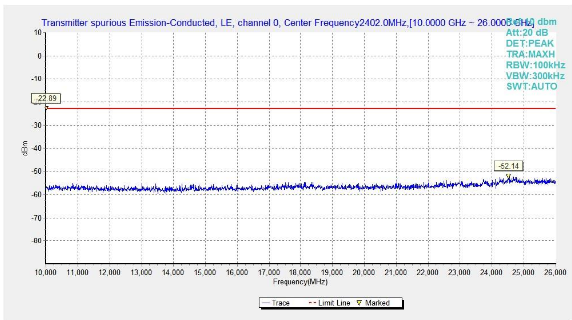
Fig.13. Transmitter Spurious Emission - Conducted: GFSK, 2402 MHz, 10GHz - 26GHz
