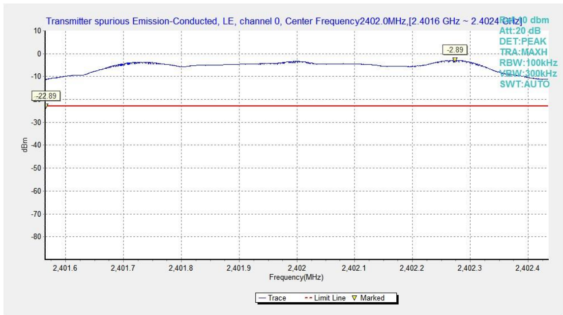
Fig.9. Transmitter Spurious Emission - Conducted: GFSK,2402MHz
