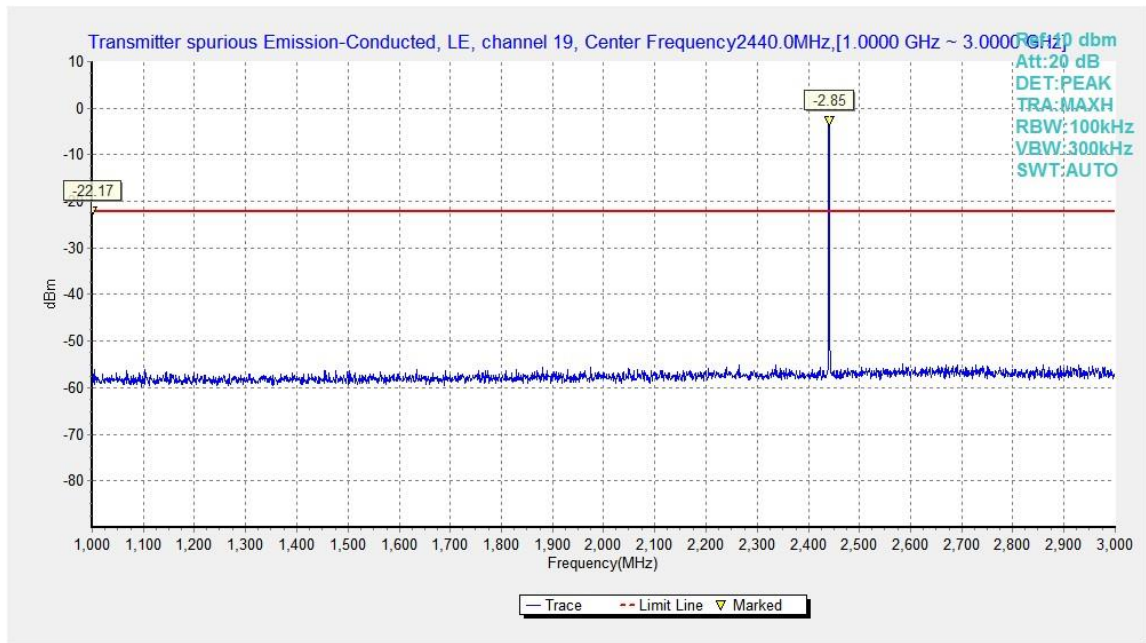
Fig.16. Transmitter Spurious Emission - Conducted: GFSK, 2440 MHz, 1GHz – 3GHz
