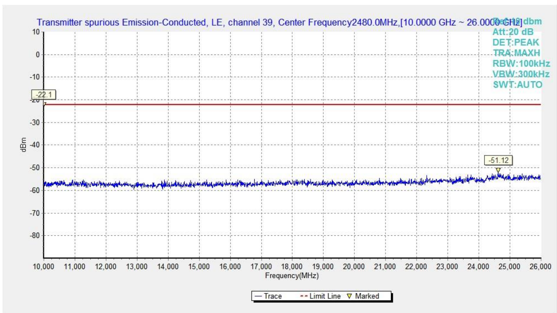
Fig.23. Transmitter Spurious Emission - Conducted: GFSK, 2480 MHz, 10GHz - 26GHz
