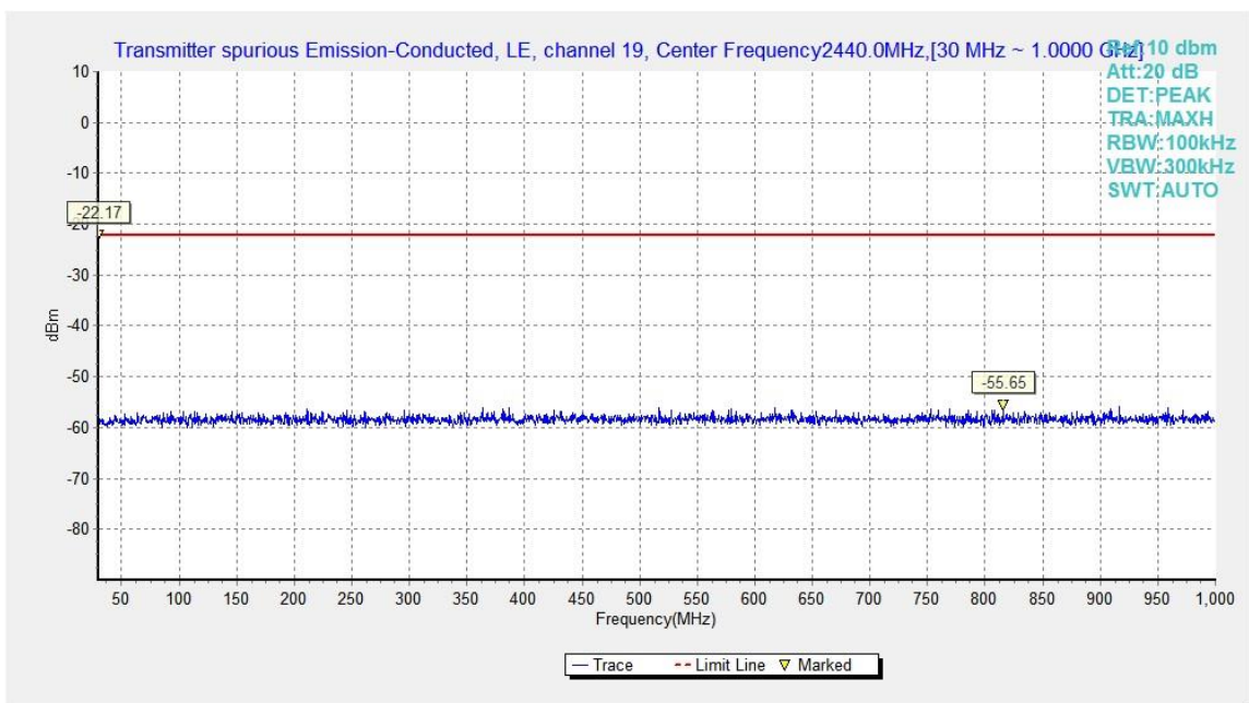
Fig.15. Transmitter Spurious Emission - Conducted: GFSK, 2440 MHz, 30MHz - 1GHz
