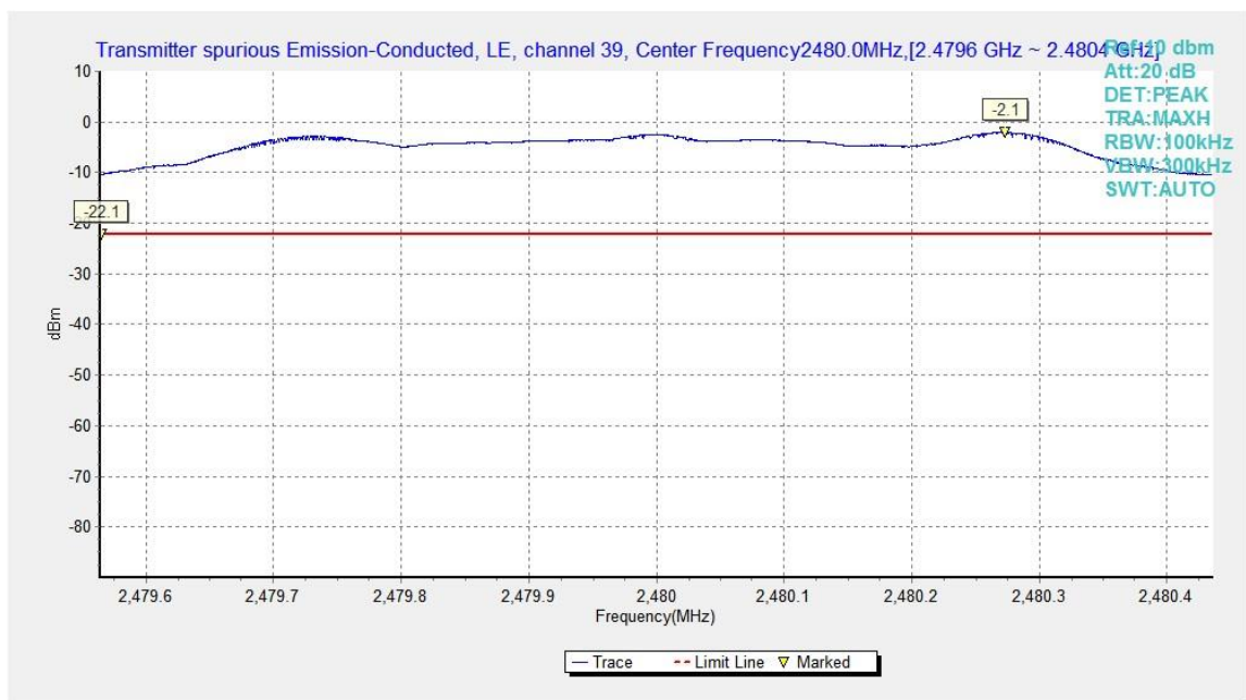
Fig.19. Transmitter Spurious Emission - Conducted: GFSK, 2480 MHz
