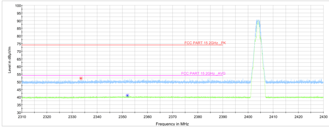
Fig.24. Frequency Band Edges: GFSK, 2404 MHz, Hopping Off, 2.31 GHz – 2.43GHz
