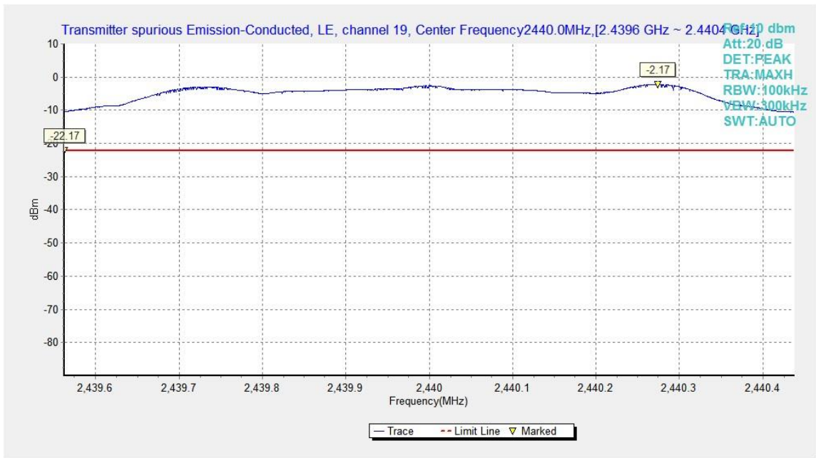
Fig.14. Transmitter Spurious Emission - Conducted: GFSK, 2440MHz
