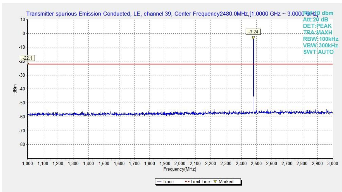
Fig.21. Transmitter Spurious Emission - Conducted: GFSK, 2480 MHz, 1GHz - 3GHz
