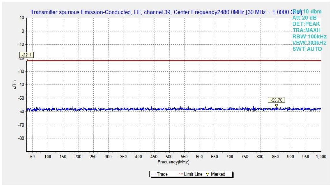
Fig.20. Transmitter Spurious Emission - Conducted: GFSK, 2480 MHz, 30MHz - 1GHz
