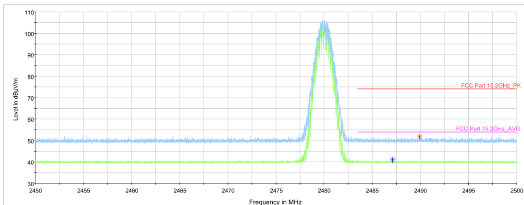
Fig.68. Frequency Band Edges: GFSK, Channel 78, Hopping Off, ch11, 2.45 GHz - 2.50GHz
