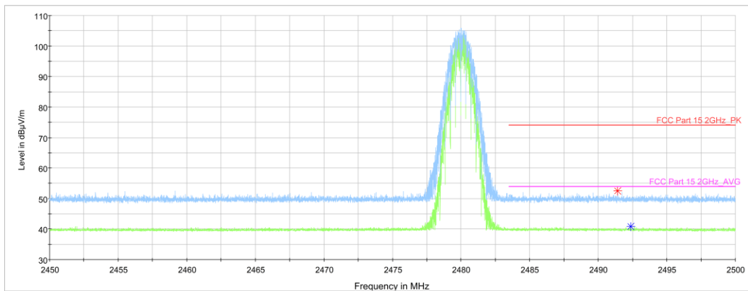
Fig.70. Frequency Band Edges: \pi/4 DQPSK, Channel 78, Hopping Off, 2.45 GHz - 2.50GHz
