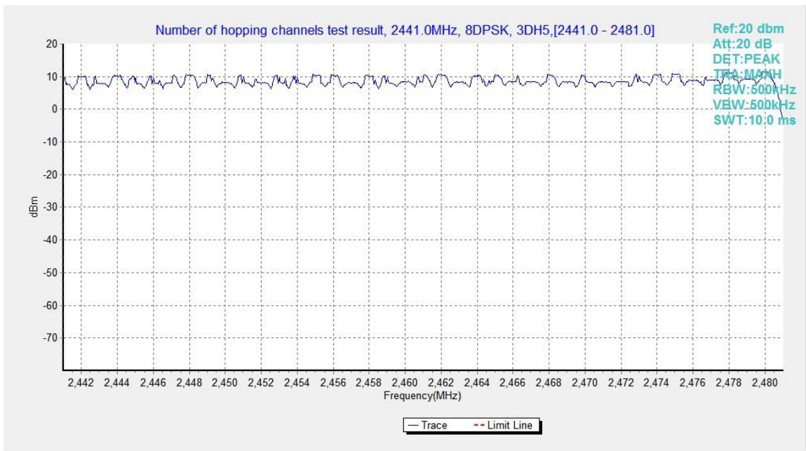
Fig.108. Number of hopping frequencies: 8DPSK, Channel 40 - 78
