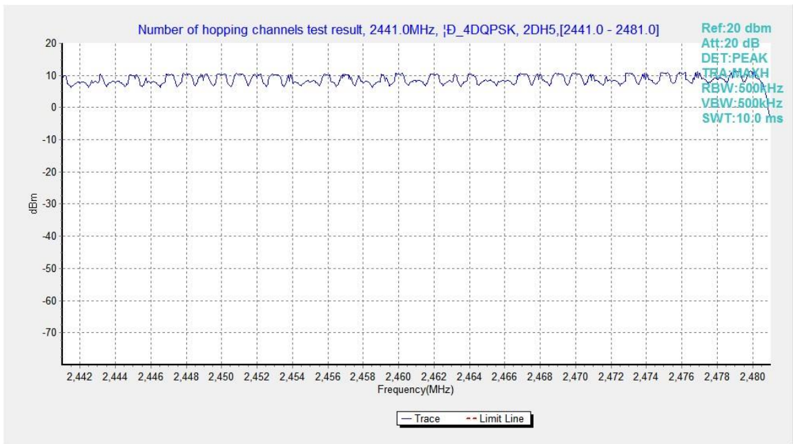
Fig.106. Number of hopping frequencies: \pi/4 DQPSK, Channel 40 - 78
