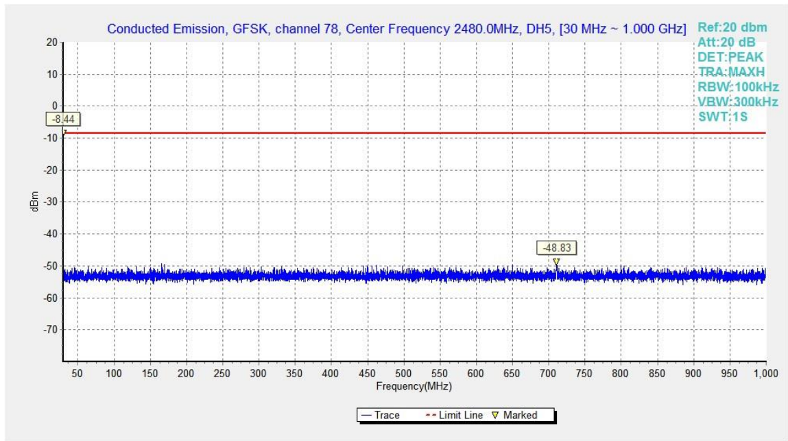
Fig.33. Conducted spurious emission: GFSK, Channel 78, 30MHz - 1GHz
