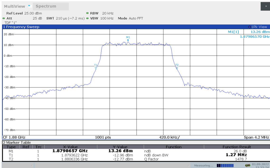
LTE band 2, 1.4MHz Bandwidth, 64QAM (-26dBc BW)
