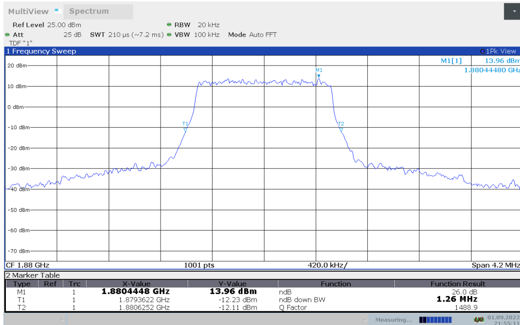
LTE band 2, 1.4MHz Bandwidth, 16QAM (-26dBc BW)
