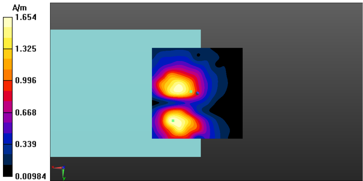
Fig A.21 T-Coil WLAN 5.5GHz-Y
