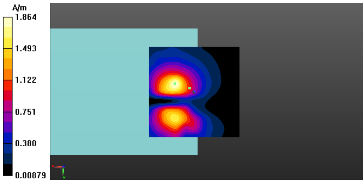
Fig A.17 T-Coil LTE-Band 5-Y
