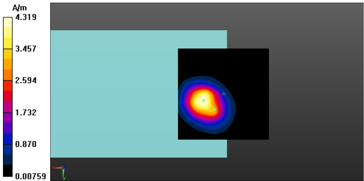
Fig A.17 T-Coil LTE-Band 5-Z
