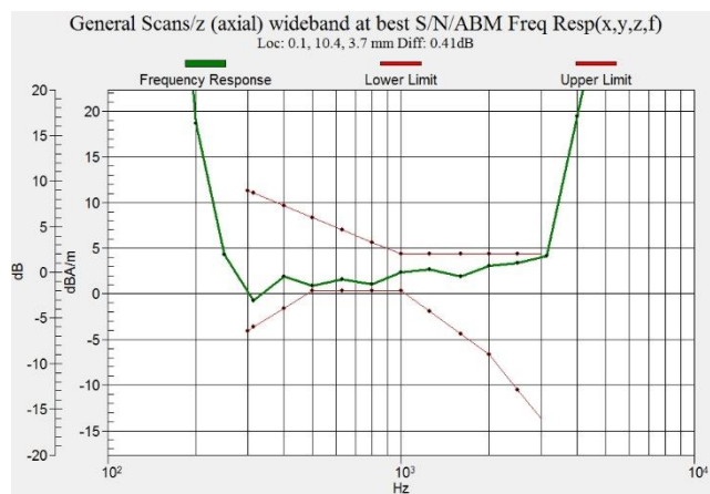
Figure C.2 Frequency Response of EDGE 1900 - OTT VoIP
