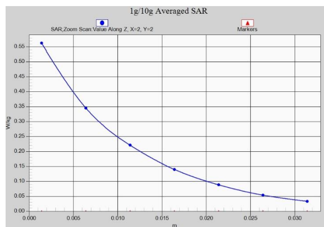
Fig. A-29 Z-Scan at power reference point (LTE Band66)
