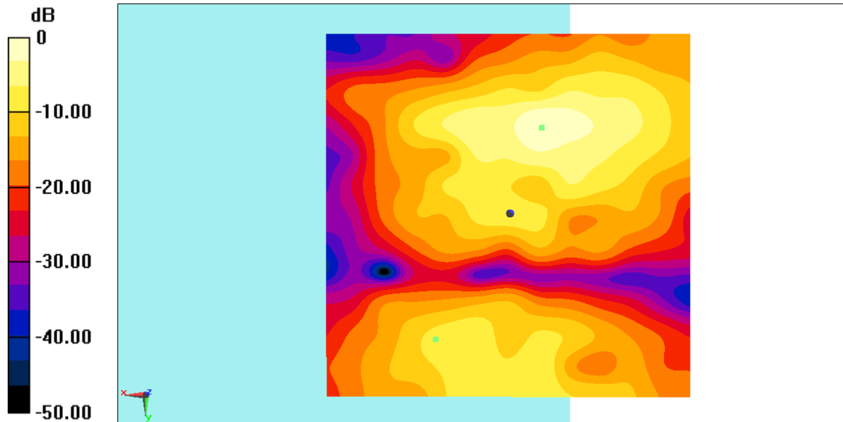
Fig B.1 T-Coil LTEB41
