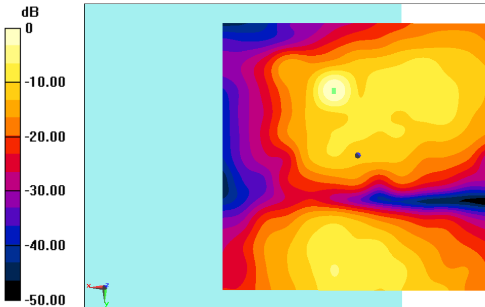
Fig B.3 T-Coil LTEB41-OTT
