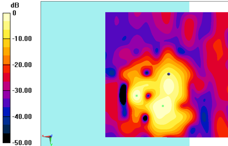
Fig B.4 T-Coil GSM1900-OTT
