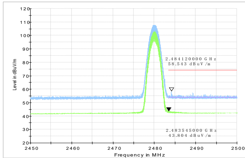
Fig.18. Frequency Band Edges: 8DPSK, Channel 78, 2.45 GHz - 2.50GHz
