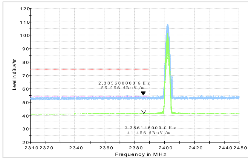
Fig.17. Frequency Band Edges: 8DPSK, Channel 0, 2.31 GHz - 2.45GHz
