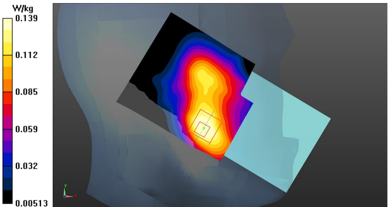
Fig.3 GSM1900 Head
