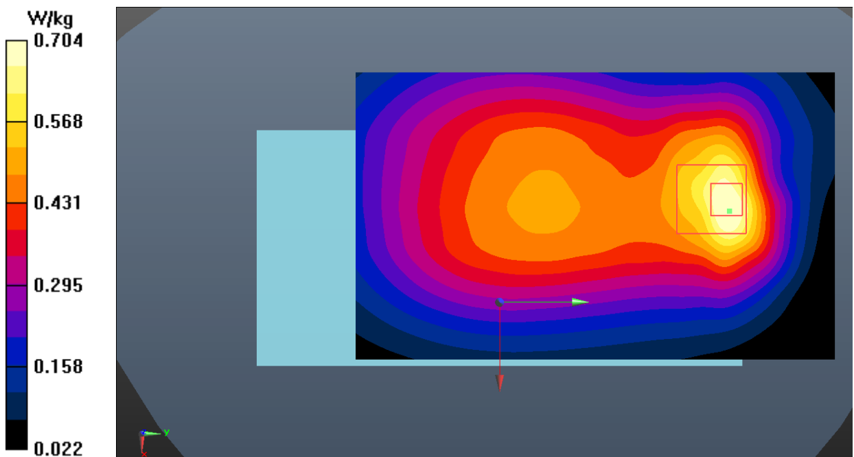
Fig.2 GSM850 Body
