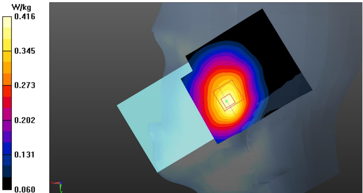
Fig.1 GSM850 Head
