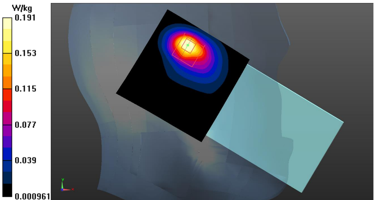
Fig.27 Bluetooth Head
