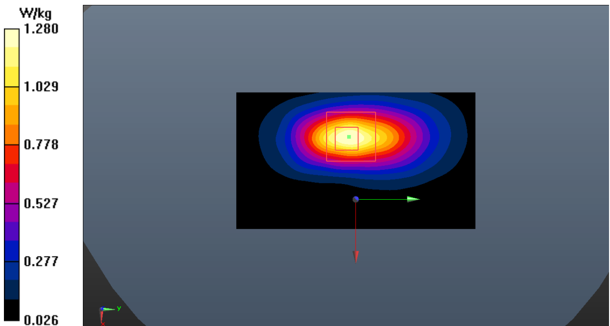
Fig.4 GSM1900 Body
