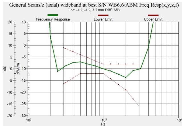
Figure C.5 Frequency Response of WCDMA850 - OTT VoIP
