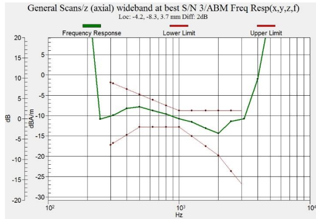
Figure C.7 Frequency Response of LTE B41 PC3 – OTT VoIP
