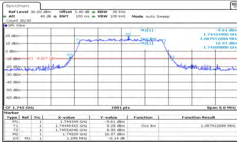
Band66-1.4MHz-QPSK-132322-6RB#0-1.088
