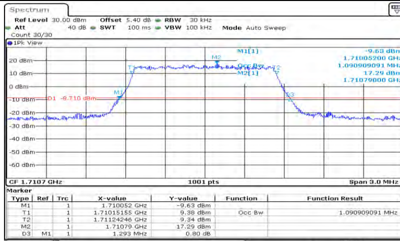
Band66-1.4MHz-QPSK-131979-6RB#0-1.091
