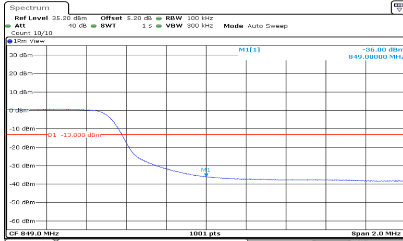
Band 26_10MHz_16QAM_26990_50RB#0
