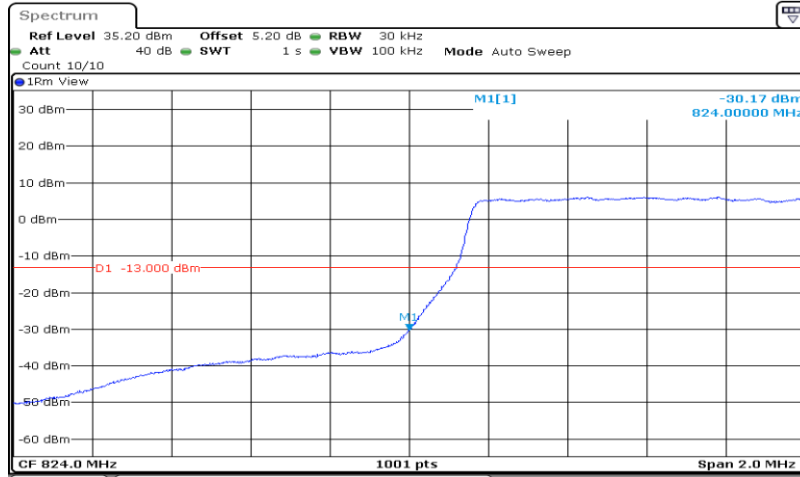
Band 26_1.4MHz_16QAM_26797_6RB#0
