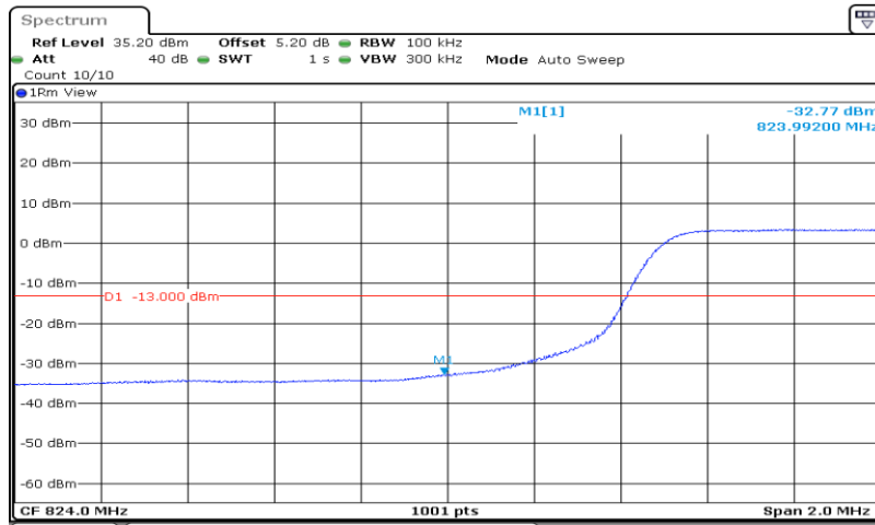
Band 26_10MHz_16QAM_26840_50RB#0
