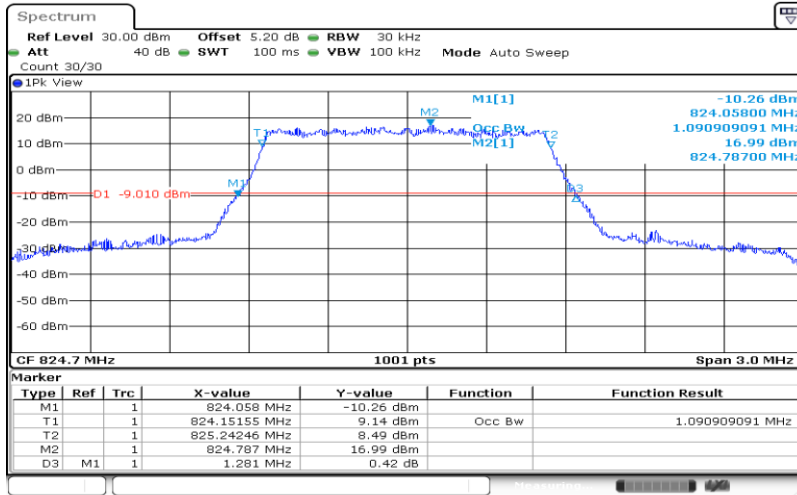
Band26-1.4MHz-QPSK-26797-6RB#0-1.091
