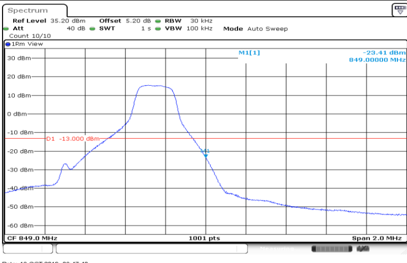
Band 26_1.4MHz_QPSK_27033_6RB#0
