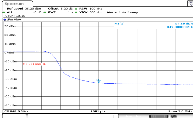
Band 26_10MHz_QPSK_26990_50RB#0
