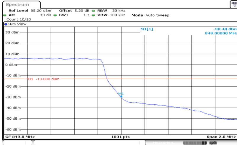
Band 26_1.4MHz_16QAM_27033_6RB#0
