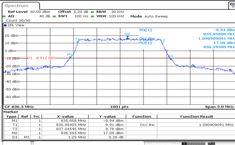
Band26-1.4MHz-QPSK-26915-6RB#0-1.091
