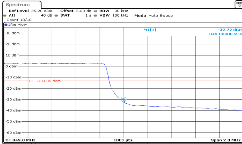
Band 26_3MHz_QPSK_27025_15RB#0
