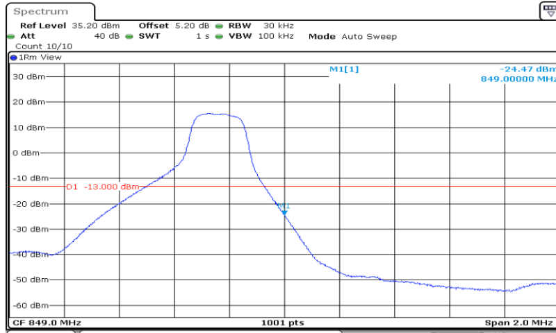
Band 26_3MHz_QPSK_27025_15RB#0
