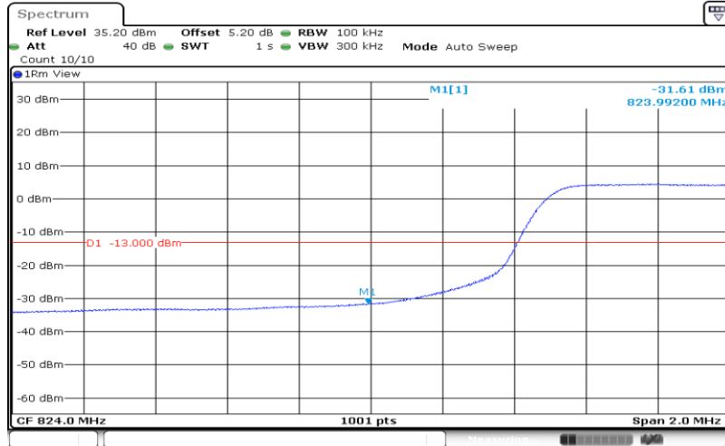
Band 26_10MHz_QPSK_26840_50RB#0
