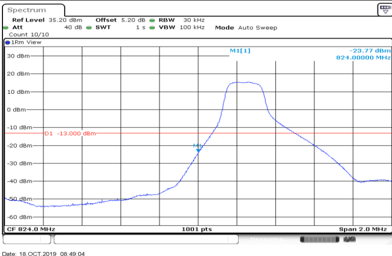
Band 26_3MHz_QPSK_26805_15RB#0
