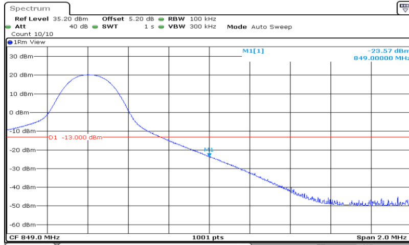
Band 26_10MHz_QPSK_26990_50RB#0
