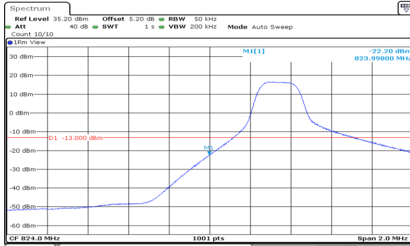
Band 26_5MHz_16QAM_26815_25RB#0
