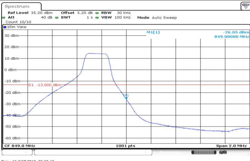
Band 26_3MHz_16QAM_27025_15RB#0
