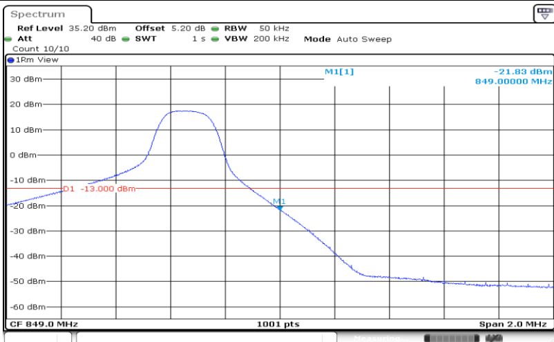
Band 26_5MHz_QPSK_27015_25RB#
