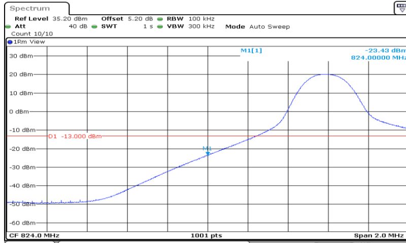
Band 26_10MHz_QPSK_26840_50RB#0
