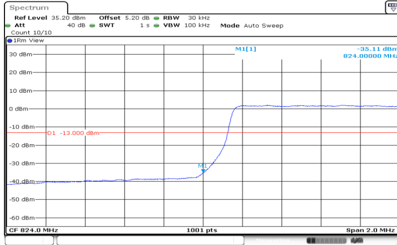
Band 26_3MHz_16QAM_26805_15RB#0
