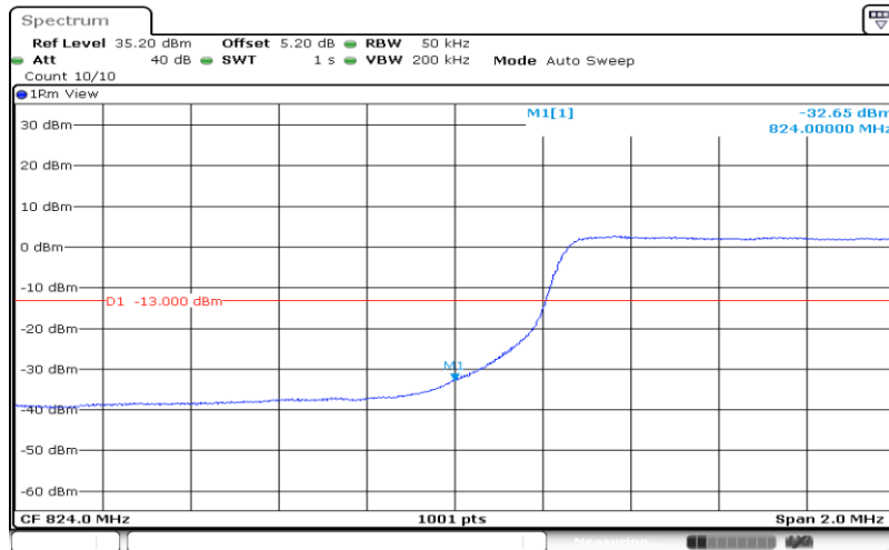
Band 26_5MHz_16QAM_26815_25RB#0
