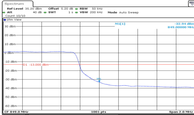
Band 26_5MHz_16QAM_27015_25RB#0
