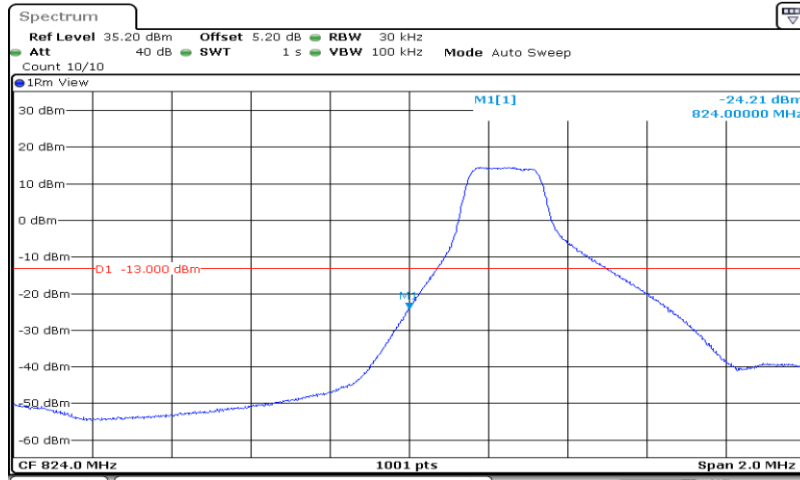
Band 26_3MHz_16QAM_26805_15RB#0
