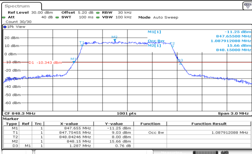
Band26-1.4MHz-16QAM-27033-6RB#0-1.088
