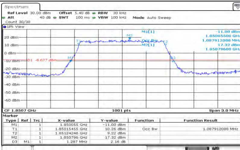
Band25-1.4MHz-QPSK-26047-6RB#0-1.088
