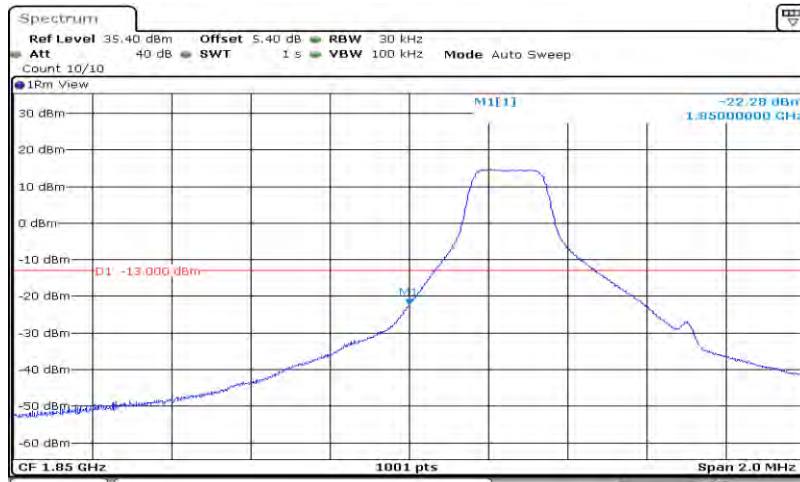
Band25-1.4MHz-16QAM-26047-6RB#0
