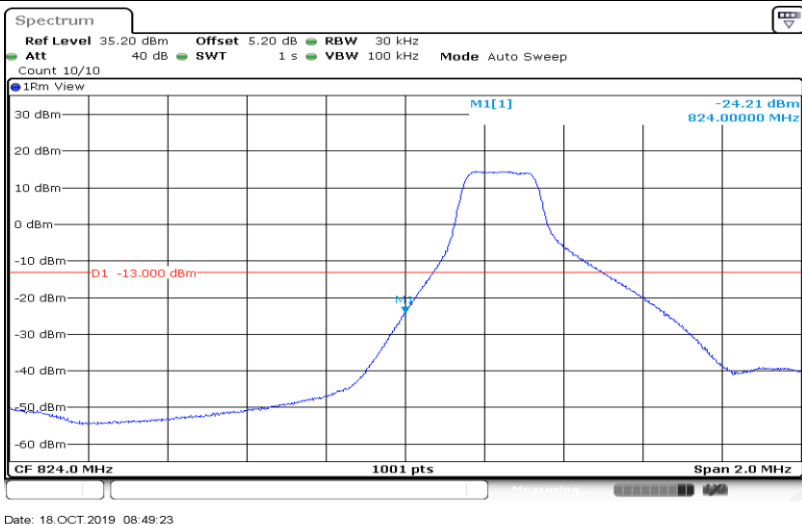
Band5-3MHz-16QAM-20415-15RB#0
