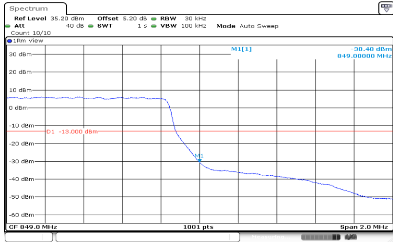
Band5-1.4MHz-16QAM-20643-6RB#0
