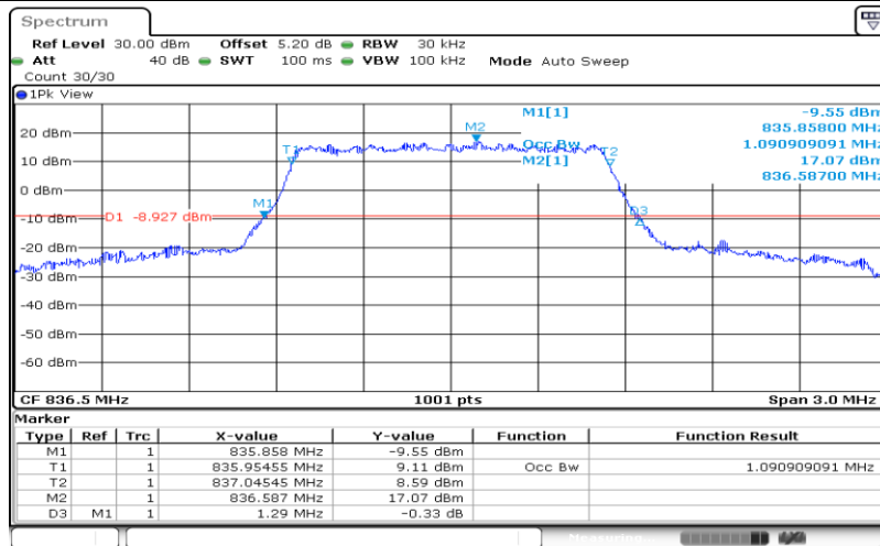
Band5-1.4MHz-QPSK-20525-6RB#0-1.091
