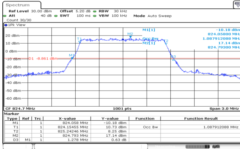
Band5-1.4MHz-QPSK-20407-6RB#0-1.088
