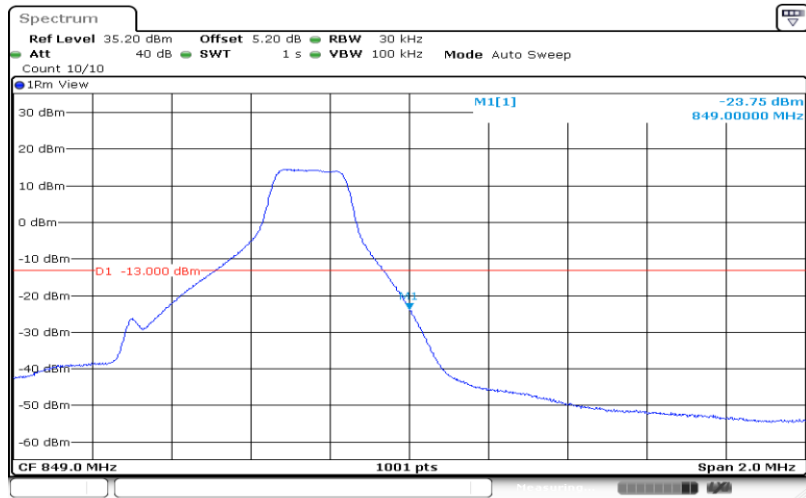
Band5-1.4MHz-16QAM-20643-6RB#0
