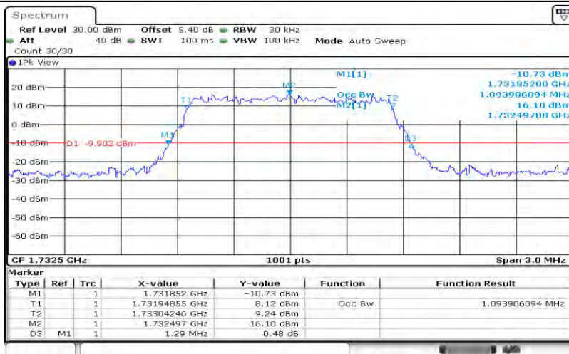
Band4-1.4MHz-QPSK-20175-6RB#0-1.094
