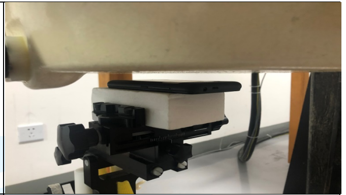
Rear Face of EUT with 1.0 cm Gap
