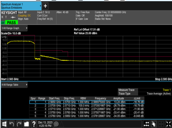
B7_5M_16QAM_25@0_CH_21425
