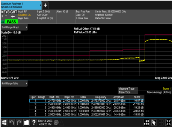
B7_5M_16QAM_25@0_CH_20775
