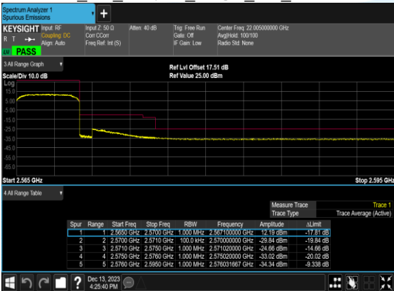
B7_5M_16QAM_25@0_CH_21425
