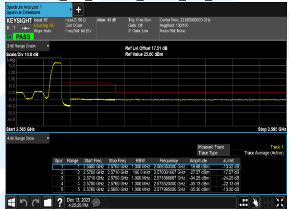
B7_5M_16QAM_1@24_CH_21425
