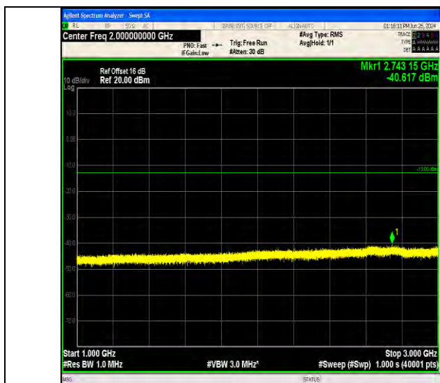
Band71_10MHz_64QAM_133297_50RB#0_1000~3000_1000~3000
