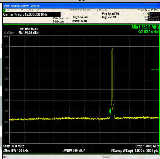
Band71_5MHz_QPSK_133447_25RB#0_30~1000_30~1000
