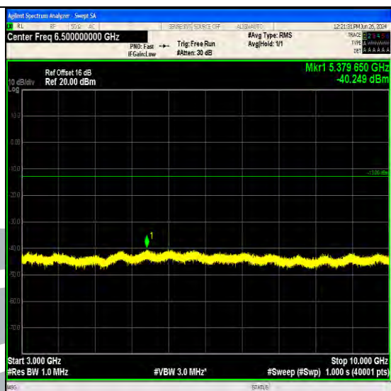
Band71_5MHz_64QAM_133447_25RB#0_3000~10000_3000~10000
