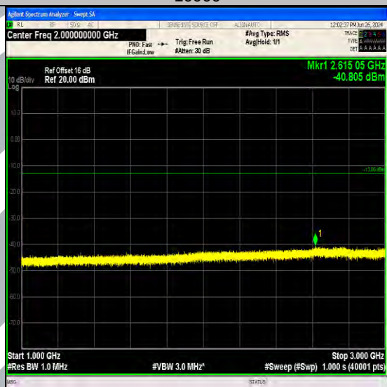
Band71_5MHz_16QAM_133147_1RB#0_1000~3000_1000~3000
