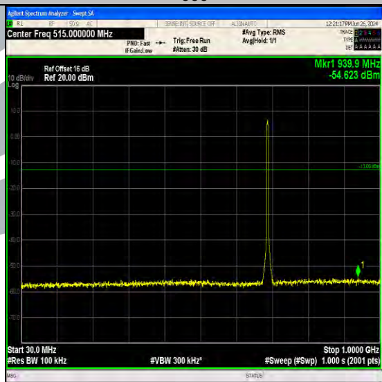
Band71_5MHz_64QAM_133447_25RB#0_30~1000_30~1000
