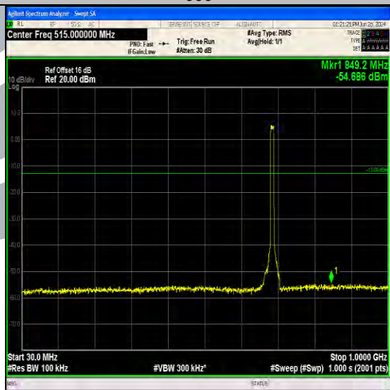
Band71_10MHz_QPSK_133422_50RB#0_30~1000_30~1000
