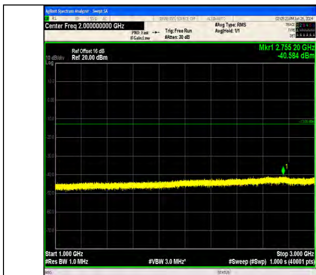
Band71_15MHz_QPSK_133197_1RB#74_1000~3000_1000~3000
