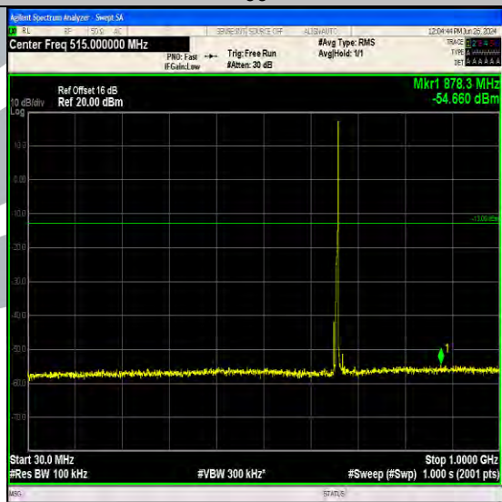
Band71_5MHz_16QAM_133147_1RB#24_30~1000_30~1000
