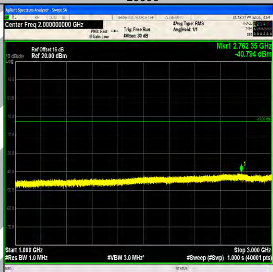
Band71_10MHz_64QAM_133422_1RB#0_1000~3000_1000~3000
