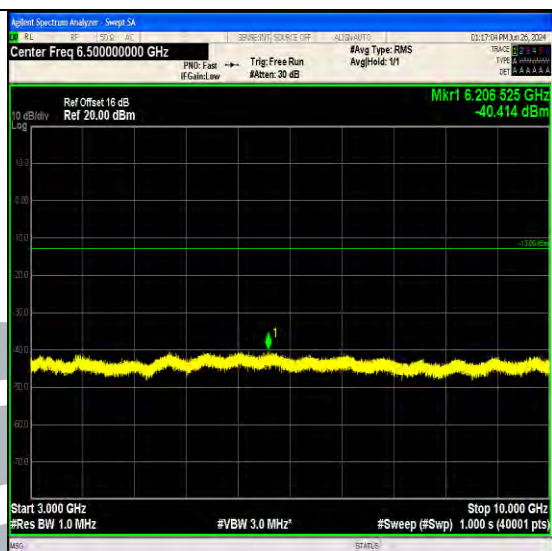
Band71_10MHz_QPSK_133422_1RB#0_3000~10000_3000~10000
