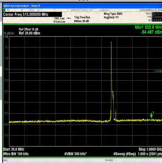
Band71_15MHz_QPSK_133297_1RB#0_30~1000_30~1000
