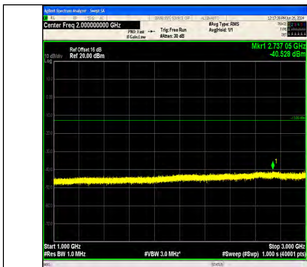
Band71_5MHz_QPSK_133447_1RB#24_1000~3000_1000~3000
