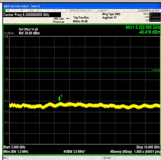
Band71_5MHz_QPSK_133447_25RB#0_3000~10000_3000~10000
