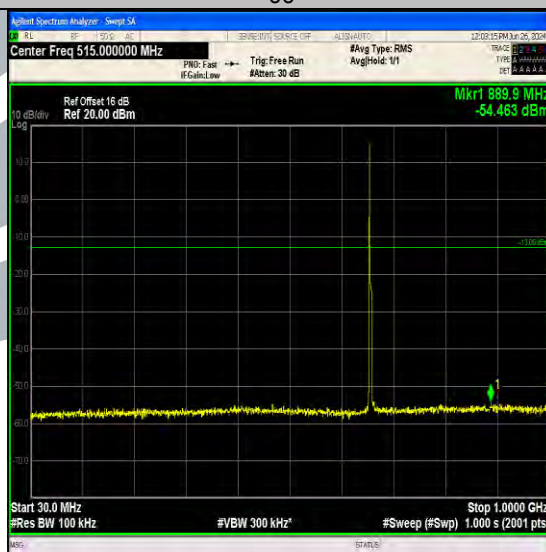
Band71_5MHz_64QAM_133147_1RB#0_30~1000_30~1000
