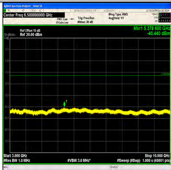
Band71_5MHz_64QAM_133447_1RB#24_3000~10000_3000~10000
