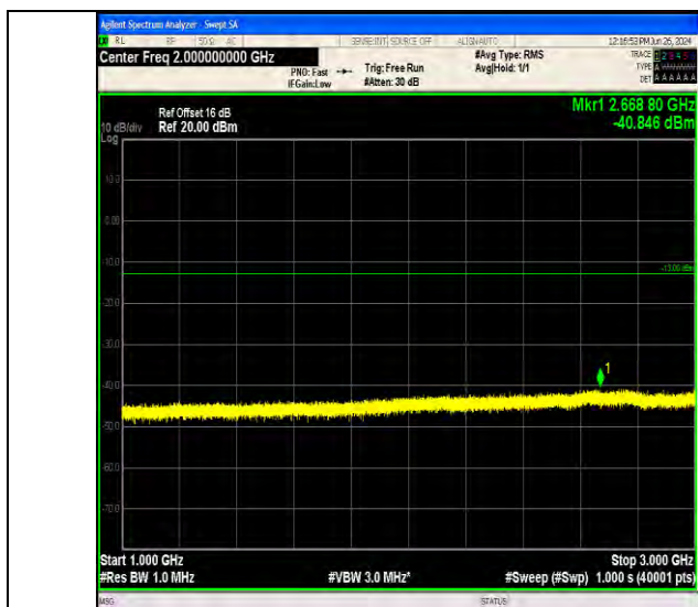
Band71_5MHz_64QAM_133447_1RB#0_1000~3000_1000~3000
