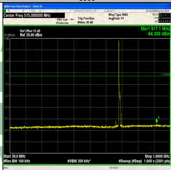
Band71_10MHz_64QAM_133422_1RB#0_30~1000_30~1000
