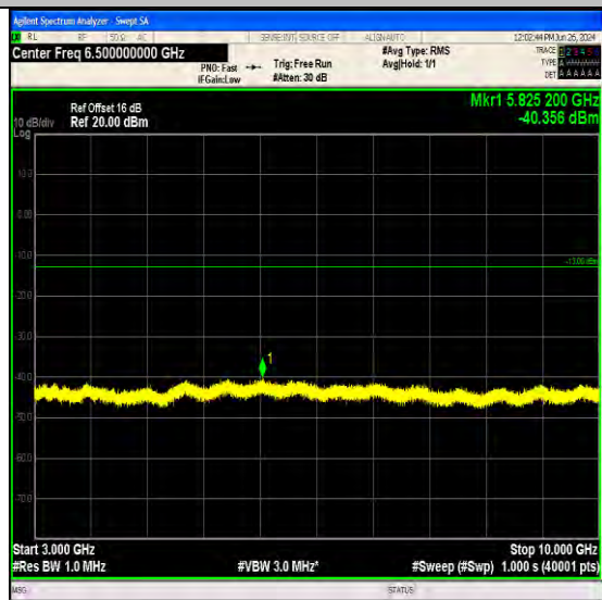
Band71_5MHz_16QAM_133147_1RB#0_3000~10000_3000~10000
