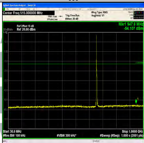
Band71_5MHz_16QAM_133147_1RB#0_30~1000_30~1000
