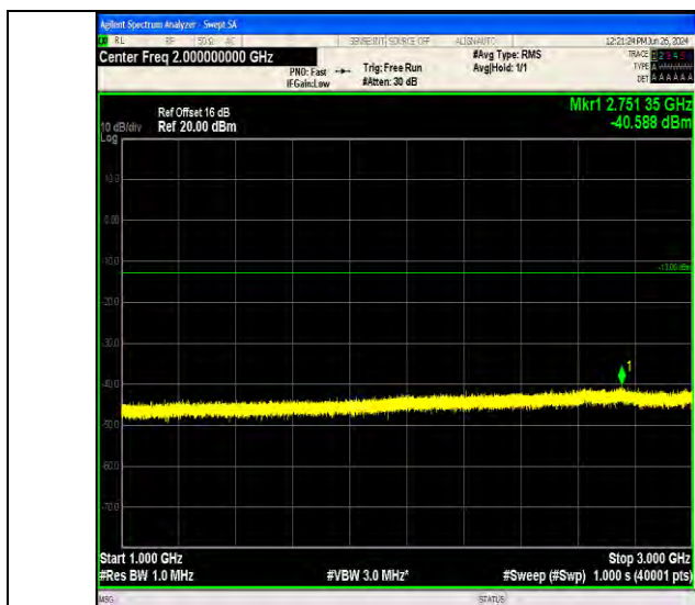
Band71_5MHz_64QAM_133447_25RB#0_1000~3000_1000~3000
