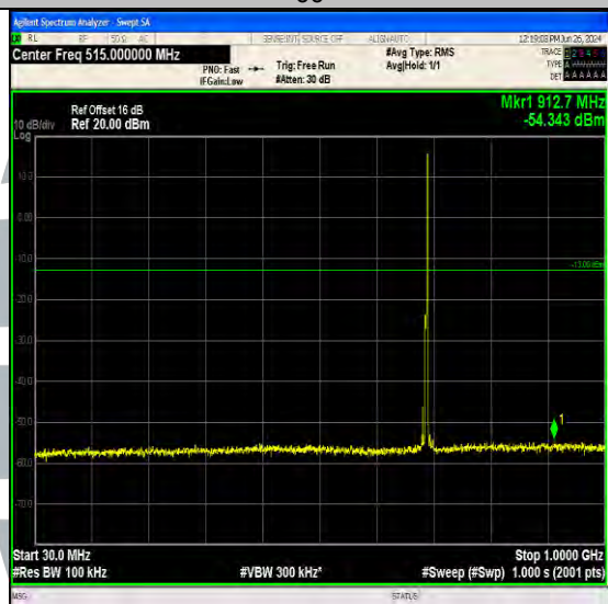
Band71_5MHz_64QAM_133447_1RB#24_30~1000_30~1000
