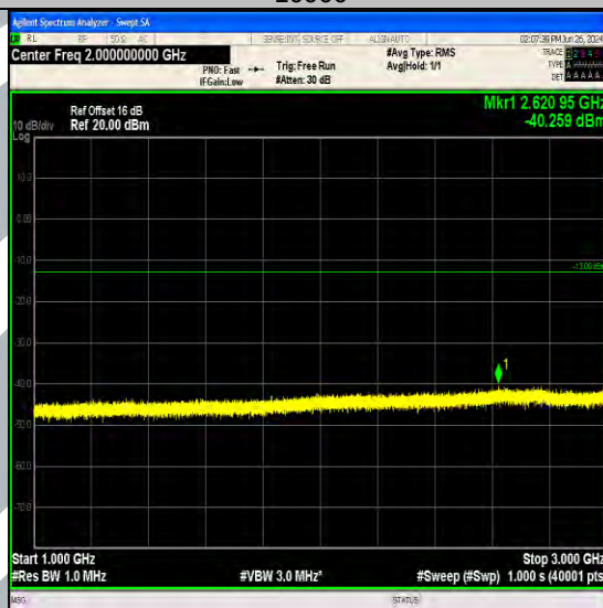
Band71_15MHz_QPSK_133197_75RB#0_1000~3000_1000~3000
