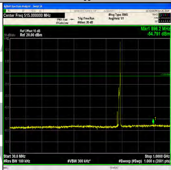
Band71_10MHz_QPSK_133422_1RB#49_30~1000_30~1000
