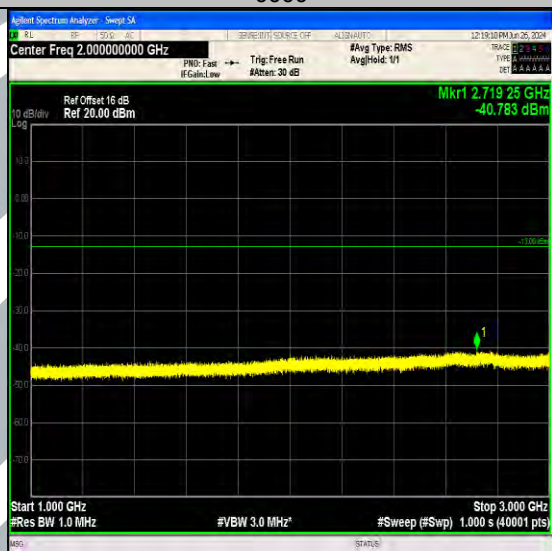
Band71_5MHz_64QAM_133447_1RB#24_1000~3000_1000~3000
