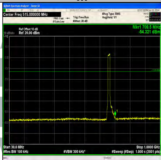
Band71_15MHz_QPSK_133197_75RB#0_30~1000_30~1000
