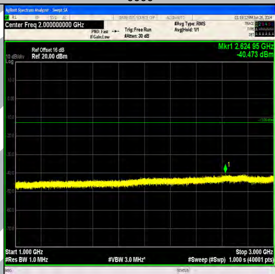
Band71_10MHz_QPSK_133422_1RB#49_1000~3000_1000~3000
