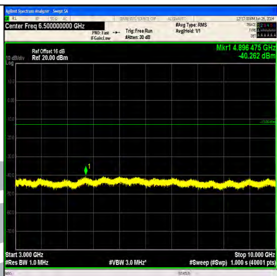
Band71_5MHz_64QAM_133447_1RB#0_3000~10000_3000~10000
