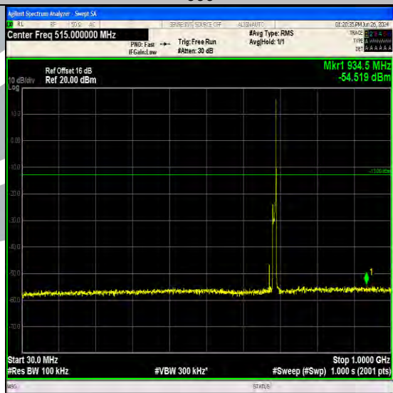
Band71_10MHz_64QAM_133422_1RB#49_30~1000_30~1000
