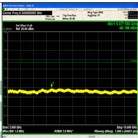
Band71_10MHz_64QAM_133297_50RB#0_3000~10000_3000~10000
