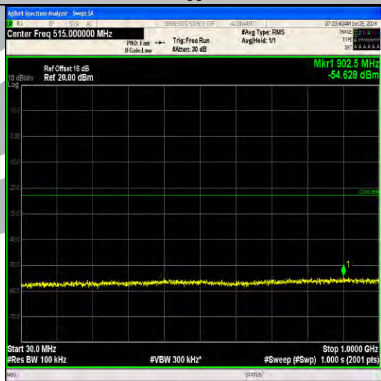
Band66_3MHz_16QAM_132322_1RB#14_30~1000_30~1000
