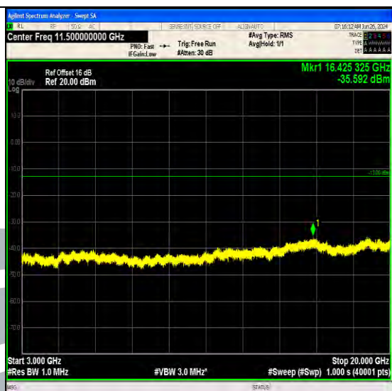
Band66_3MHz_16QAM_131987_1RB#0_3000~20000_3000~20000
