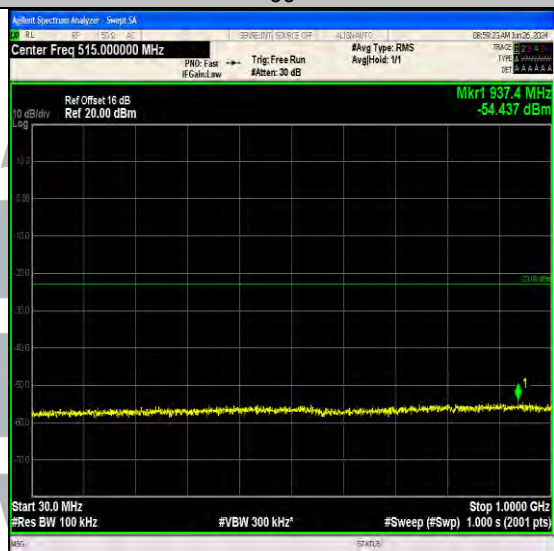
Band66_10MHz_QPSK_132022_1RB#49_30~1000_30~1000
