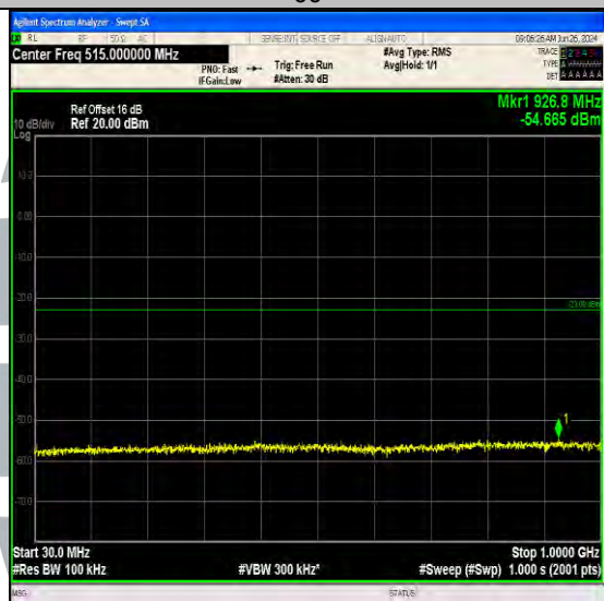
Band66_10MHz_QPSK_132622_1RB#49_30~1000_30~1000
