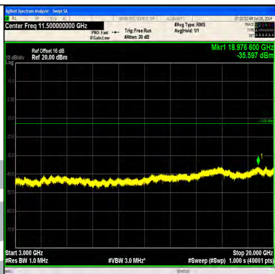
Band66_3MHz_16QAM_132322_1RB#14_3000~20000_3000~20000
