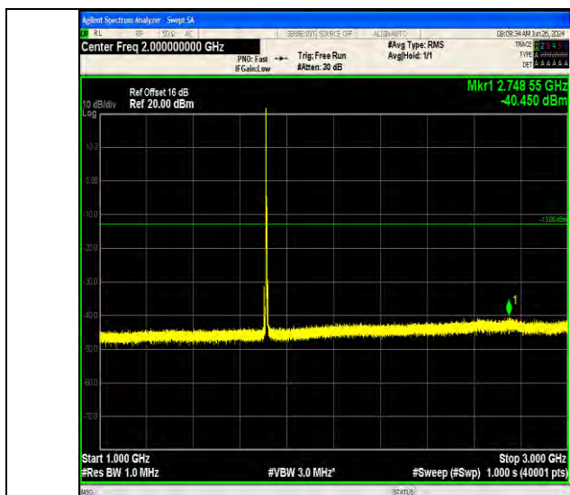
Band66_5MHz_64QAM_131997_1RB#0_1000~3000_1000~3000
