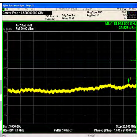
Band66_3MHz_16QAM_131987_15RB#0_3000~20000_3000~20000
