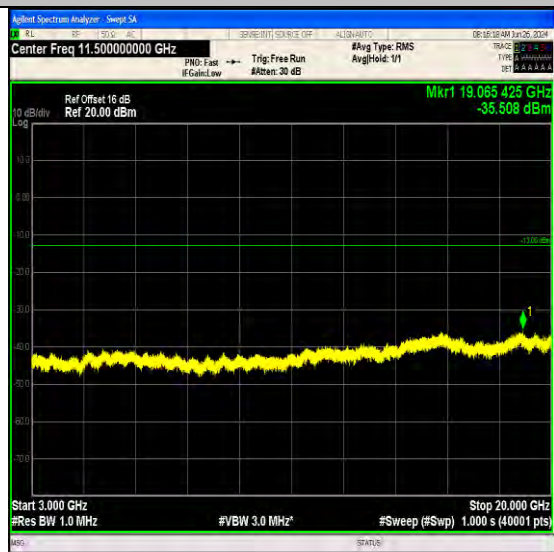
Band66_5MHz_16QAM_132647_1RB#0_3000~20000_3000~20000
