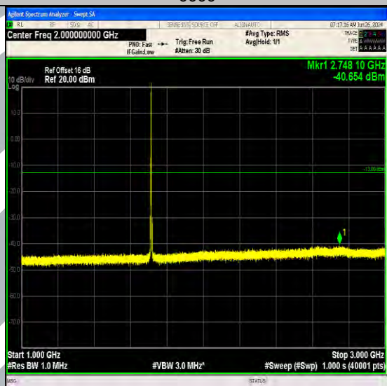
Band66_3MHz_16QAM_131987_1RB#14_1000~3000_1000~3000
