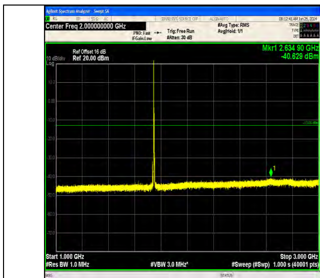
Band66_5MHz_16QAM_132322_1RB#0_1000~3000_1000~3000
