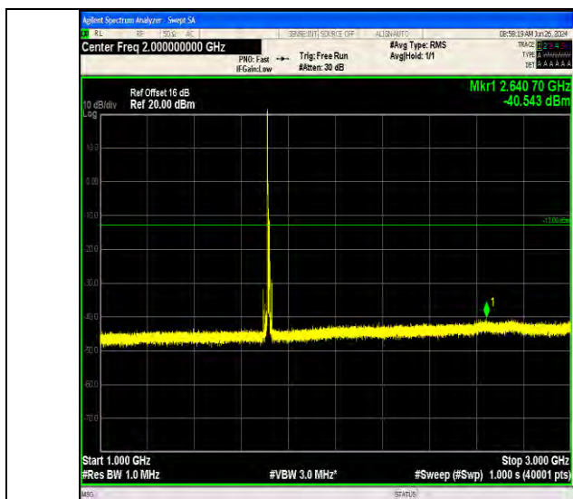
Band66_10MHz_QPSK_132022_1RB#0_1000~3000_1000~3000
