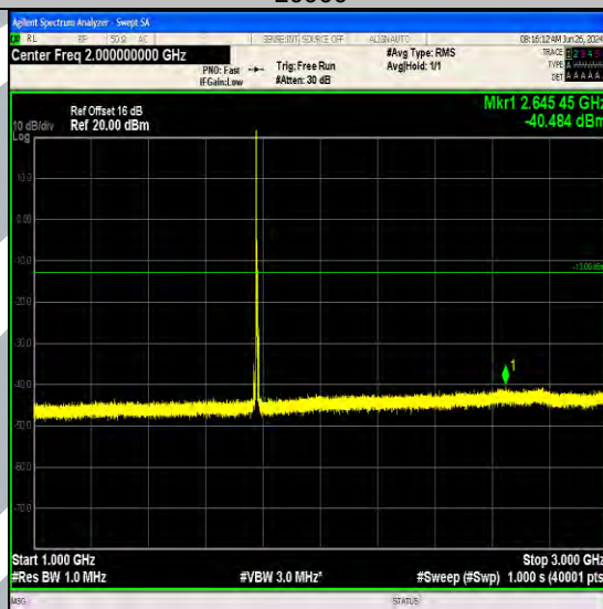
Band66_5MHz_16QAM_132647_1RB#0_1000~3000_1000~3000
