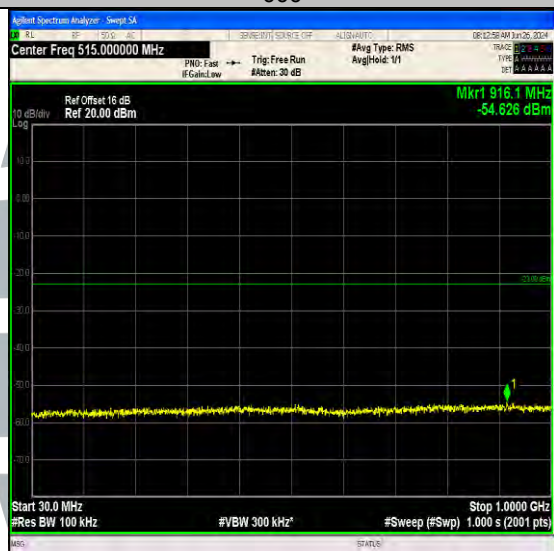
Band66_5MHz_64QAM_132322_1RB#0_30~1000_30~1000
