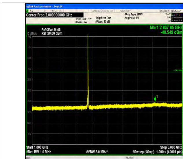
Band66_5MHz_QPSK_132322_1RB#0_1000~3000_1000~3000
