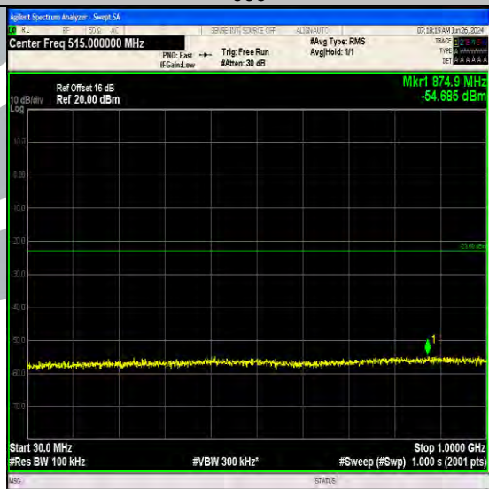
Band66_3MHz_16QAM_131987_15RB#0_30~1000_30~1000
