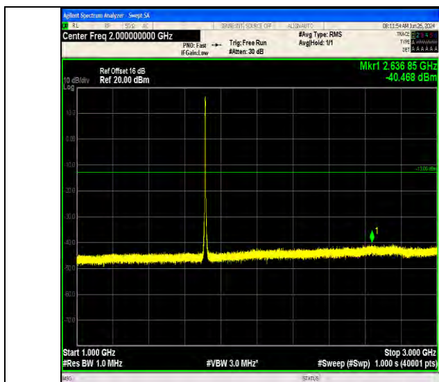
Band66_5MHz_64QAM_131997_25RB#0_1000~3000_1000~3000
