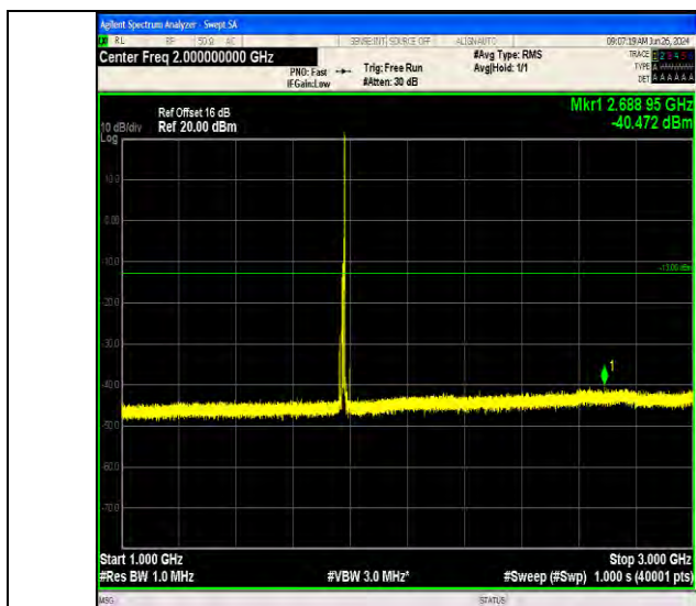
Band66_10MHz_64QAM_132622_1RB#49_1000~3000_1000~3000
