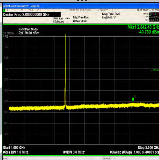
Band66_5MHz_QPSK_132322_1RB#24_1000~3000_1000~3000
