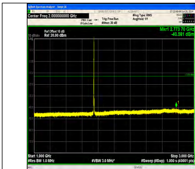
Band66_3MHz_16QAM_132322_1RB#14_1000~3000_1000~3000
