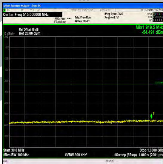
Band66_5MHz_64QAM_131997_25RB#0_30~1000_30~1000
