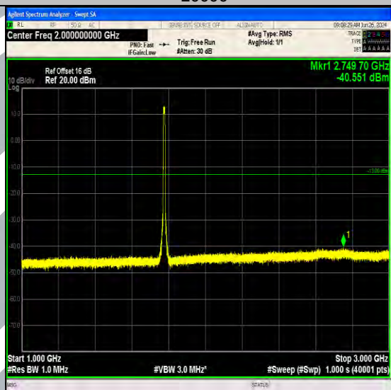
Band66_10MHz_64QAM_132622_50RB#0_1000~3000_1000~3000
