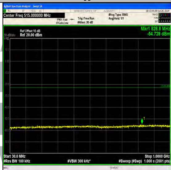
Band66_5MHz_16QAM_132322_1RB#24_30~1000_30~1000
