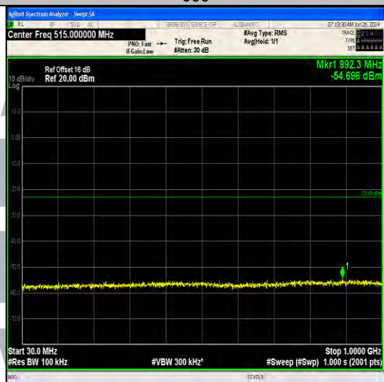
Band66_3MHz_16QAM_132322_1RB#0_30~1000_30~1000
