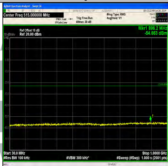
Band66_5MHz_QPSK_132322_1RB#24_30~1000_30~1000
