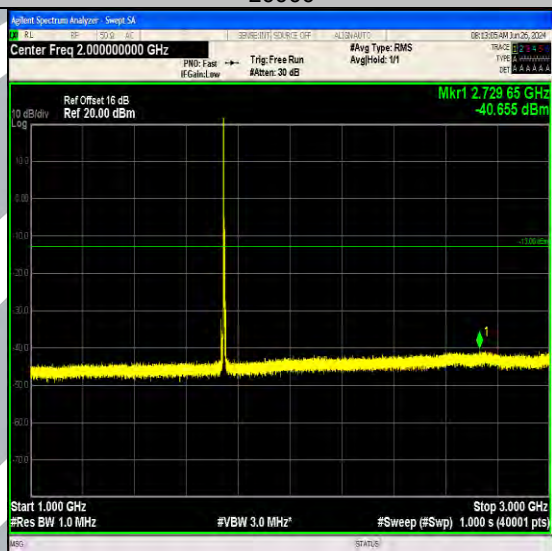
Band66_5MHz_64QAM_132322_1RB#0_1000~3000_1000~3000
