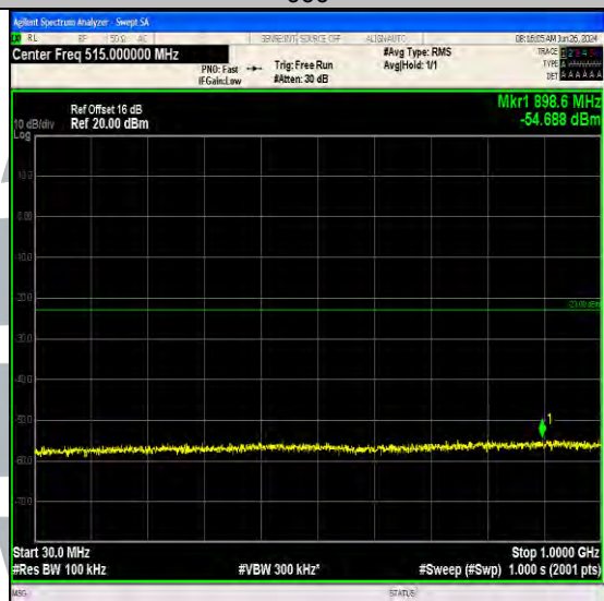
Band66_5MHz_16QAM_132647_1RB#0_30~1000_30~1000
