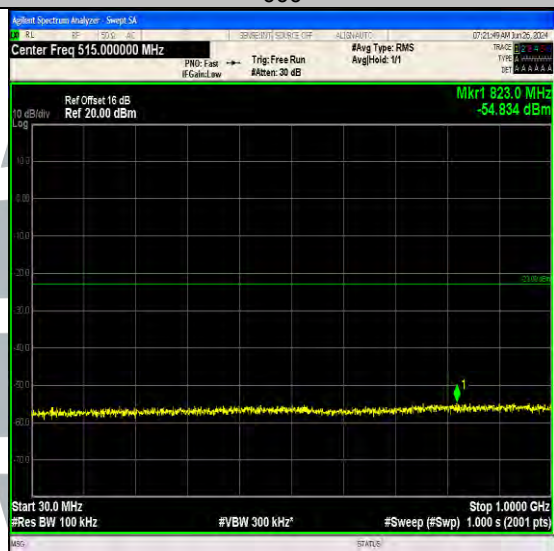
Band66_3MHz_16QAM_132322_15RB#0_30~1000_30~1000
