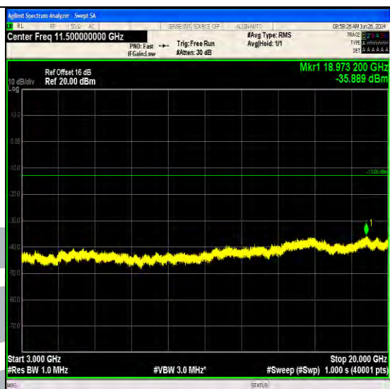
Band66_10MHz_QPSK_132022_1RB#0_3000~20000_3000~20000
