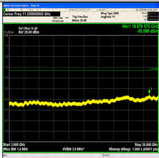
Band66_5MHz_16QAM_132322_1RB#24_3000~20000_3000~20000
