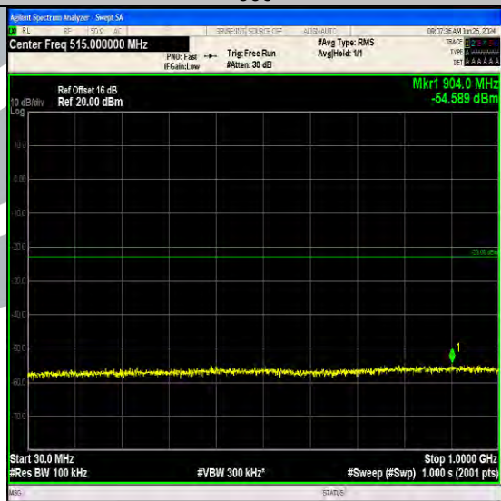
Band66_10MHz_QPSK_132622_50RB#0_30~1000_30~1000
