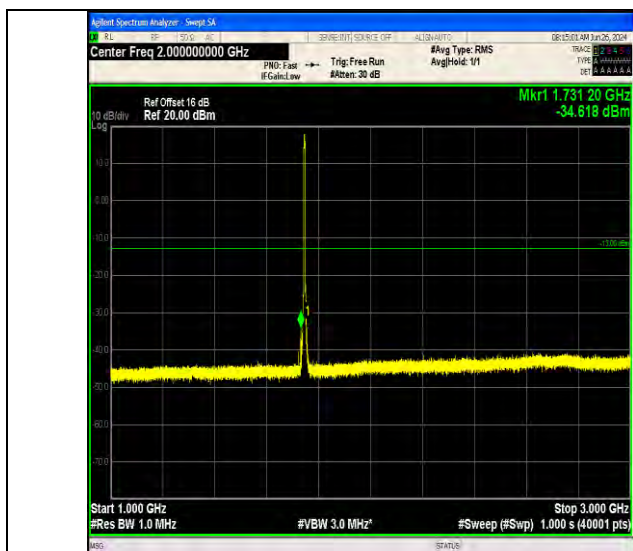
Band66_5MHz_16QAM_132322_25RB#0_1000~3000_1000~3000
