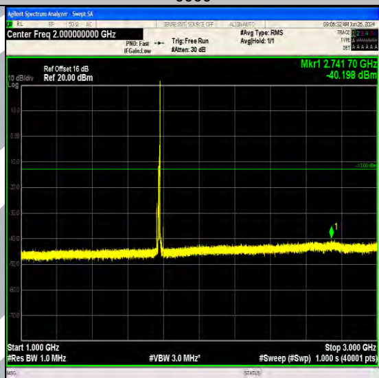
Band66_10MHz_QPSK_132622_1RB#49_1000~3000_1000~3000
