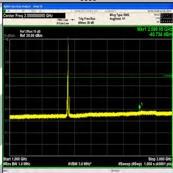
Band66_10MHz_QPSK_132022_1RB#49_1000~3000_1000~3000
