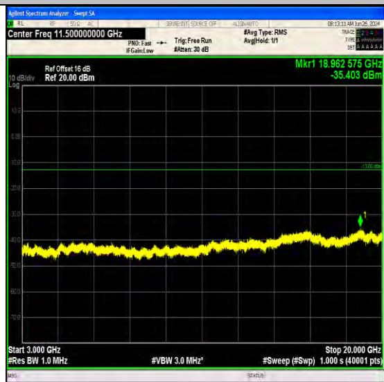
Band66_5MHz_64QAM_132322_1RB#0_3000~20000_3000~20000
