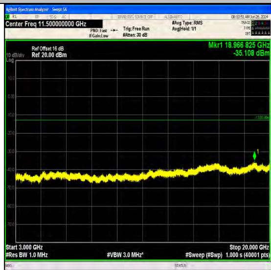
Band66_5MHz_64QAM_131997_1RB#24_3000~20000_3000~20000
