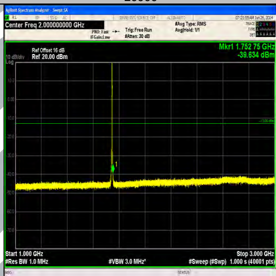
Band66_3MHz_16QAM_132322_15RB#0_1000~3000_1000~3000
