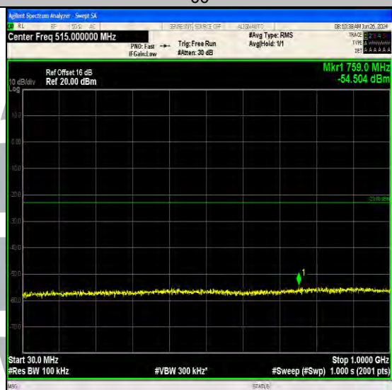
Band66_5MHz_64QAM_131997_1RB#24_30~1000_30~1000
