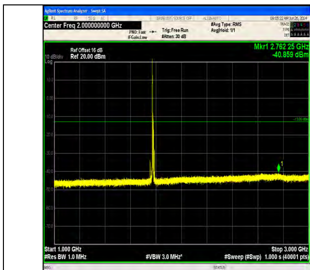
Band66_10MHz_QPSK_132622_1RB#0_1000~3000_1000~3000
