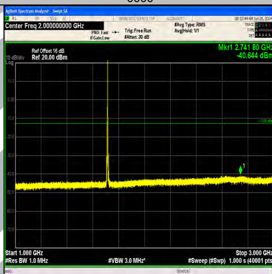
Band66_5MHz_64QAM_131997_1RB#24_1000~3000_1000~3000
