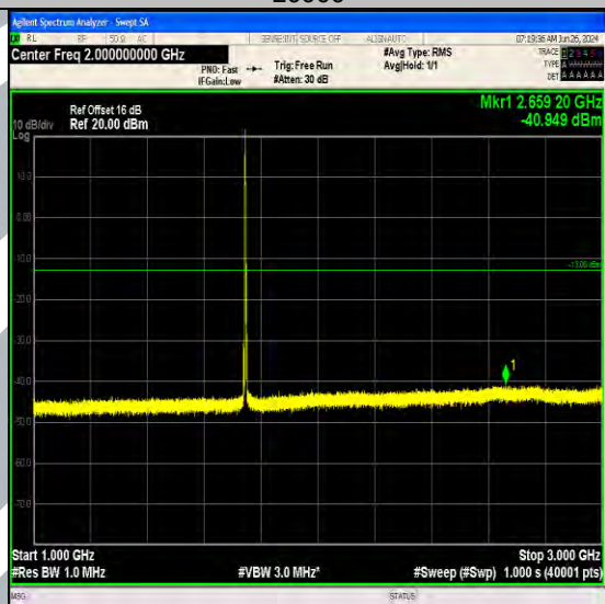
Band66_3MHz_16QAM_132322_1RB#0_1000~3000_1000~3000
