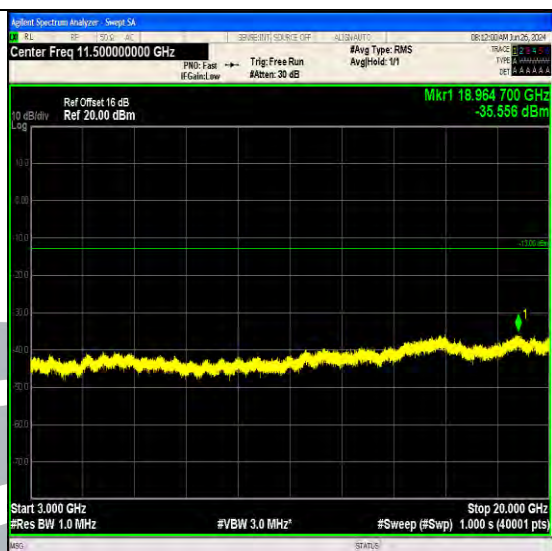
Band66_5MHz_64QAM_131997_25RB#0_3000~20000_3000~20000
