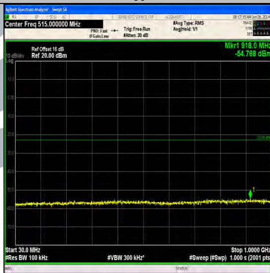
Band66_5MHz_16QAM_132647_1RB#24_30~1000_30~1000
