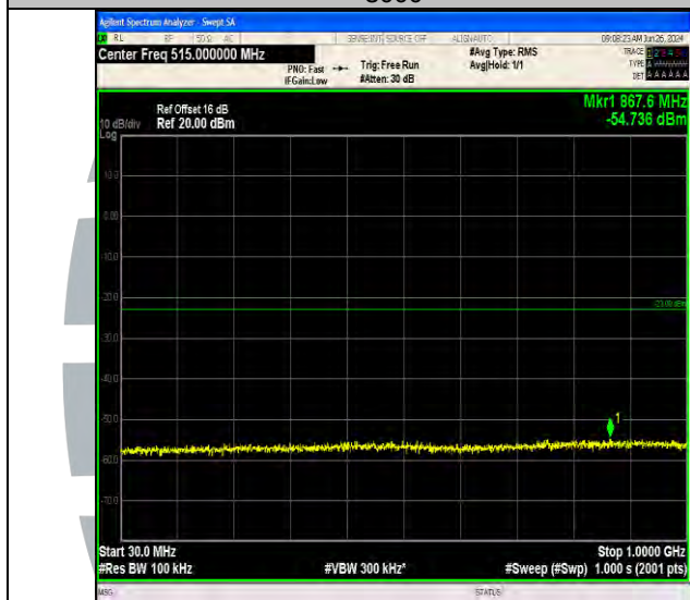
Band66_10MHz_64QAM_132622_50RB#0_30~1000_30~1000
