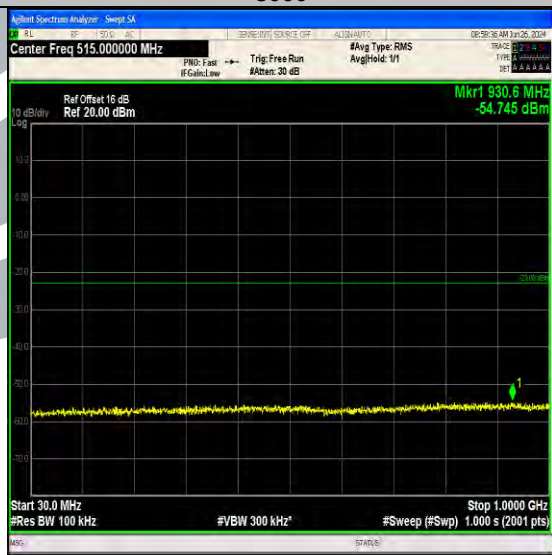
Band66_10MHz_16QAM_132022_1RB#0_30~1000_30~1000
