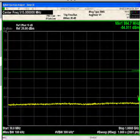
Band66_10MHz_QPSK_132022_50RB#0_30~1000_30~1000
