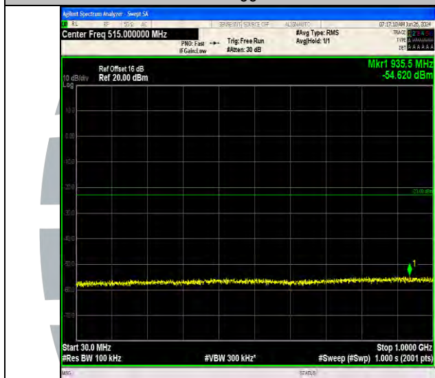
Band66_3MHz_16QAM_131987_1RB#14_30~1000_30~1000
