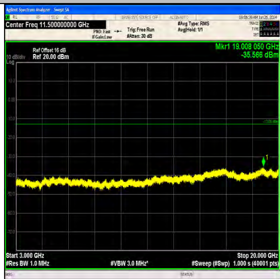
Band66_10MHz_QPSK_132622_1RB#49_3000~20000_3000~20000
