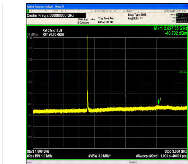
Band66_3MHz_16QAM_131987_1RB#0_1000~3000_1000~3000
