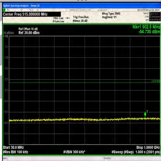
Band66_5MHz_16QAM_132322_25RB#0_30~1000_30~1000
