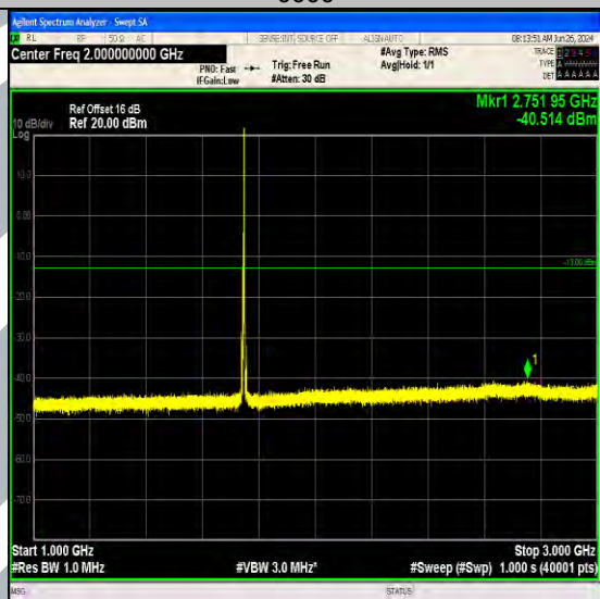
Band66_5MHz_16QAM_132322_1RB#24_1000~3000_1000~3000
