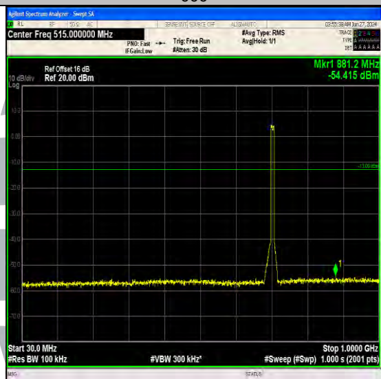
Band17_10MHz_16QAM_23790_50RB#0_30~1000_30~1000
