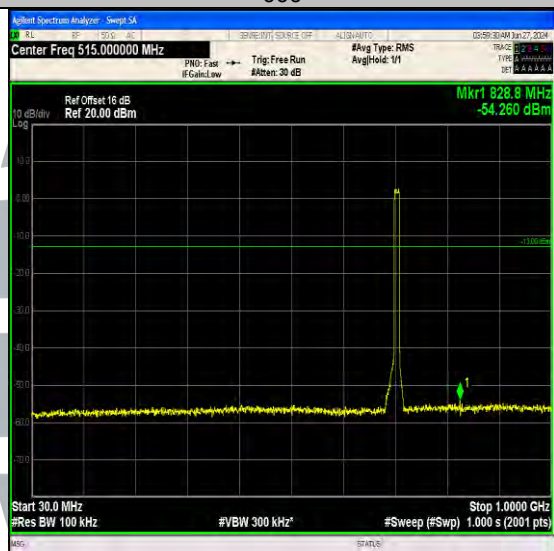
Band17_10MHz_64QAM_23800_50RB#0_30~1000_30~1000
