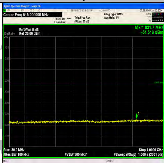
Band66_3MHz_QPSK_132657_1RB#14_30~1000_30~1000
