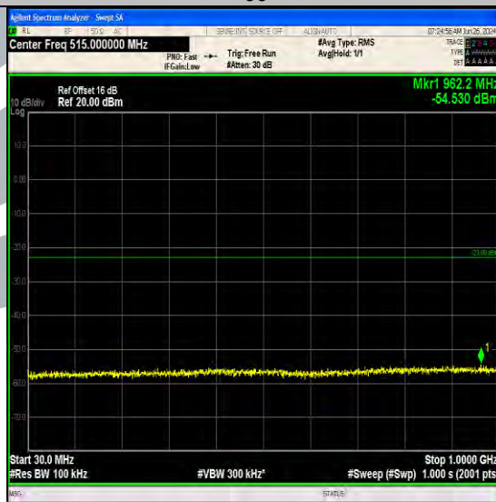
Band66_3MHz_QPSK_132657_15RB#0_30~1000_30~1000
