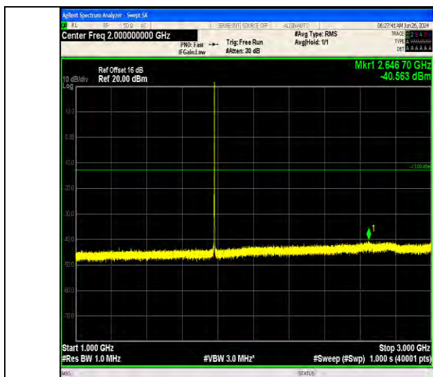
Band66_1.4MHz_16QAM_132665_1RB#5_1000~3000_1000~3000
