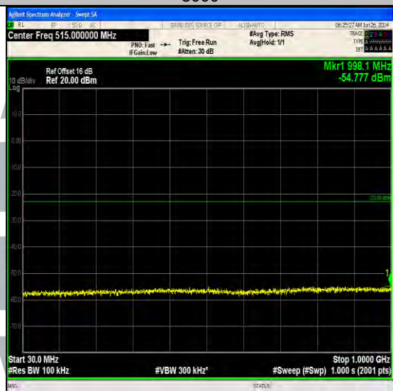
Band66_1.4MHz_64QAM_132322_6RB#0_30~1000_30~1000
