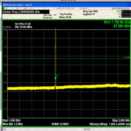
Band66_1.4MHz_16QAM_132665_6RB#0_1000~3000_1000~3000
