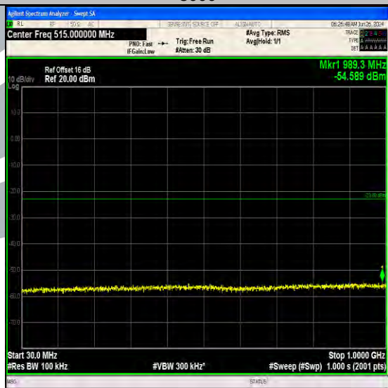
Band66_1.4MHz_64QAM_132665_1RB#0_30~1000_30~1000
