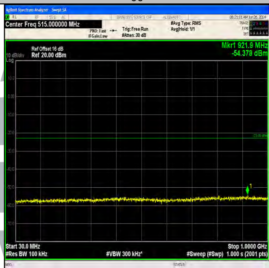
Band66_1.4MHz_QPSK_131979_6RB#0_30~1000_30~1000
