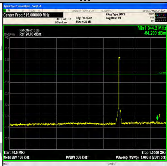
Band17_10MHz_64QAM_23780_50RB#0_30~1000_30~1000
