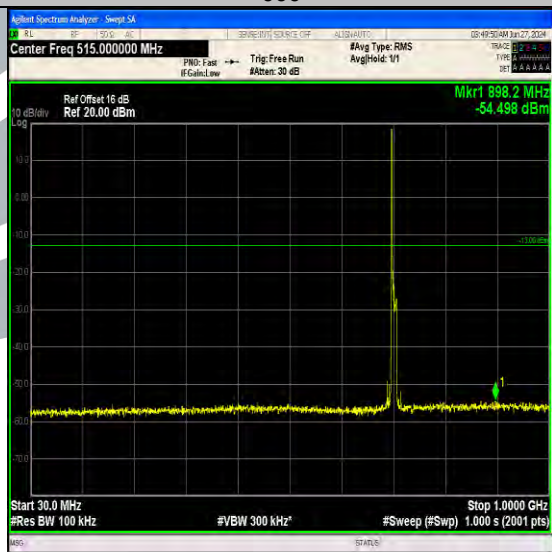
Band17_10MHz_16QAM_23780_1RB#0_30~1000_30~1000
