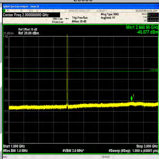
Band66_1.4MHz_64QAM_132665_1RB#5_1000~3000_1000~3000
