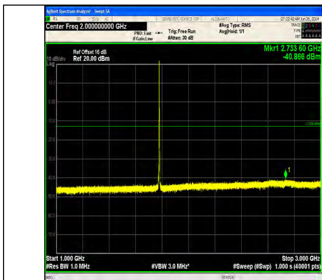
Band66_3MHz_QPSK_132657_1RB#0_1000~3000_1000~3000
