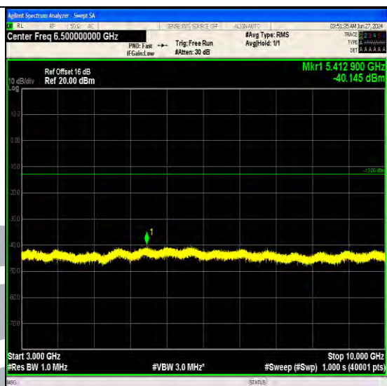
Band17_10MHz_64QAM_23780_1RB#49_3000~10000_3000~10000
