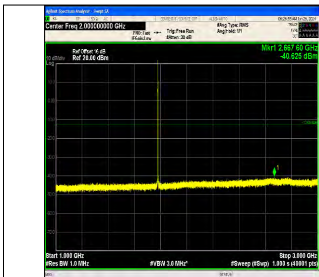
Band66_1.4MHz_64QAM_132665_1RB#0_1000~3000_1000~3000
