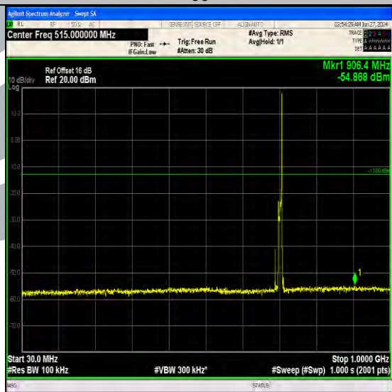
Band17_10MHz_16QAM_23790_1RB#49_30~1000_30~1000
