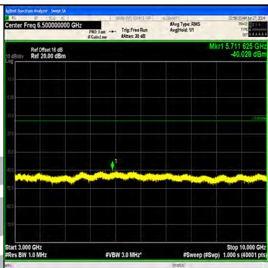
Band17_10MHz_64QAM_23800_1RB#49_3000~10000_3000~10000
