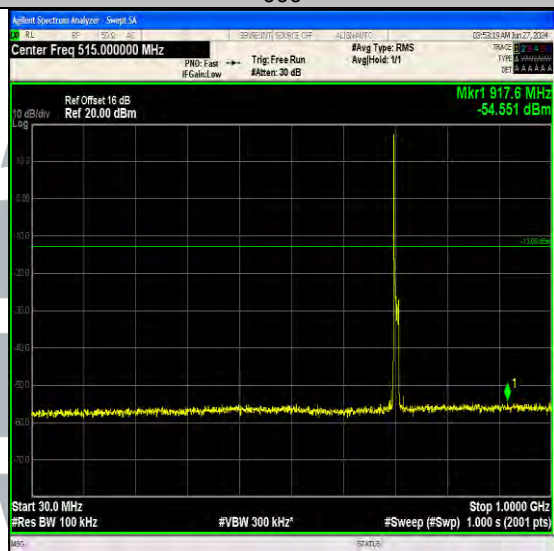
Band17_10MHz_16QAM_23790_1RB#0_30~1000_30~1000
