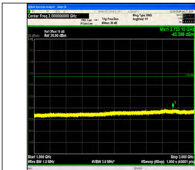
Band17_10MHz_16QAM_23790_1RB#49_1000~3000_1000~3000
