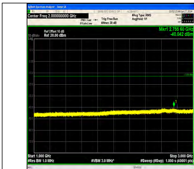
Band17_10MHz_16QAM_23780_50RB#0_1000~3000_1000~3000
