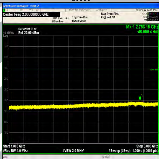
Band17_10MHz_64QAM_23800_50RB#0_1000~3000_1000~3000
