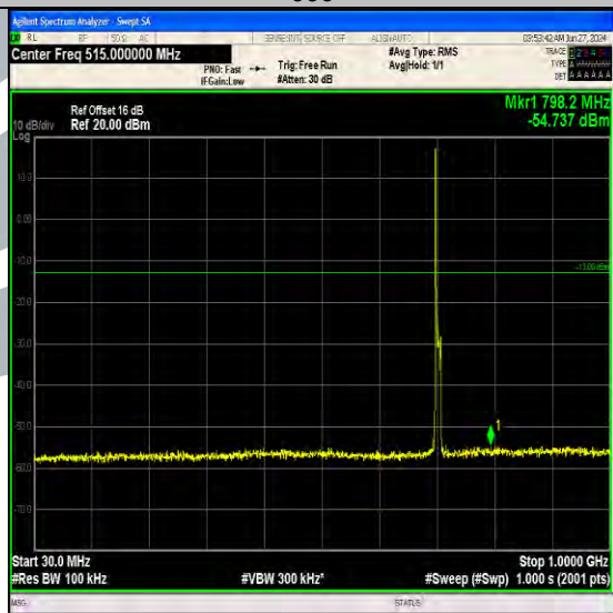
Band17_10MHz_64QAM_23790_1RB#0_30~1000_30~1000
