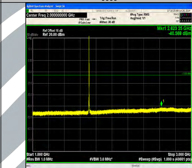
Band66_3MHz_64QAM_131987_1RB#0_1000~3000_1000~3000
