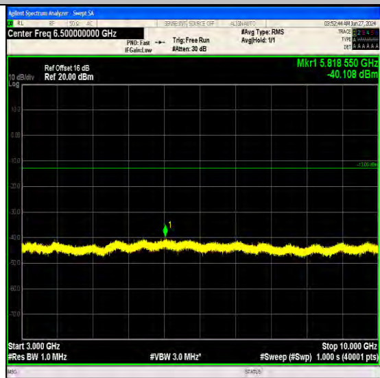
Band17_10MHz_64QAM_23780_50RB#0_3000~10000_3000~10000
