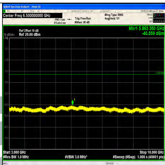
Band17_10MHz_16QAM_23780_50RB#0_3000~10000_3000~10000
