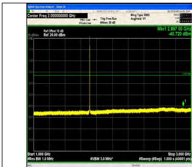
Band66_1.4MHz_QPSK_131979_1RB#5_1000~3000_1000~3000
