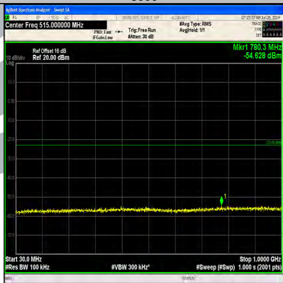
Band66_3MHz_QPSK_131987_1RB#0_30~1000_30~1000
