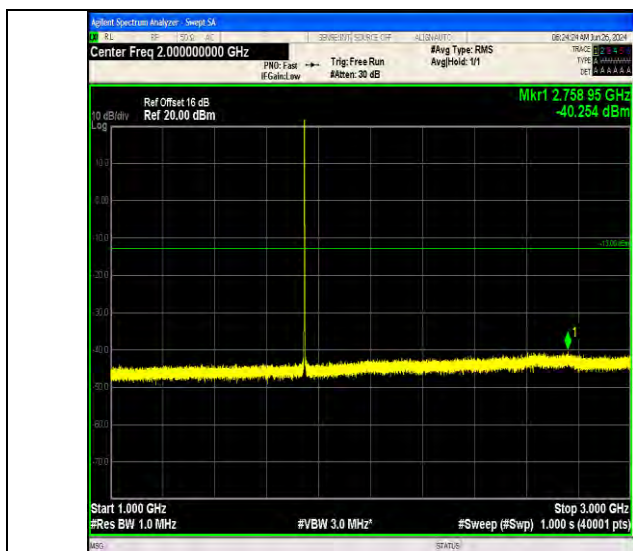
Band66_1.4MHz_64QAM_132322_1RB#5_1000~3000_1000~3000
