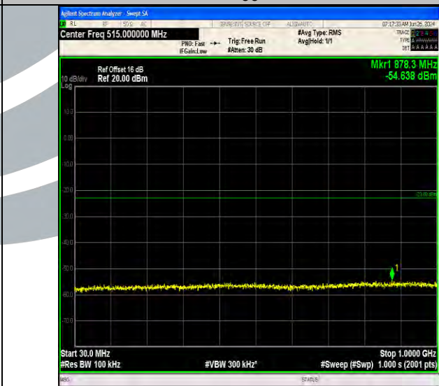
Band66_3MHz_64QAM_131987_1RB#14_30~1000_30~1000
