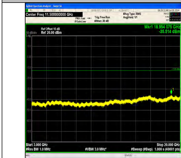
Band66_1.4MHz_64QAM_132665_1RB#5_3000~20000_3000~20000
