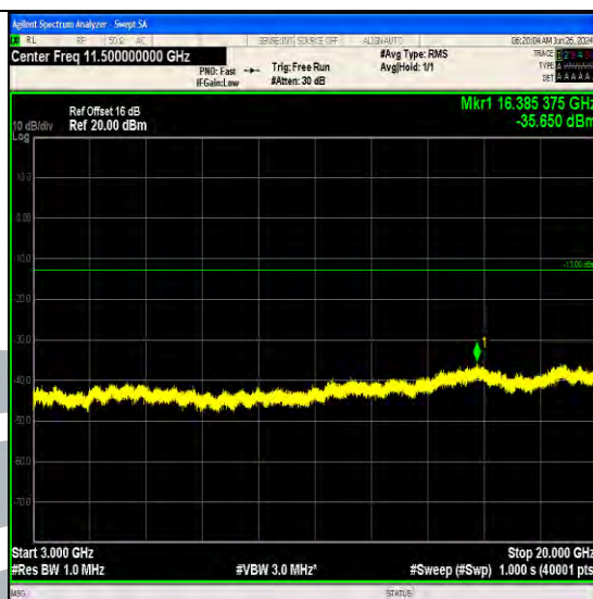
Band66_1.4MHz_QPSK_131979_1RB#5_3000~20000_3000~20000
