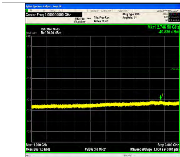
Band17_10MHz_64QAM_23780_1RB#49_1000~3000_1000~3000
