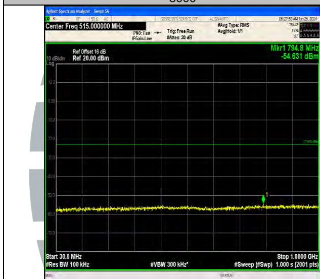
Band66_1.4MHz_64QAM_132665_1RB#5_30~1000_30~1000
