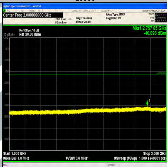
Band17_10MHz_16QAM_23790_50RB#0_1000~3000_1000~3000
