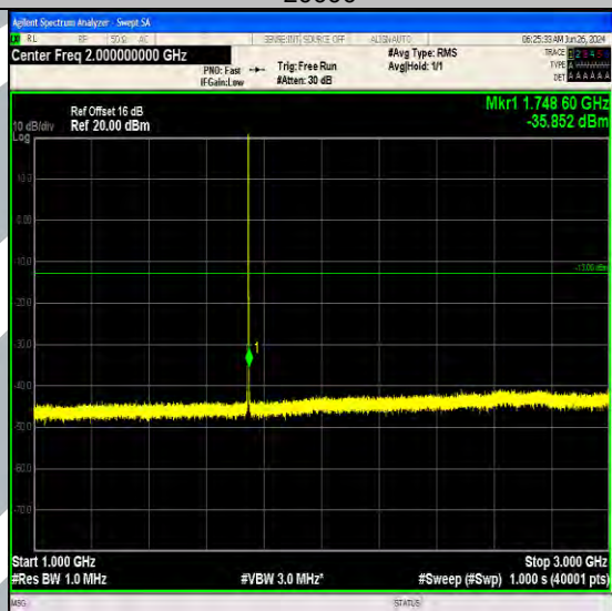
Band66_1.4MHz_64QAM_132322_6RB#0_1000~3000_1000~3000
