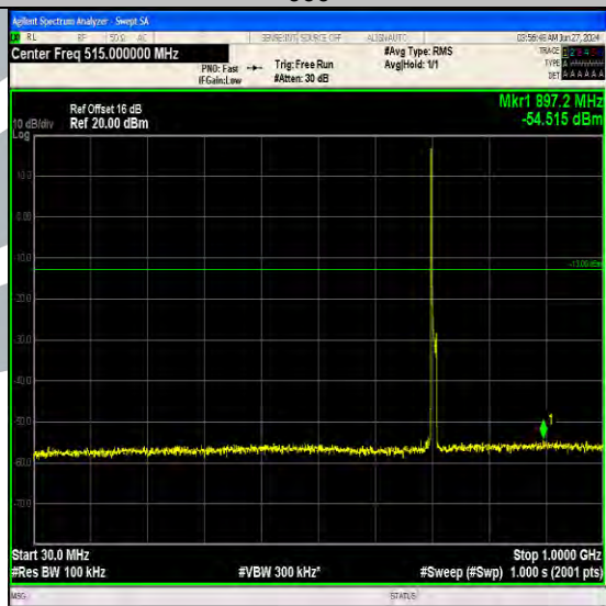
Band17_10MHz_16QAM_23800_1RB#0_30~1000_30~1000
