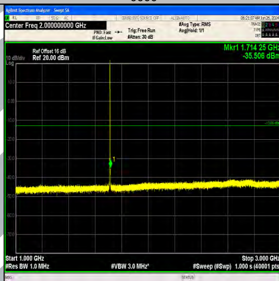
Band66_1.4MHz_QPSK_131979_6RB#0_1000~3000_1000~3000
