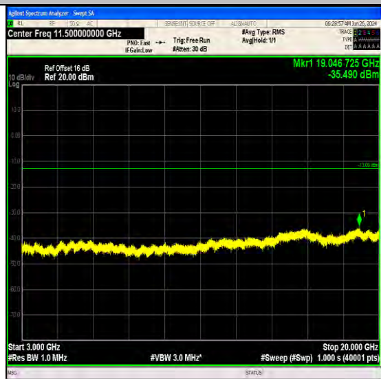
Band66_1.4MHz_16QAM_132665_6RB#0_3000~20000_3000~20000
