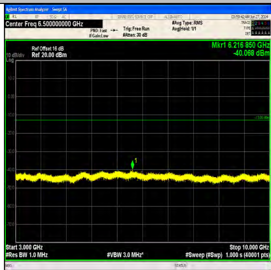
Band17_10MHz_64QAM_23800_50RB#0_3000~10000_3000~10000
