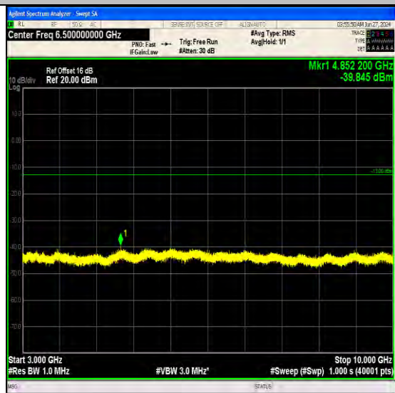
Band17_10MHz_16QAM_23790_50RB#0_3000~10000_3000~10000
