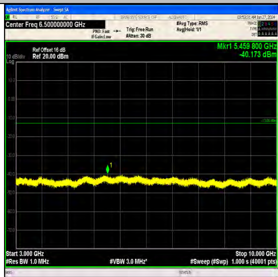
Band17_10MHz_16QAM_23790_1RB#0_3000~10000_3000~10000
