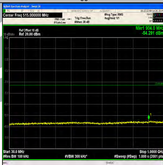
Band66_1.4MHz_QPSK_132322_1RB#0_30~1000_30~1000
