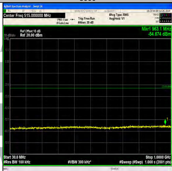
Band66_1.4MHz_16QAM_132665_6RB#0_30~1000_30~1000
