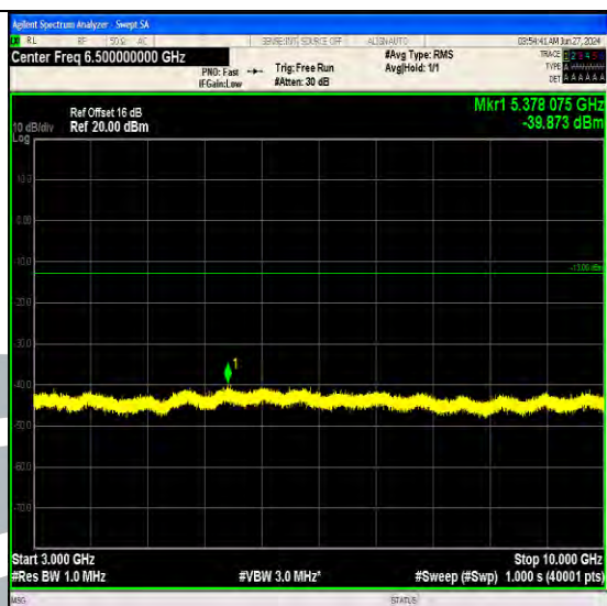
Band17_10MHz_16QAM_23790_1RB#49_3000~10000_3000~10000
