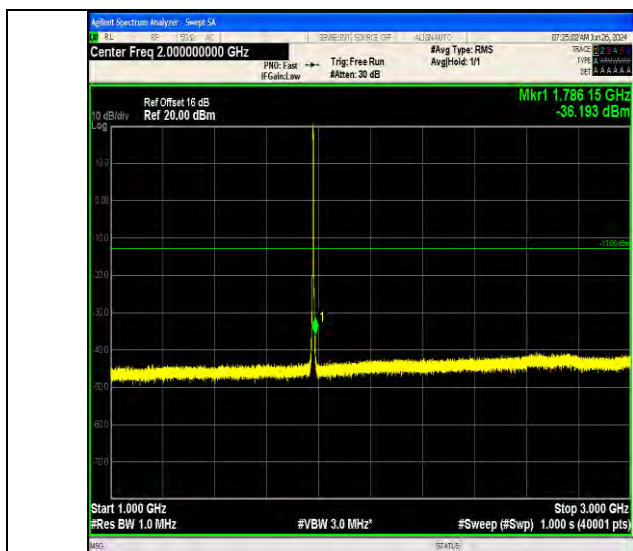
Band66_3MHz_QPSK_132657_15RB#0_1000~3000_1000~3000
