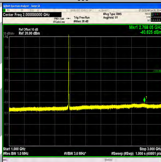
Band66_3MHz_QPSK_132657_1RB#14_1000~3000_1000~3000
