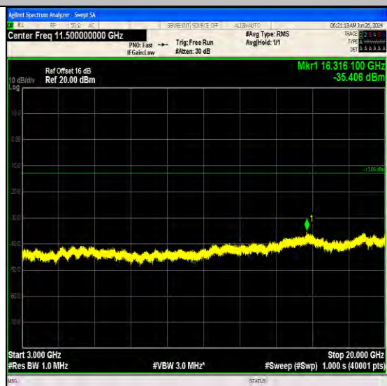
Band66_1.4MHz_QPSK_131979_6RB#0_3000~20000_3000~20000
