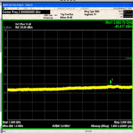
Band17_10MHz_64QAM_23780_50RB#0_1000~3000_1000~3000
