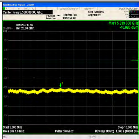
Band17_5MHz_64QAM_23825_1RB#24_3000~10000_3000~10000
