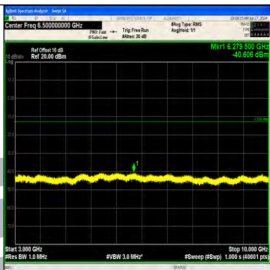
Band17_5MHz_64QAM_23825_1RB#0_3000~10000_3000~10000
