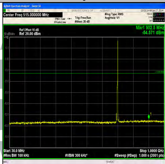
Band17_5MHz_64QAM_23755_1RB#24_30~1000_30~1000
