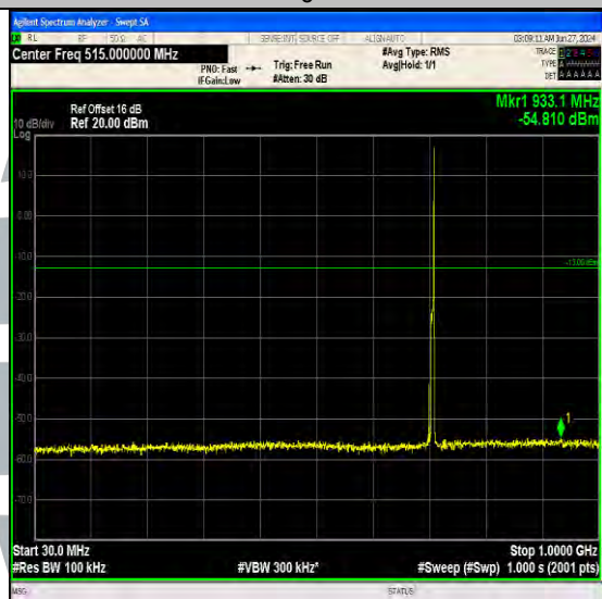
Band17_5MHz_64QAM_23825_1RB#24_30~1000_30~1000
