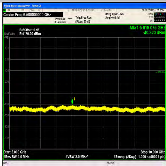
Band17_5MHz_64QAM_23755_1RB#24_3000~10000_3000~10000 0000
