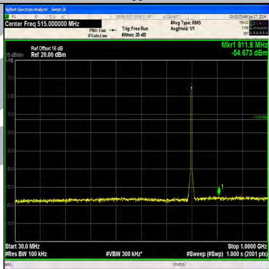
Band17_5MHz_64QAM_23755_25RB#0_30~1000_30~1000
