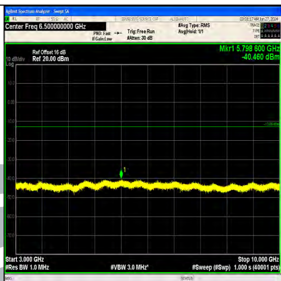
Band17_5MHz_64QAM_23755_1RB#0_3000~10000_3000~10000 000
