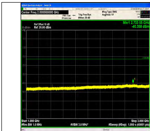
Band17_5MHz_64QAM_23825_1RB#0_1000~3000_1000~3000
