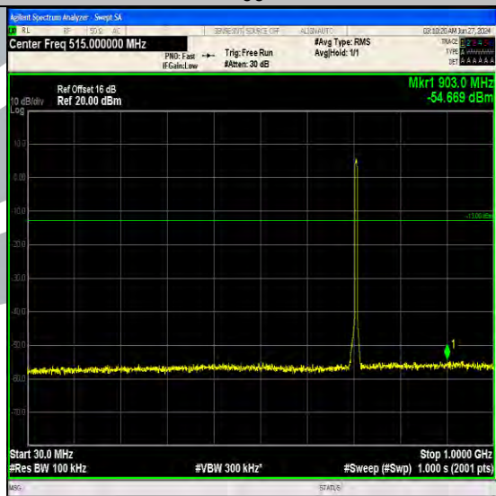
Band17_5MHz_64QAM_23825_25RB#0_30~1000_30~1000
