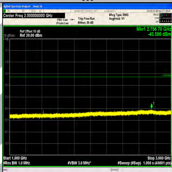
Band17_5MHz_64QAM_23755_1RB#24_1000~3000_1000~3000 00
