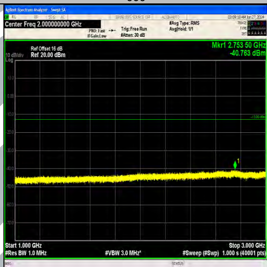
Band17_5MHz_64QAM_23825_1RB#24_1000~3000_1000~3000
