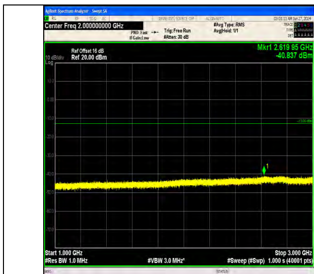
Band17_5MHz_64QAM_23755_1RB#0_1000~3000_1000~3000 0
