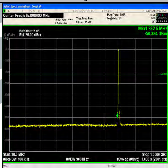
Band12_3MHz_QPSK_23025_15RB#0_30~1000_30~1000
