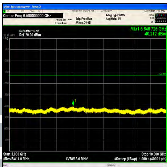
Band12_3MHz_QPSK_23025_1RB#0_3000~10000_3000~10000
