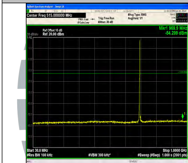
Band12_3MHz_QPSK_23025_1RB#14_30~1000_30~1000
