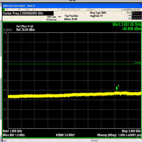
Band12_3MHz_QPSK_23025_1RB#14_1000~3000_1000~3000
