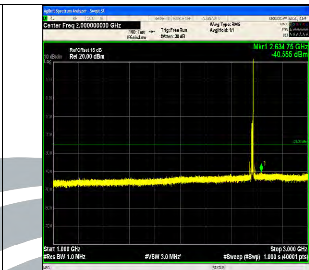
Band7_15MHz_QPSK_21375_1RB#74_1000~3000_1000~3000
