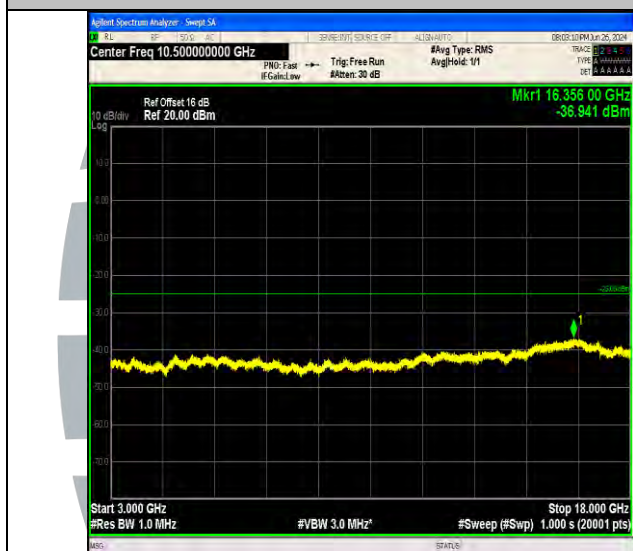
Band7_15MHz_QPSK_21375_1RB#74_3000~18000_3000~18000
