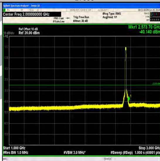
Band7_15MHz_64QAM_21100_75RB#0_1000~3000_1000~3000
