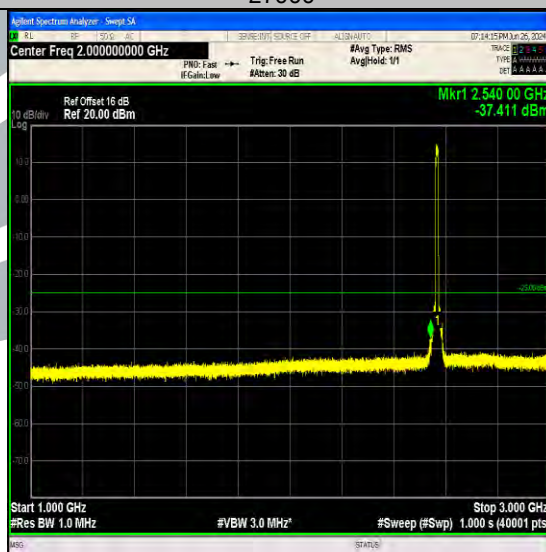
Band7_10MHz_QPSK_21400_50RB#0_1000~3000_1000~3000
