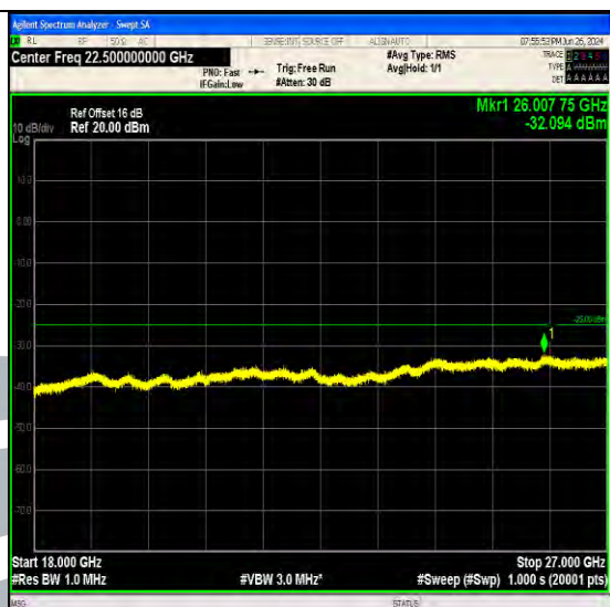
Band7_15MHz_QPSK_20825_75RB#0_18000~27000_18000~27000
