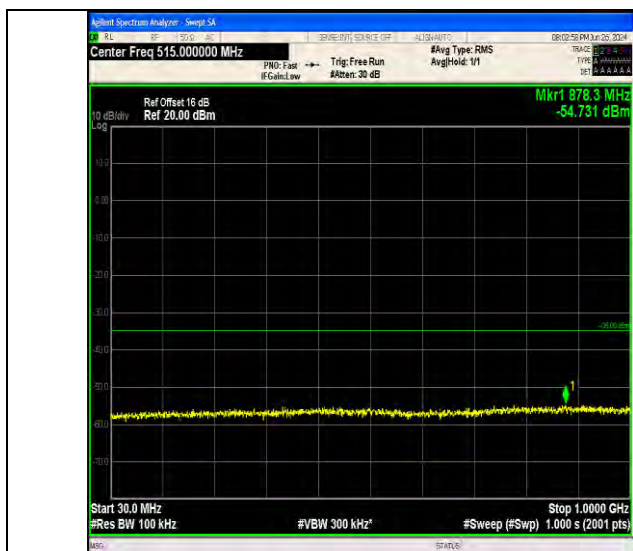
Band7_15MHz_QPSK_21375_1RB#74_30~1000_30~1000
