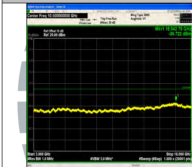
Band7_10MHz_QPSK_21400_1RB#49_3000~18000_3000~18000
