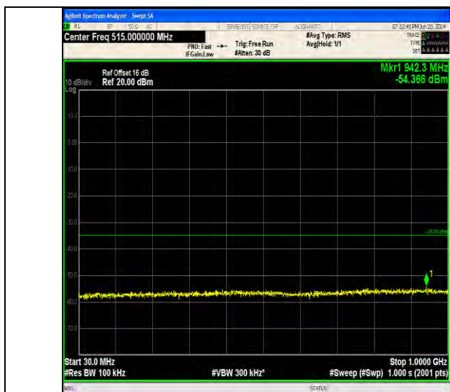
Band7_10MHz_QPSK_21400_1RB#49_30~1000_30~1000
