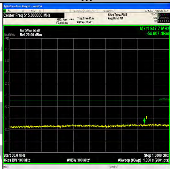
Band7_15MHz_64QAM_20825_1RB#0_30~1000_30~1000
