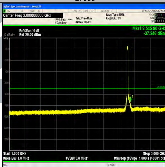
Band7_15MHz_QPSK_20825_75RB#0_1000~3000_1000~3000
