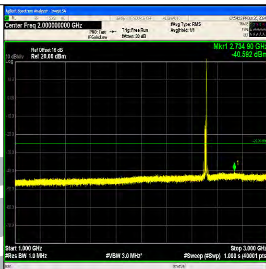
Band7_15MHz_QPSK_20825_1RB#74_1000~3000_1000~3000
