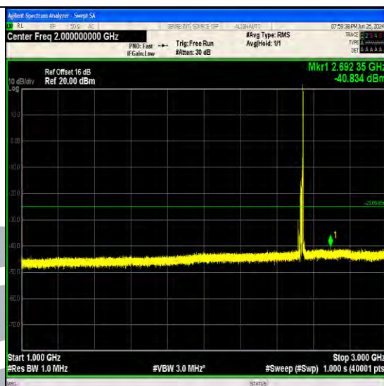
Band7_15MHz_64QAM_21100_1RB#74_1000~3000_1000~3000
