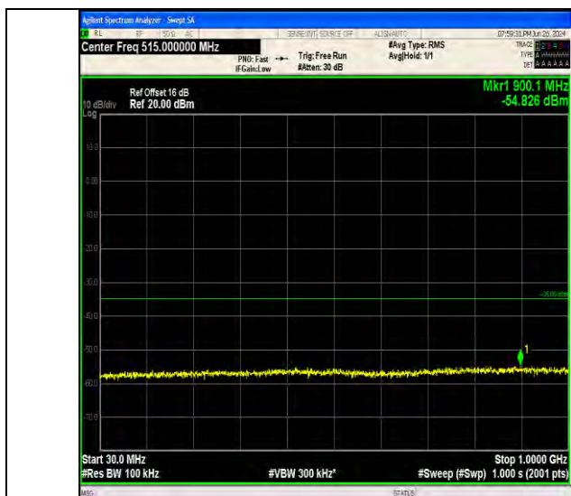
Band7_15MHz_64QAM_21100_1RB#74_30~1000_30~1000
