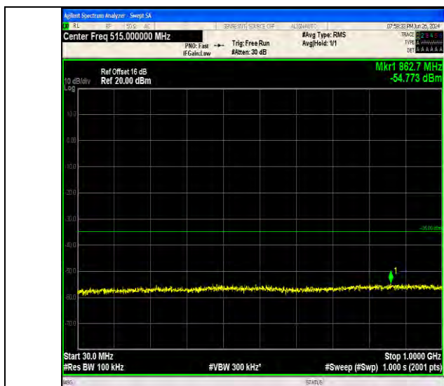
Band7_15MHz_QPSK_21100_1RB#74_30~1000_30~1000
