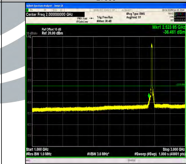
Band7_15MHz_QPSK_21375_75RB#0_1000~3000_1000~3000
