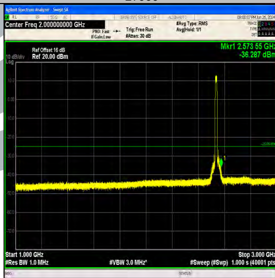
Band7_15MHz_QPSK_21100_75RB#0_1000~3000_1000~3000
