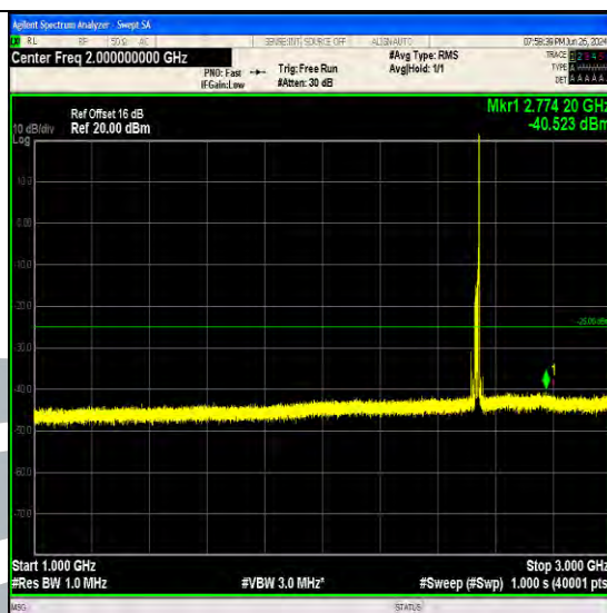
Band7_15MHz_QPSK_21100_1RB#74_1000~3000_1000~3000
