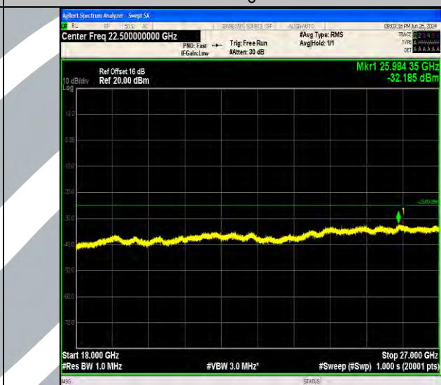
Band7_15MHz_QPSK_21375_1RB#74_18000~27000_18000~27000
