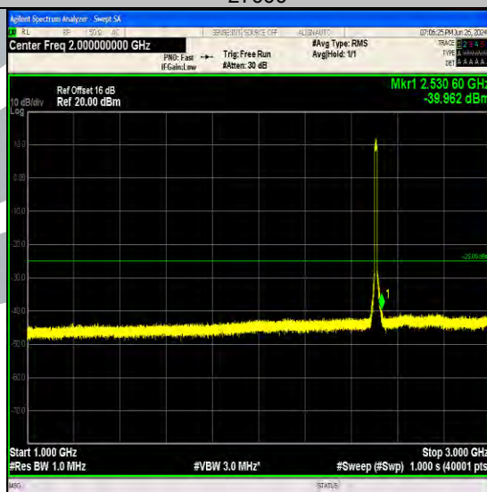
Band7_10MHz_64QAM_20800_50RB#0_1000~3000_1000~3000
