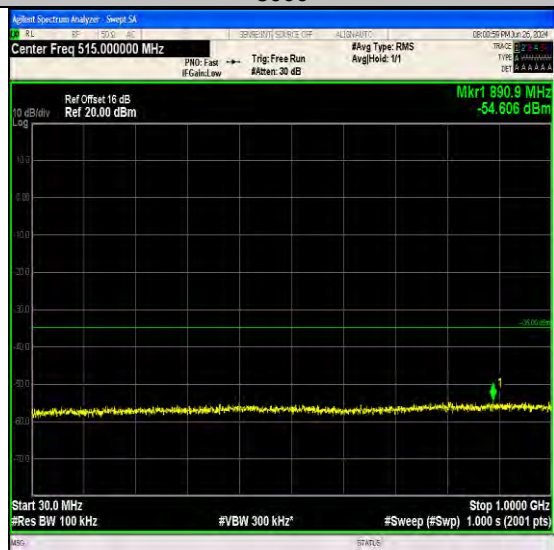
Band7_15MHz_64QAM_21100_75RB#0_30~1000_30~1000
