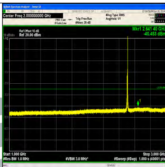
Band7_10MHz_64QAM_20800_1RB#49_1000~3000_1000~3000
