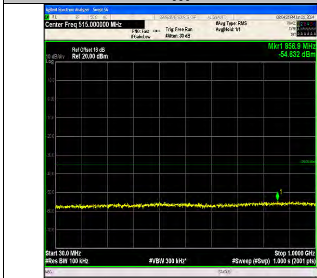
Band7_15MHz_QPSK_21375_75RB#0_30~1000_30~1000
