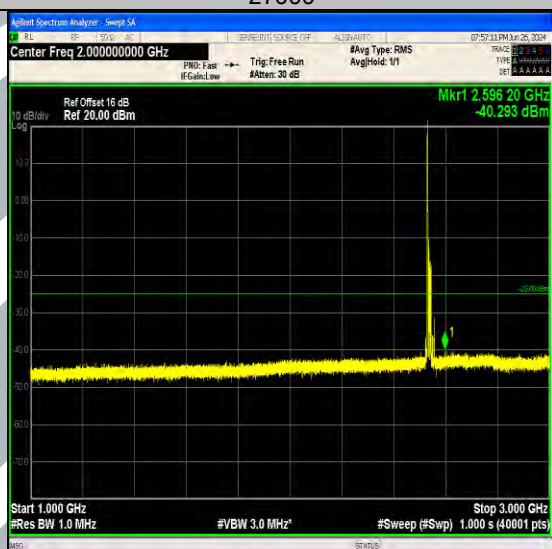
Band7_15MHz_QPSK_21100_1RB#0_1000~3000_1000~3000
