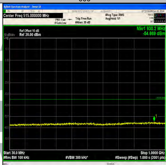
Band7_15MHz_QPSK_21100_1RB#0_30~1000_30~1000
