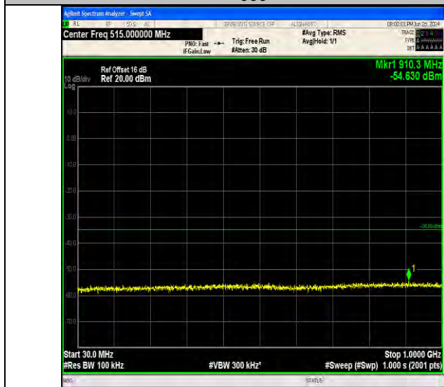
Band7_15MHz_QPSK_21100_75RB#0_30~1000_30~1000
