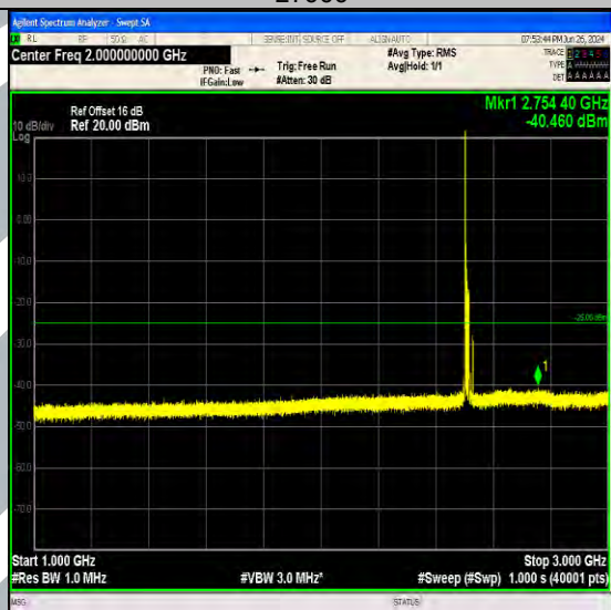
Band7_15MHz_64QAM_20825_1RB#0_1000~3000_1000~3000
