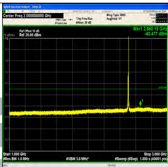
Band7_10MHz_QPSK_20800_1RB#49_1000~3000_1000~3000
