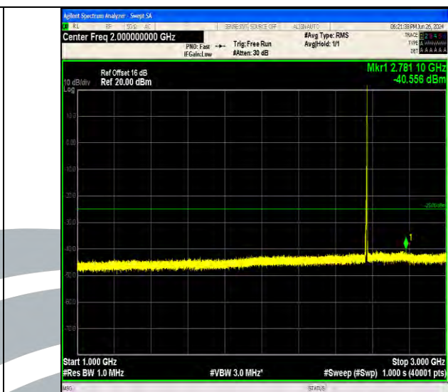
Band7_5MHz_64QAM_21425_1RB#24_1000~3000_1000~3000
