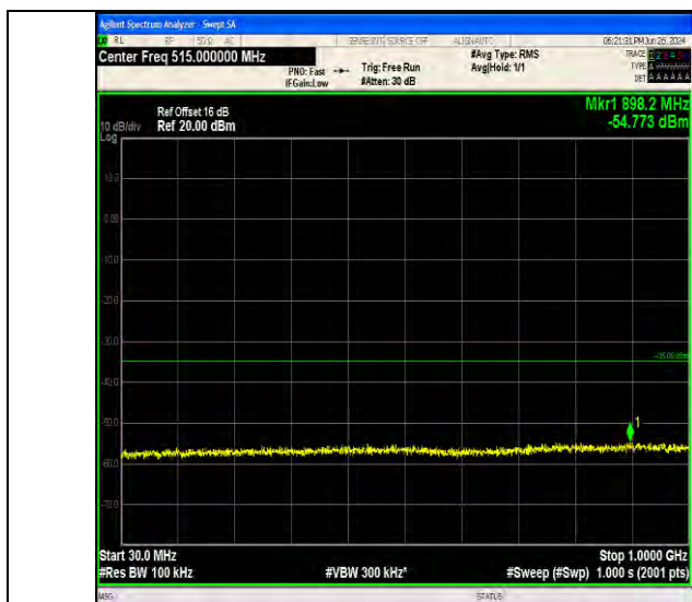
Band7_5MHz_64QAM_21425_1RB#24_30~1000_30~1000
