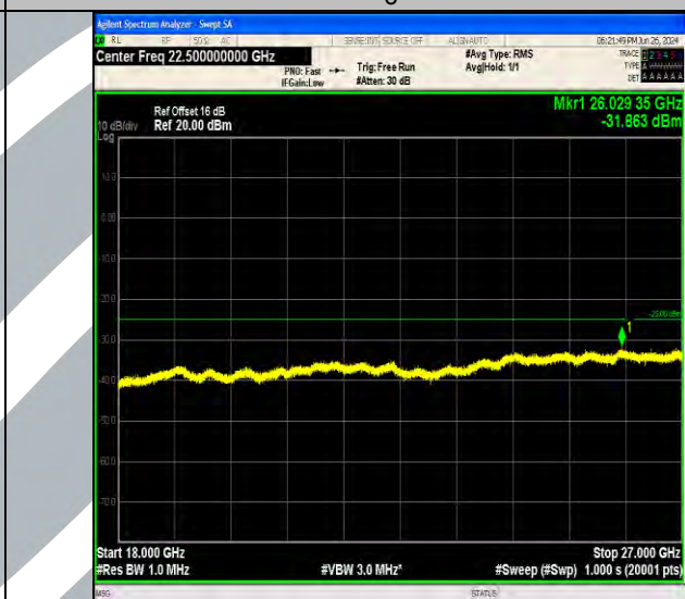
Band7_5MHz_64QAM_21425_1RB#24_18000~27000_18000~27000
