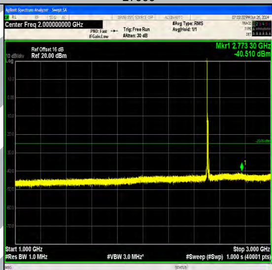
Band7_10MHz_QPSK_20800_1RB#0_1000~3000_1000~3000
