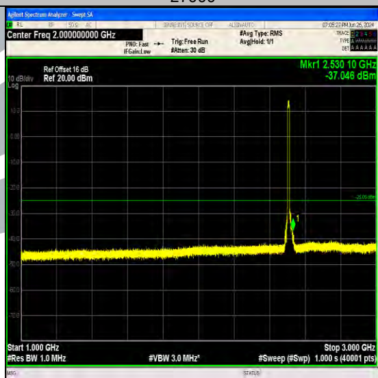
Band7_10MHz_QPSK_20800_50RB#0_1000~3000_1000~3000
