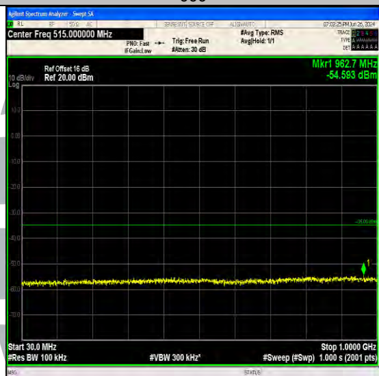
Band7_10MHz_QPSK_20800_1RB#0_30~1000_30~1000
