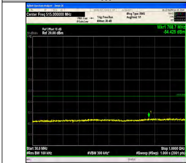
Band7_5MHz_64QAM_21425_25RB#0_30~1000_30~1000
