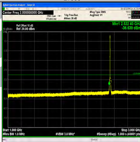
Band7_5MHz_16QAM_21100_25RB#0_1000~3000_1000~3000
