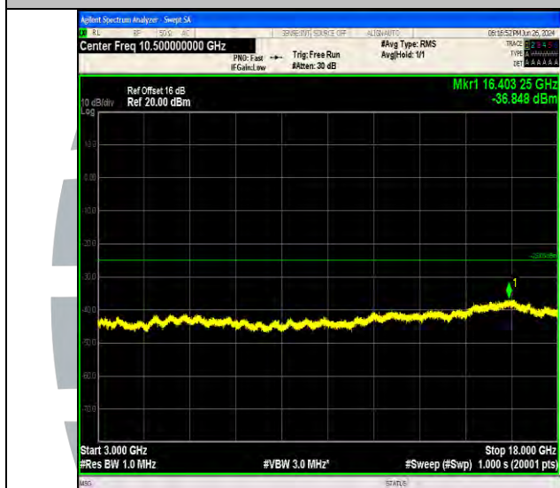
Band7_5MHz_16QAM_21100_1RB#24_3000~18000_3000~18000
