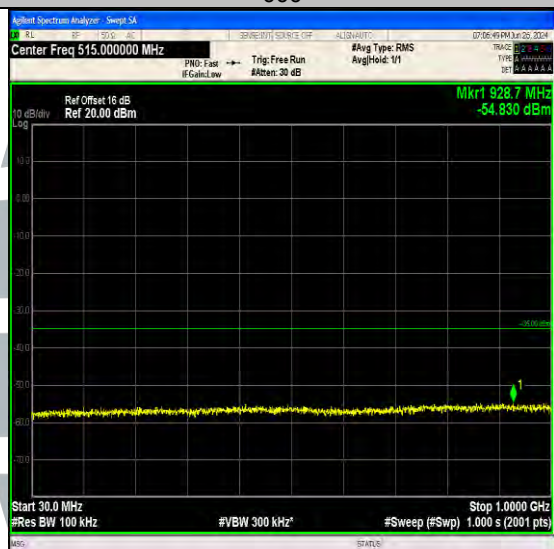
Band7_10MHz_QPSK_21100_1RB#0_30~1000_30~1000
