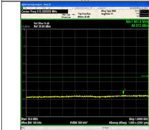
Band7_5MHz_16QAM_21100_25RB#0_30~1000_30~1000
