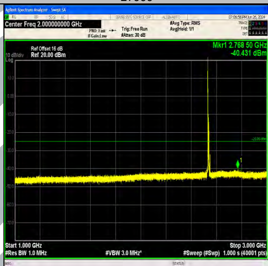
Band7_10MHz_QPSK_21100_1RB#0_1000~3000_1000~3000
