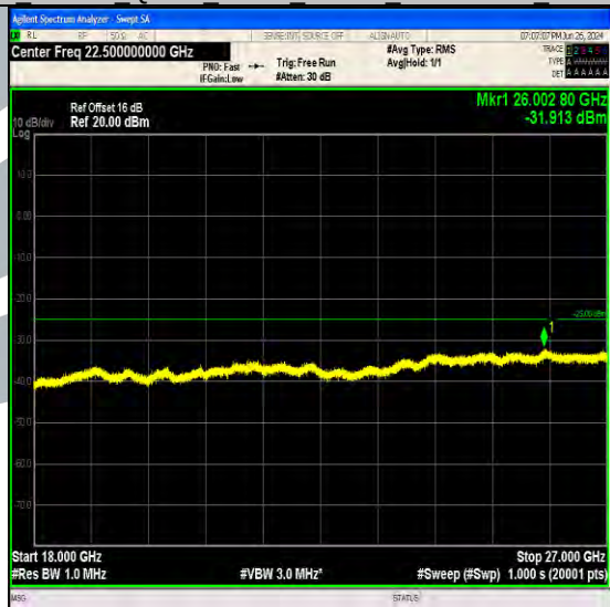
Band7_10MHz_QPSK_21100_1RB#0_18000~27000_18000~27000
