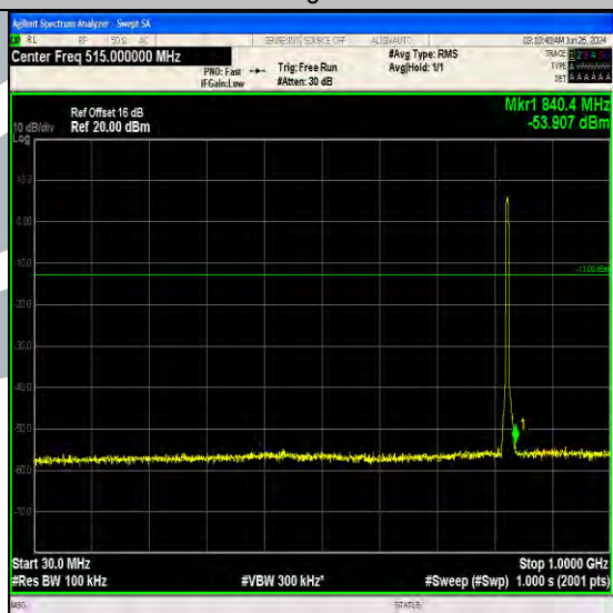
Band5_5MHz_64QAM_20425_25RB#0_30~1000_30~1000
