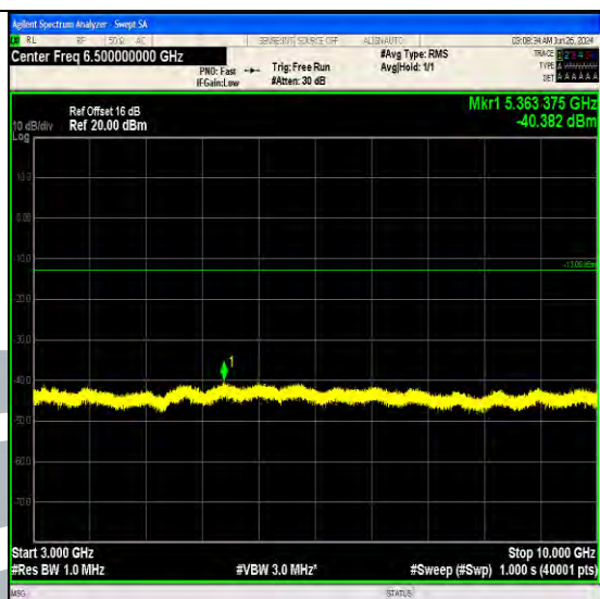
Band5_5MHz_64QAM_20425_1RB#0_3000~10000_3000~10000
