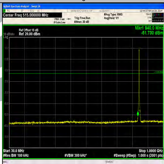
Band5_3MHz_16QAM_20635_15RB#0_30~1000_30~1000
