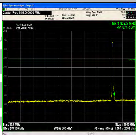
Band5_5MHz_QPSK_20425_25RB#0_30~1000_30~1000
