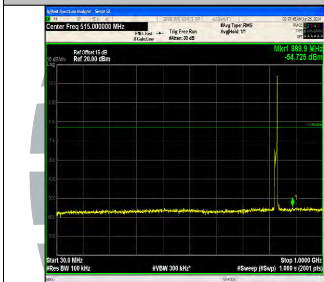
Band5_10MHz_QPSK_20450_1RB#49_30~1000_30~1000
