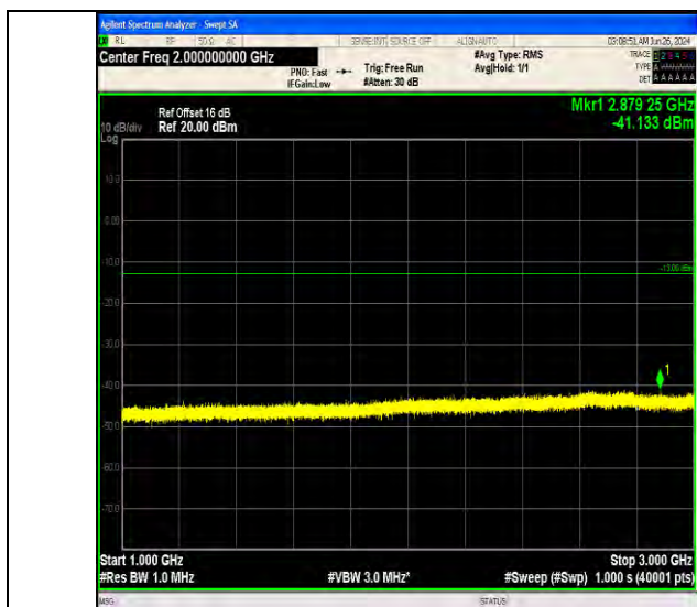
Band5_5MHz_QPSK_20425_1RB#24_1000~3000_1000~3000
