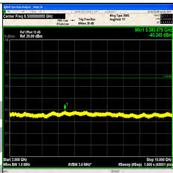
Band5_3MHz_16QAM_20635_1RB#0_3000~10000_3000~10000
