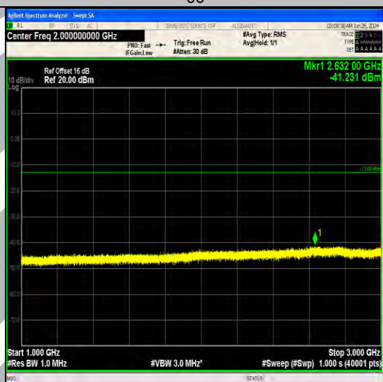
Band5_5MHz_64QAM_20425_1RB#24_1000~3000_1000~3000
