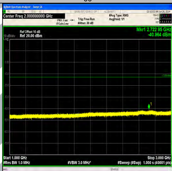
Band5_5MHz_QPSK_20425_25RB#0_1000~3000_1000~3000
