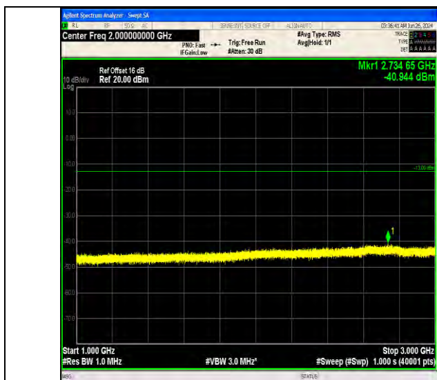
Band5_10MHz_QPSK_20450_1RB#0_1000~3000_1000~3000
