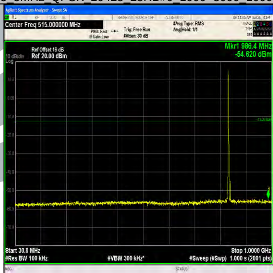
Band5_5MHz_QPSK_20525_1RB#0_30~1000_30~1000
