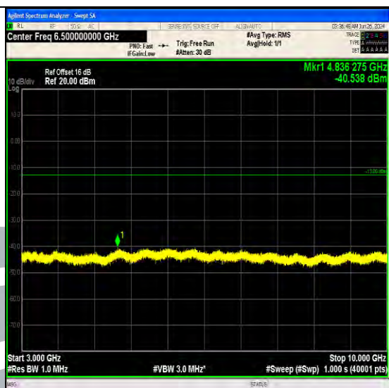
Band5_10MHz_QPSK_20450_1RB#0_3000~10000_3000~10000
