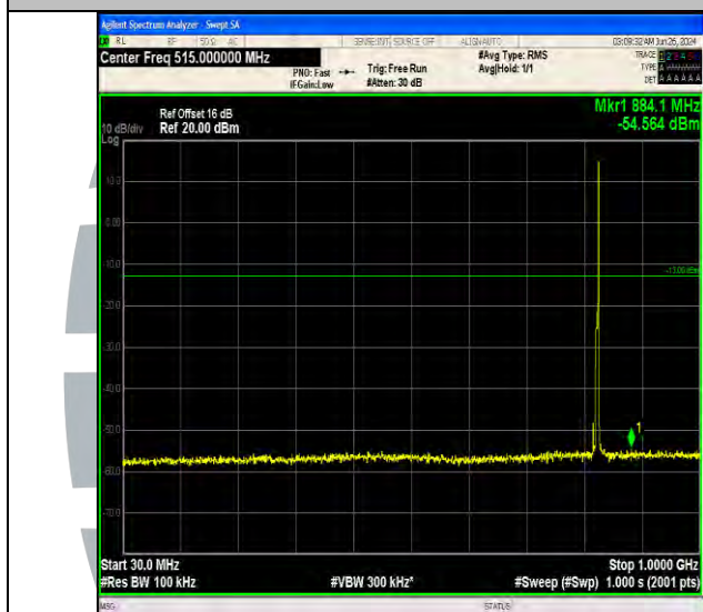
Band5_5MHz_64QAM_20425_1RB#24_30~1000_30~1000
