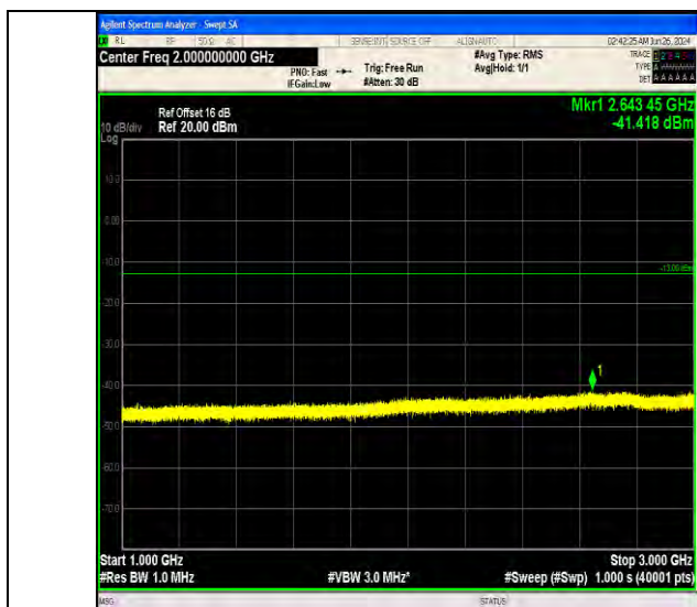
Band5_3MHz_16QAM_20635_1RB#0_1000~3000_1000~3000
