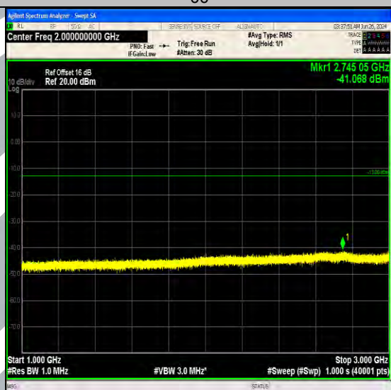
Band5_10MHz_QPSK_20450_1RB#49_1000~3000_1000~3000
