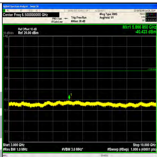
Band5_5MHz_QPSK_20425_1RB#24_3000~10000_3000~10000
