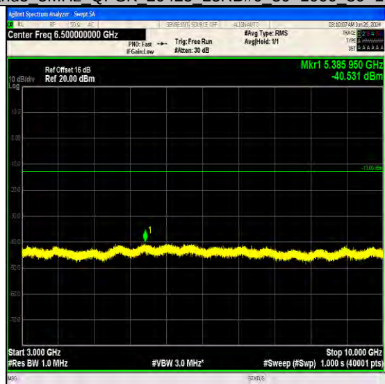
Band5_5MHz_QPSK_20425_25RB#0_3000~10000_3000~10000
