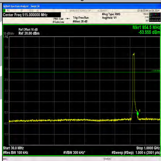
Band5_10MHz_QPSK_20450_50RB#0_30~1000_30~1000
