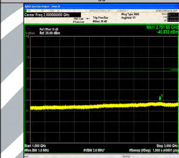
Band5_1.4MHz_QPSK_20643_6RB#0_1000~3000_1000~3000
