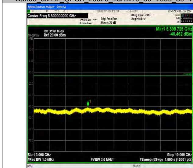
Band5_3MHz_QPSK_20525_15RB#0_3000~10000_3000~10000
