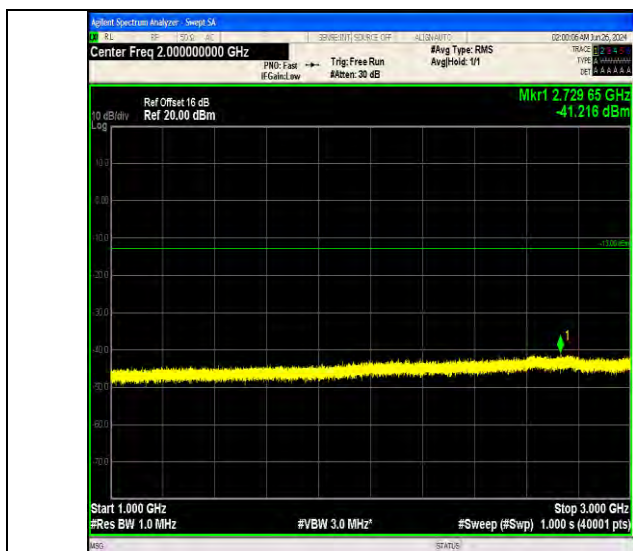
Band5_1.4MHz_QPSK_20407_1RB#5_1000~3000_1000~3000
