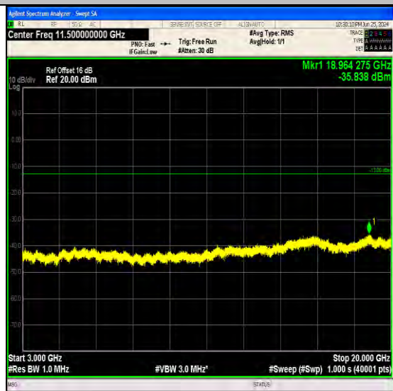
Band4_20MHz_QPSK_20175_100RB#0_3000~20000_3000~20000
