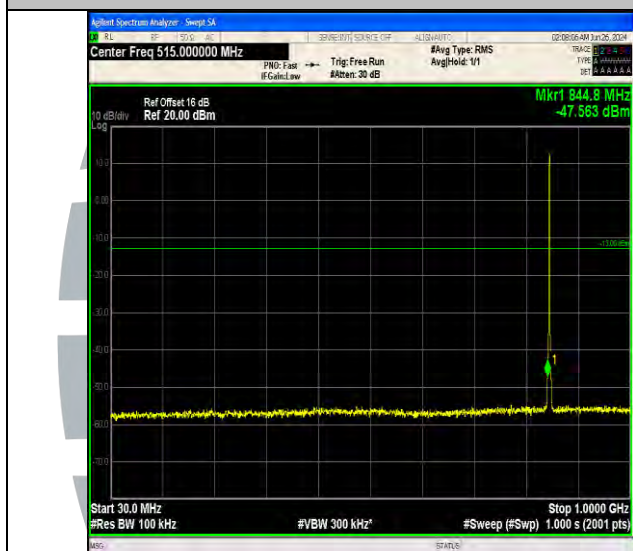
Band5_1.4MHz_QPSK_20643_6RB#0_30~1000_30~1000
