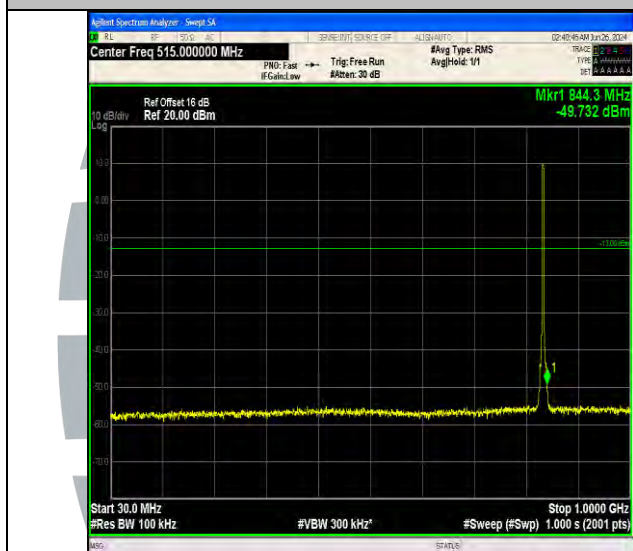
Band5_3MHz_QPSK_20525_15RB#0_30~1000_30~1000
