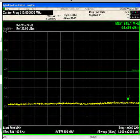
Band4_20MHz_QPSK_20175_100RB#0_30~1000_30~1000
