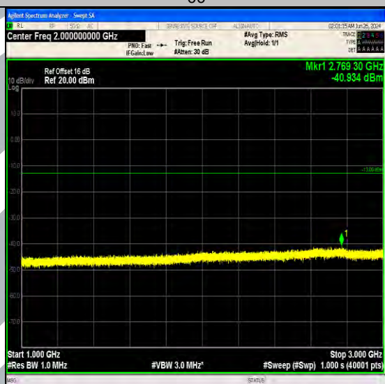
Band5_1.4MHz_QPSK_20407_6RB#0_1000~3000_1000~3000
