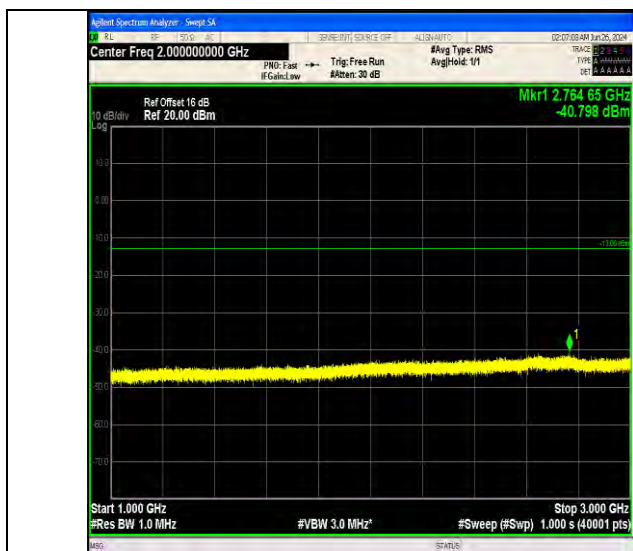
Band5_1.4MHz_QPSK_20643_1RB#5_1000~3000_1000~3000
