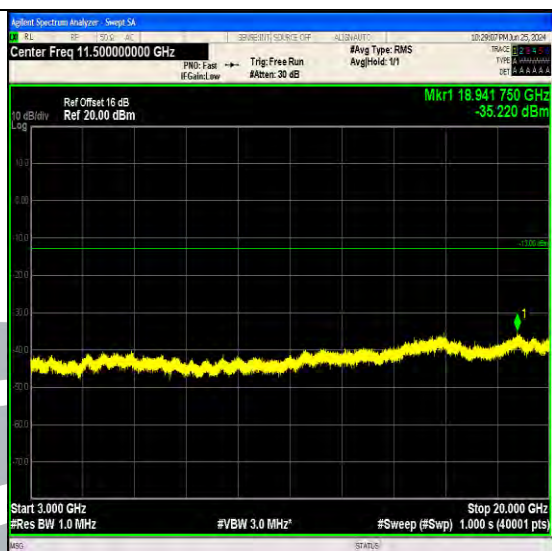
Band4_20MHz_QPSK_20175_1RB#99_3000~20000_3000~20000
