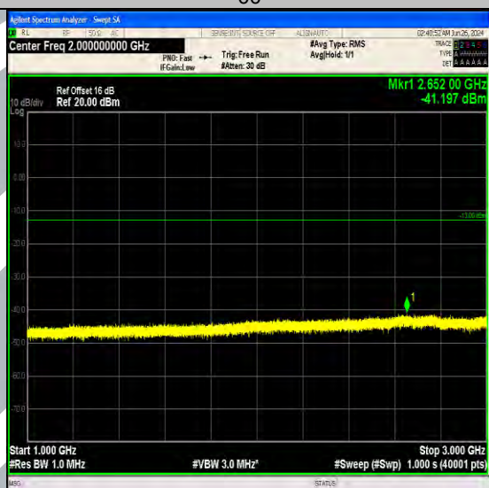
Band5_3MHz_QPSK_20525_15RB#0_1000~3000_1000~3000
