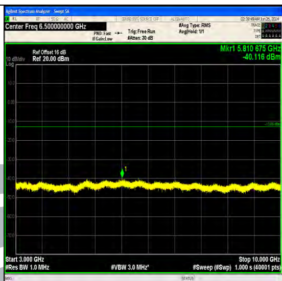
Band5_3MHz_QPSK_20525_1RB#14_3000~10000_3000~10000
