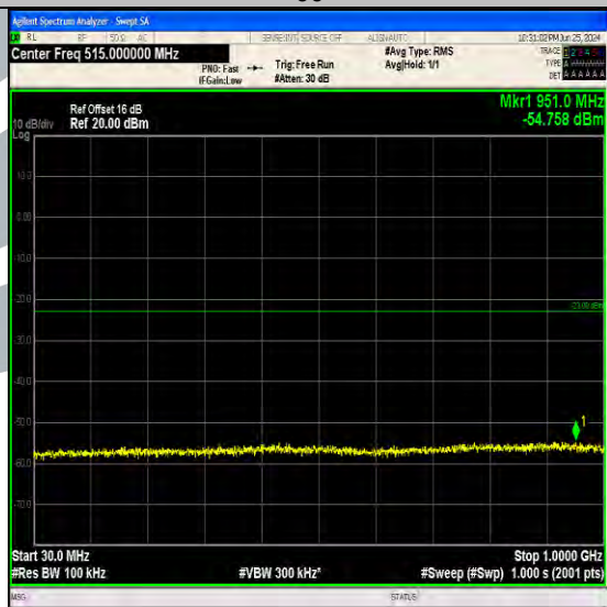
Band4_20MHz_QPSK_20300_1RB#0_30~1000_30~1000
