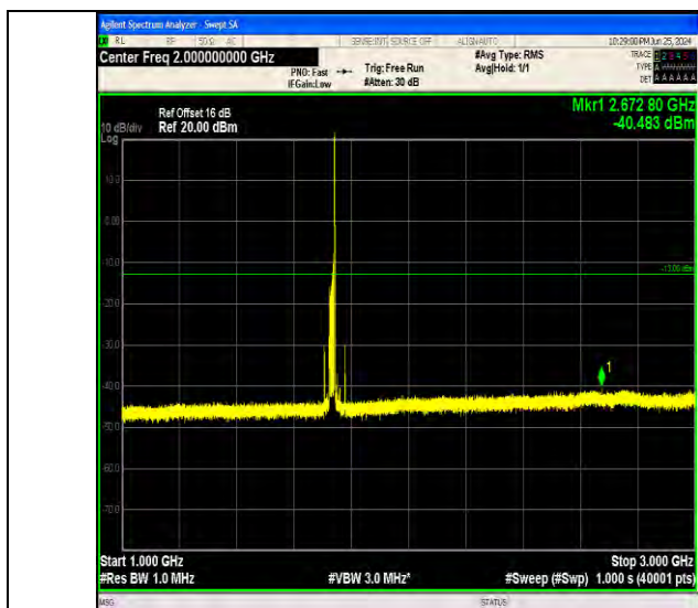
Band4_20MHz_QPSK_20175_1RB#99_1000~3000_1000~3000
