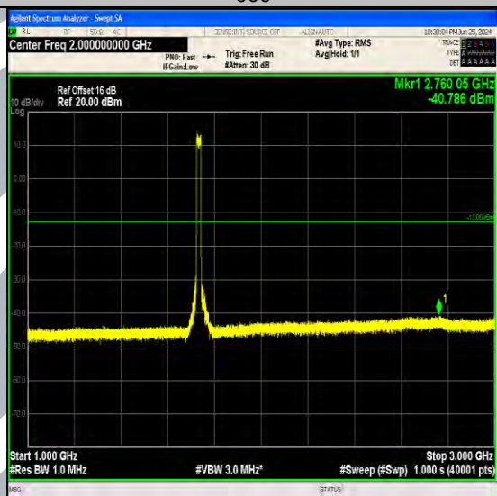
Band4_20MHz_QPSK_20175_100RB#0_1000~3000_1000~3000
