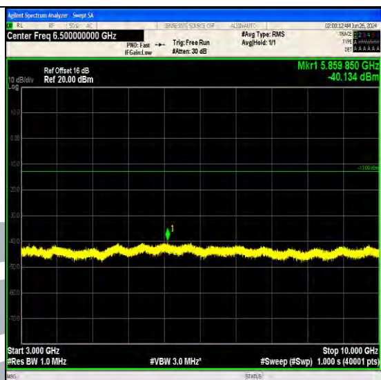
Band5_1.4MHz_QPSK_20407_1RB#5_3000~10000_3000~10000
