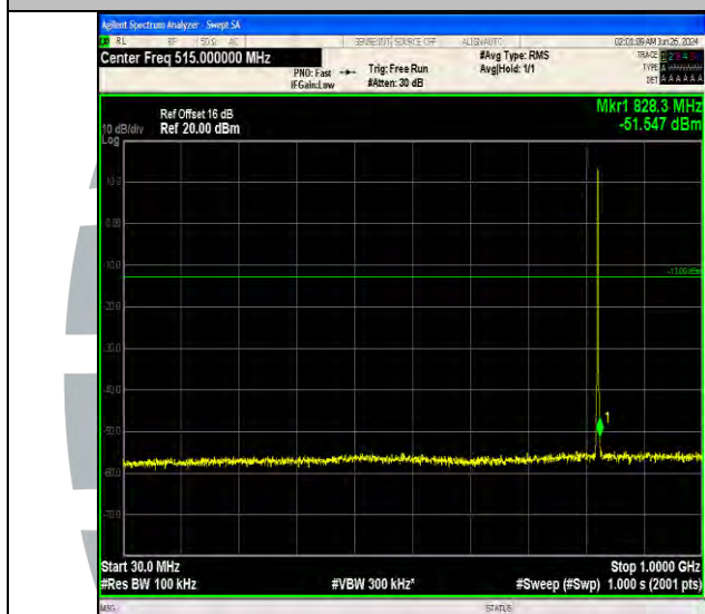
Band5_1.4MHz_QPSK_20407_6RB#0_30~1000_30~1000
