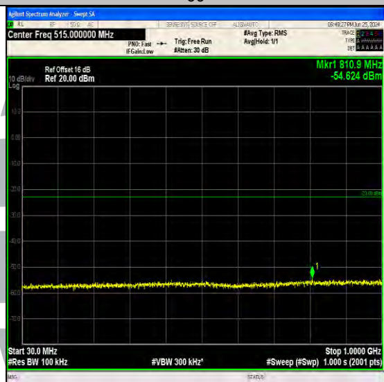
Band4_15MHz_16QAM_20325_75RB#0_30~1000_30~1000
