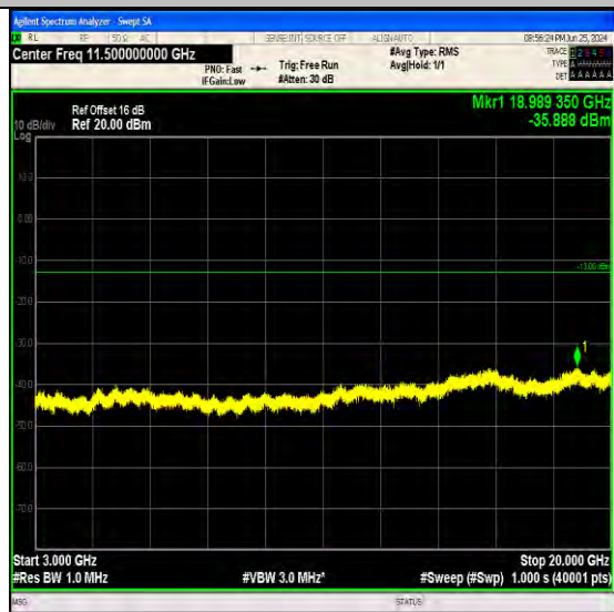
Band4_10MHz_64QAM_20000_50RB#0_3000~20000_3000~20000
