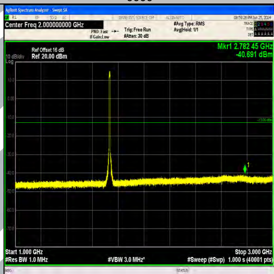
Band4_10MHz_16QAM_20175_50RB#0_1000~3000_1000~3000
