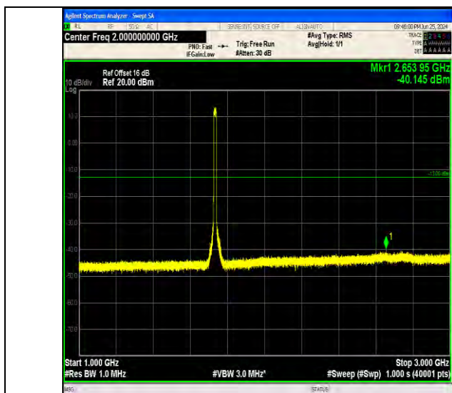
Band4_15MHz_16QAM_20175_75RB#0_1000~3000_1000~3000
