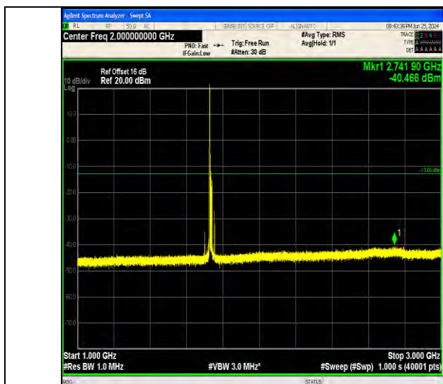
Band4_15MHz_16QAM_20175_1RB#0_1000~3000_1000~3000
