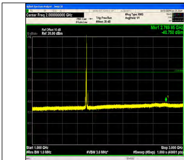
Band4_10MHz_64QAM_20000_1RB#49_1000~3000_1000~3000
