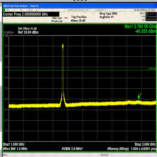
Band4_15MHz_64QAM_20175_75RB#0_1000~3000_1000~3000
