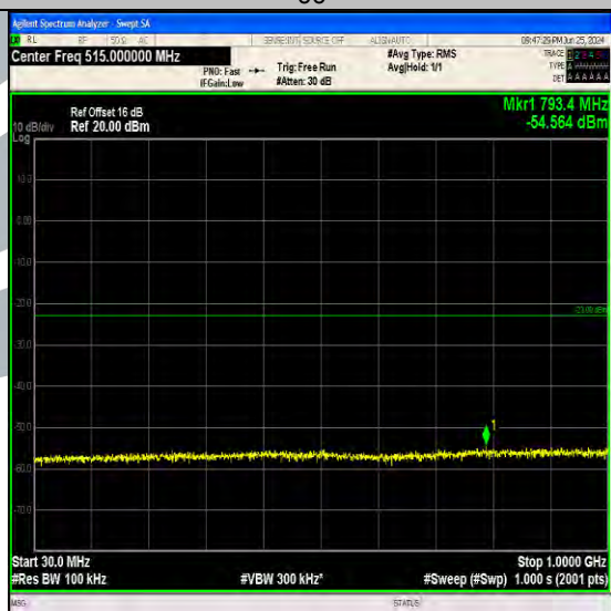
Band4_15MHz_64QAM_20325_1RB#0_30~1000_30~1000
