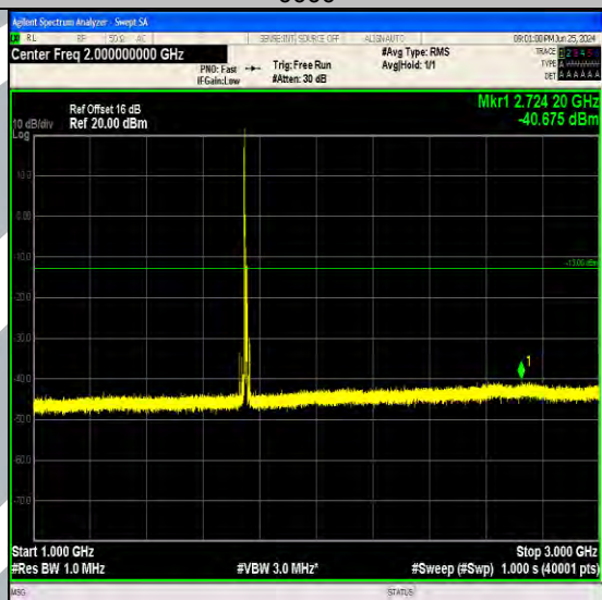
Band4_10MHz_64QAM_20350_1RB#0_1000~3000_1000~3000
