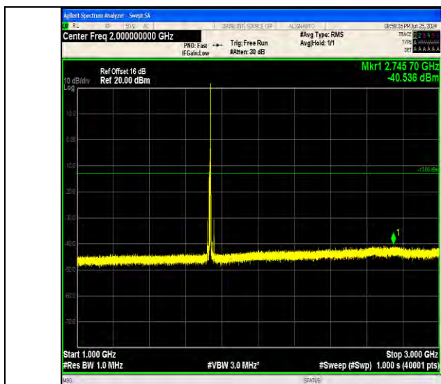
Band4_10MHz_16QAM_20175_1RB#49_1000~3000_1000~3000
