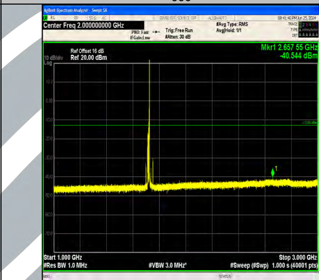
Band4_15MHz_64QAM_20025_1RB#74_1000~3000_1000~3000
