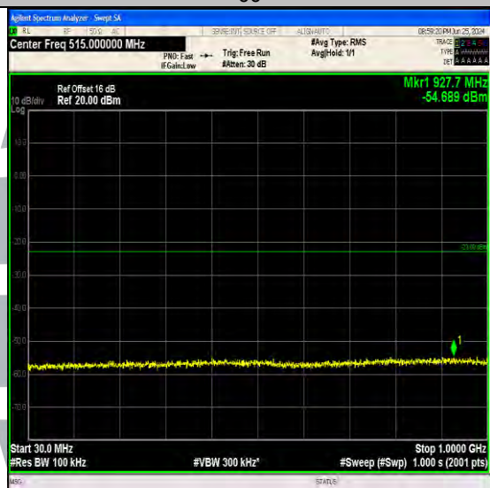
Band4_10MHz_16QAM_20175_50RB#0_30~1000_30~1000
