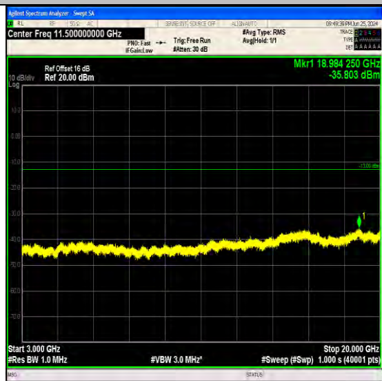
Band4_15MHz_16QAM_20325_75RB#0_3000~20000_3000~20000
