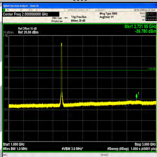
Band4_10MHz_64QAM_20000_50RB#0_1000~3000_1000~3000
