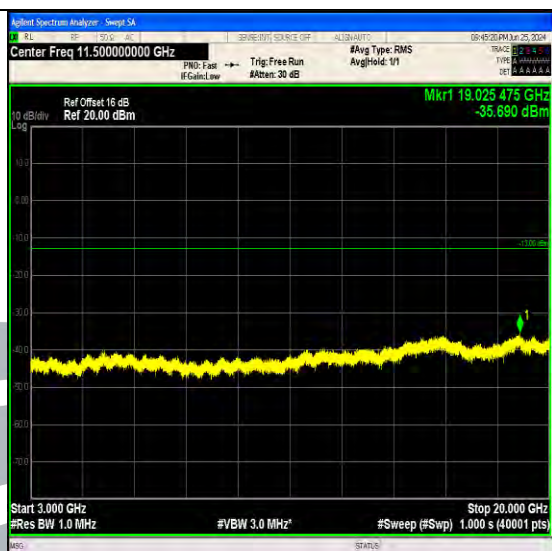
Band4_15MHz_64QAM_20175_1RB#74_3000~20000_3000~20000
