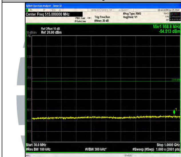
Band4_15MHz_16QAM_20175_1RB#74_30~1000_30~1000
