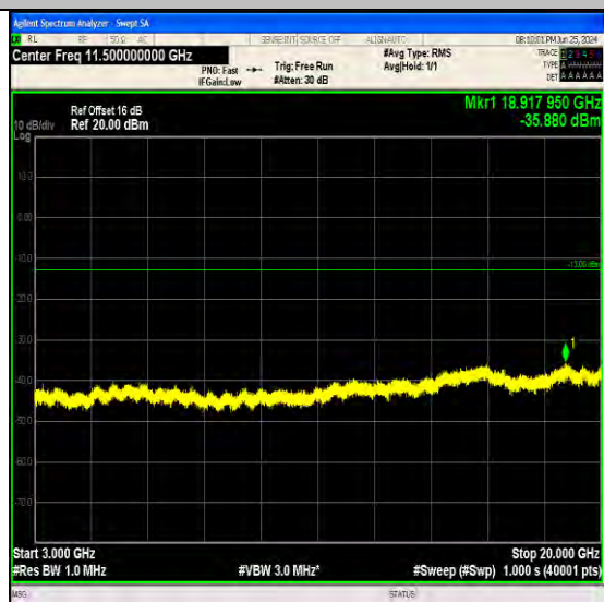
Band4_5MHz_16QAM_20175_1RB#24_3000~20000_3000~20000
