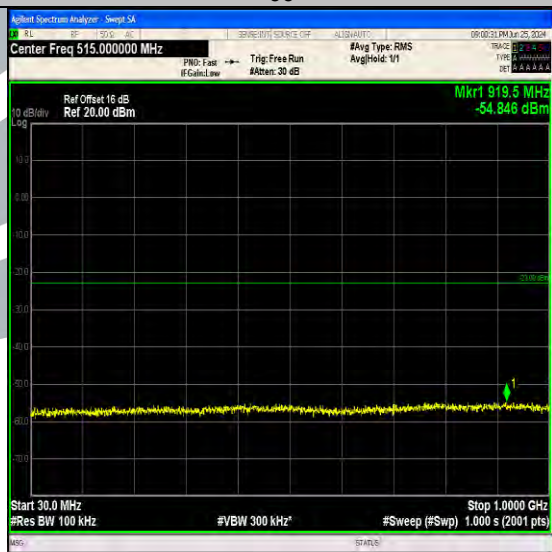
Band4_10MHz_16QAM_20350_1RB#0_30~1000_30~1000
