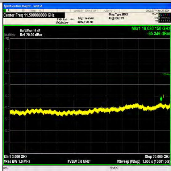
Band4_10MHz_64QAM_20350_1RB#0_3000~20000_3000~20000
