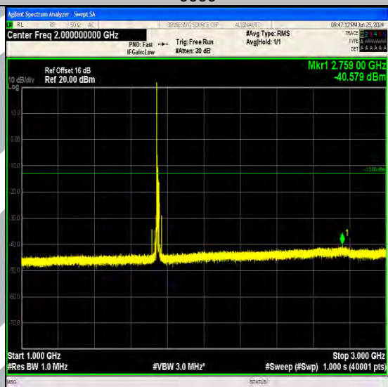
Band4_15MHz_16QAM_20325_1RB#0_1000~3000_1000~3000
