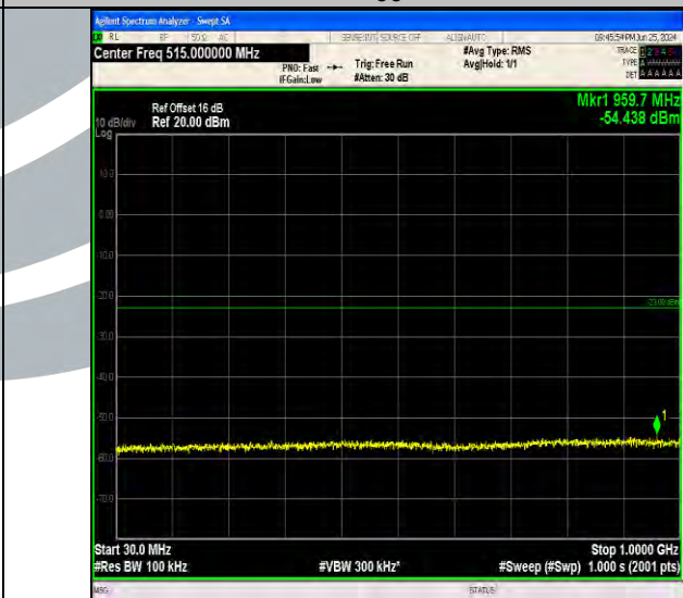
Band4_15MHz_16QAM_20175_75RB#0_30~1000_30~1000
