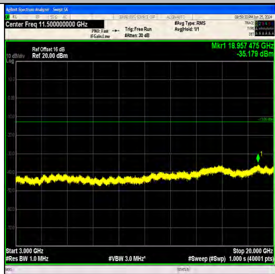
Band4_10MHz_16QAM_20175_50RB#0_3000~20000_3000~20000
