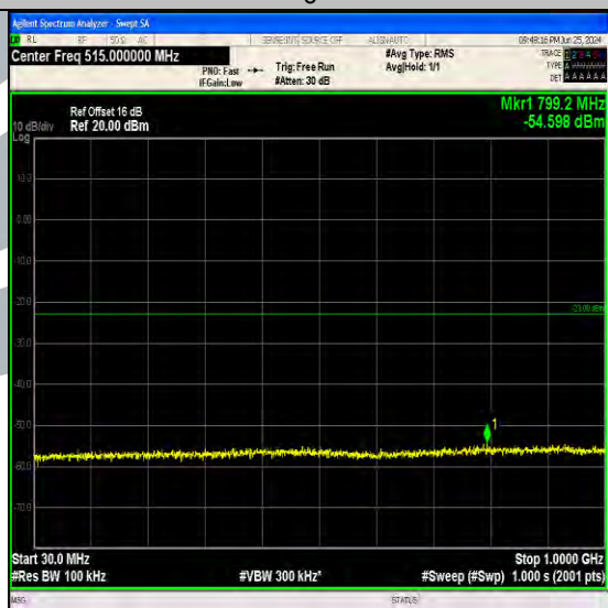
Band4_15MHz_16QAM_20325_1RB#74_30~1000_30~1000
