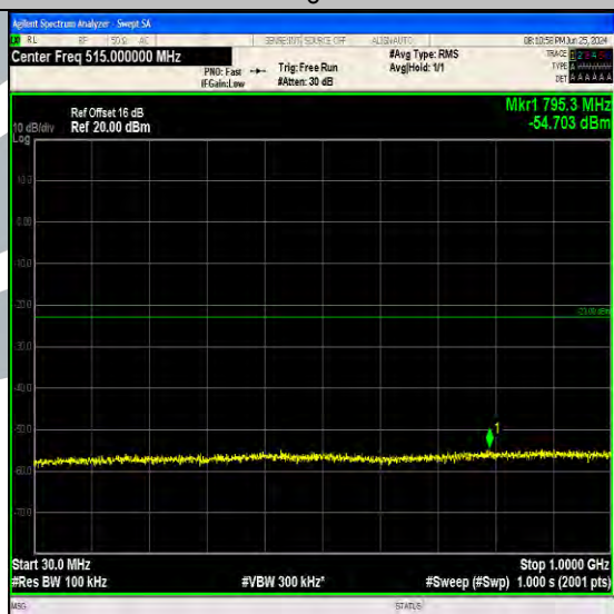
Band4_5MHz_16QAM_20175_25RB#0_30~1000_30~1000
