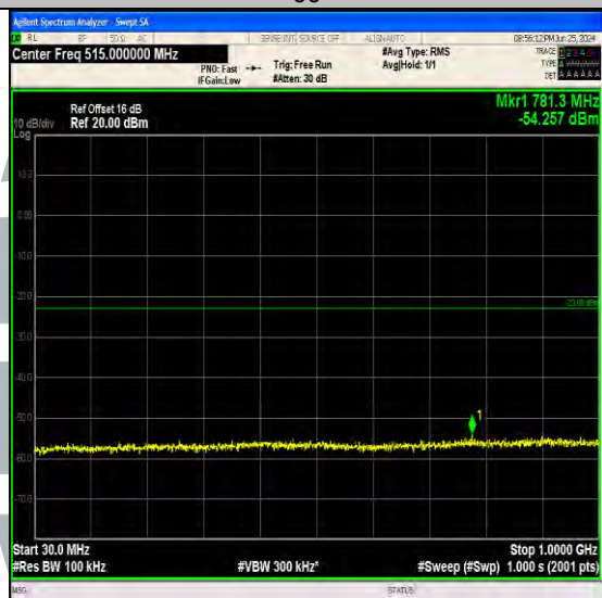
Band4_10MHz_64QAM_20000_50RB#0_30~1000_30~1000
