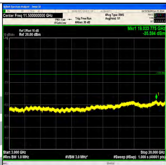
Band4_10MHz_64QAM_20175_50RB#0_3000~20000_3000~20000
