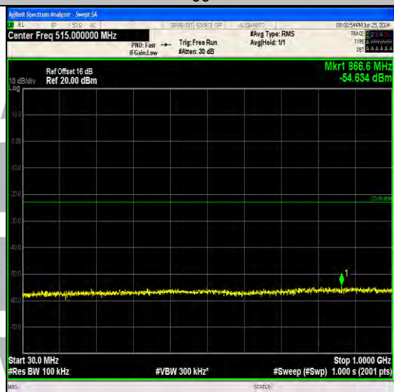
Band4_10MHz_64QAM_20350_1RB#0_30~1000_30~1000
