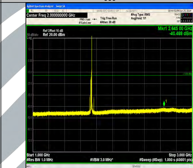
Band4_15MHz_16QAM_20175_1RB#74_1000~3000_1000~3000
