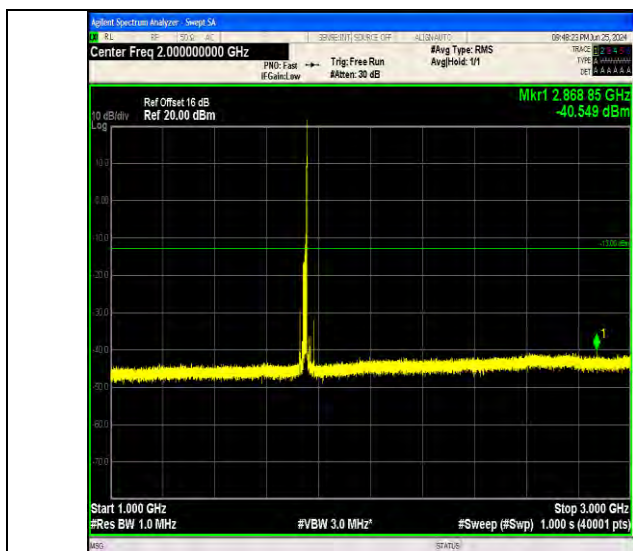
Band4_15MHz_16QAM_20325_1RB#74_1000~3000_1000~3000
