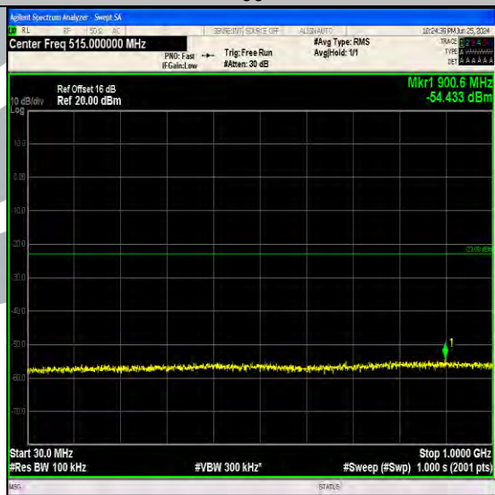
Band4_20MHz_QPSK_20050_1RB#0_30~1000_30~1000
