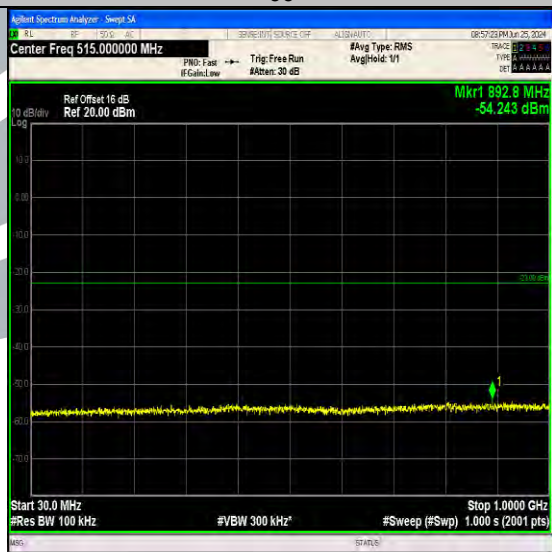
Band4_10MHz_64QAM_20175_1RB#0_30~1000_30~1000
