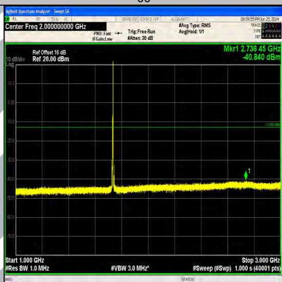
Band4_5MHz_16QAM_20175_1RB#24_1000~3000_1000~3000
