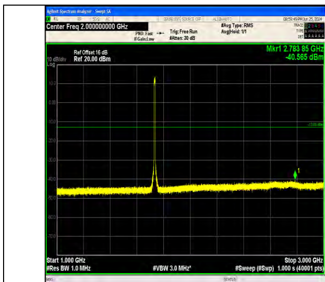
Band4_10MHz_64QAM_20175_50RB#0_1000~3000_1000~3000
