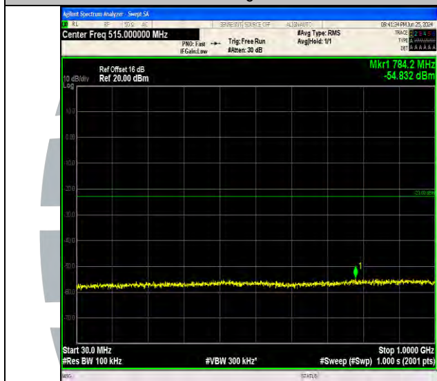
Band4_15MHz_64QAM_20025_1RB#74_30~1000_30~1000
