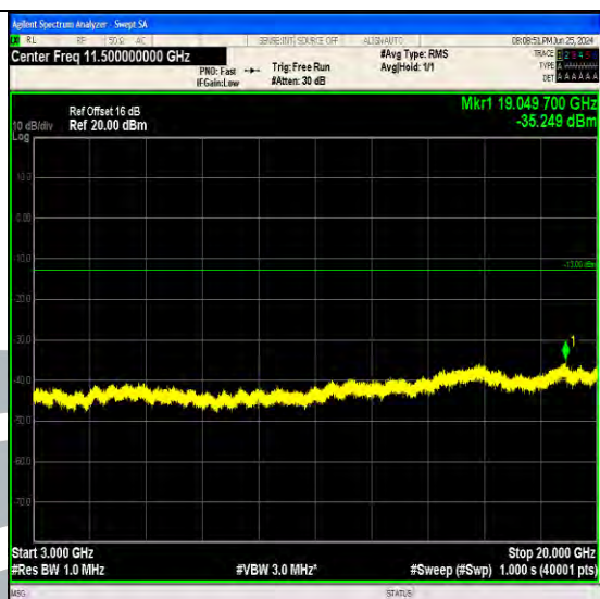
Band4_5MHz_16QAM_20175_1RB#0_3000~20000_3000~20000
