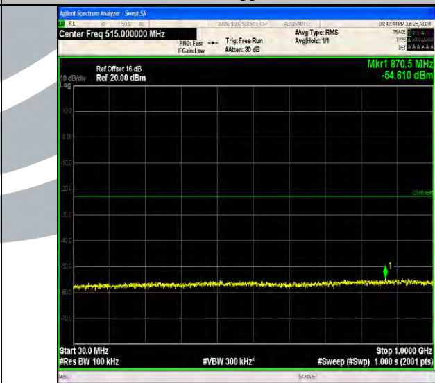
Band4_15MHz_64QAM_20025_75RB#0_30~1000_30~1000
