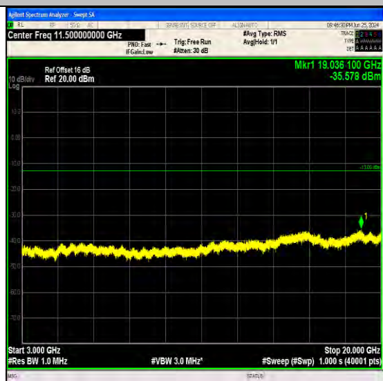
Band4_15MHz_64QAM_20175_75RB#0_3000~20000_3000~20000
