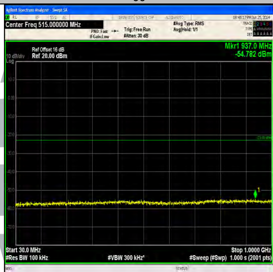
Band4_15MHz_64QAM_20175_75RB#0_30~1000_30~1000
