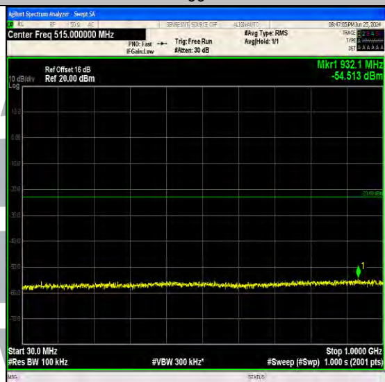
Band4_15MHz_16QAM_20325_1RB#0_30~1000_30~1000
