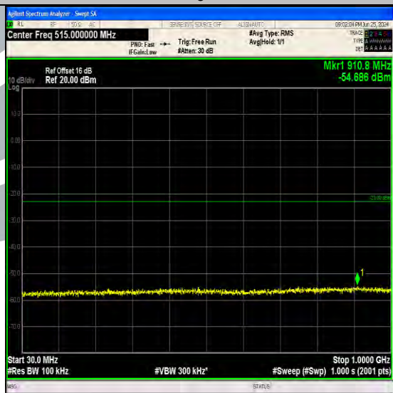
Band4_10MHz_64QAM_20350_1RB#49_30~1000_30~1000
