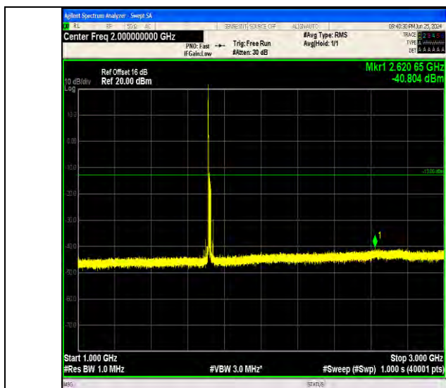
Band4_15MHz_64QAM_20025_1RB#0_1000~3000_1000~3000
