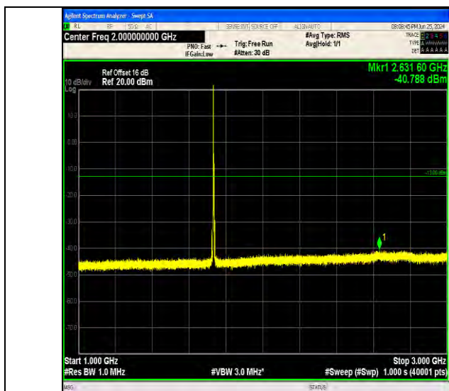
Band4_5MHz_16QAM_20175_1RB#0_1000~3000_1000~3000
