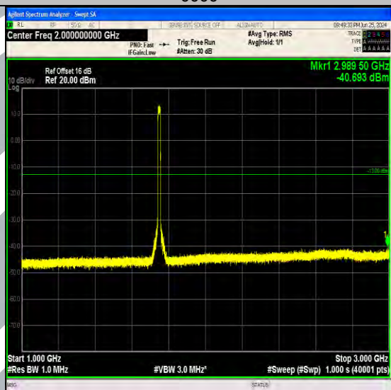
Band4_15MHz_16QAM_20325_75RB#0_1000~3000_1000~3000
