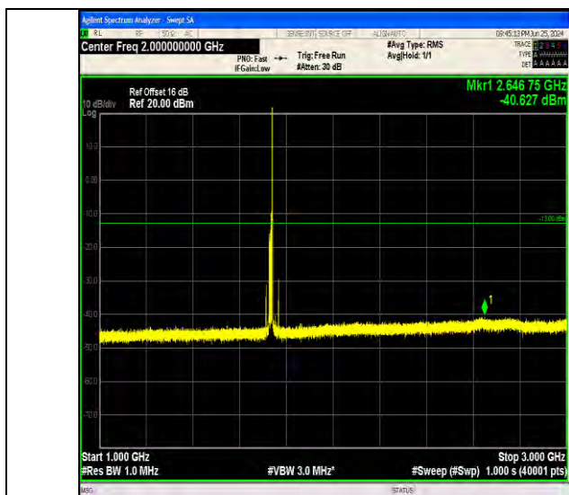
Band4_15MHz_64QAM_20175_1RB#74_1000~3000_1000~3000
