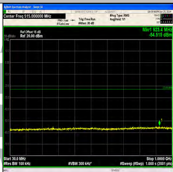
Band4_5MHz_16QAM_20175_1RB#24_30~1000_30~1000
