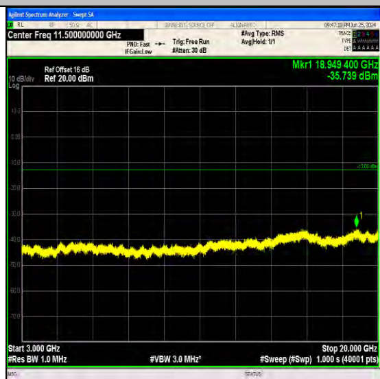
Band4_15MHz_16QAM_20325_1RB#0_3000~20000_3000~20000
