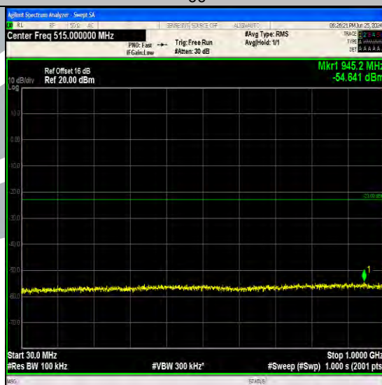
Band4_1.4MHz_16QAM_20393_1RB#5_30~1000_30~1000
