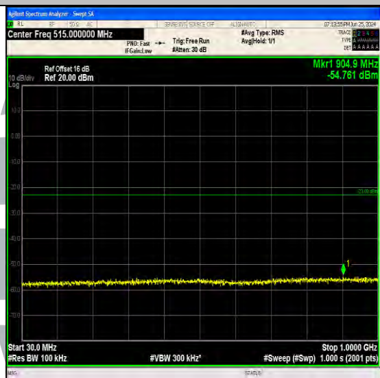
Band4_3MHz_QPSK_19965_1RB#14_30~1000_30~1000
