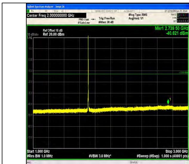
Band4_3MHz_QPSK_19965_1RB#0_1000~3000_1000~3000
