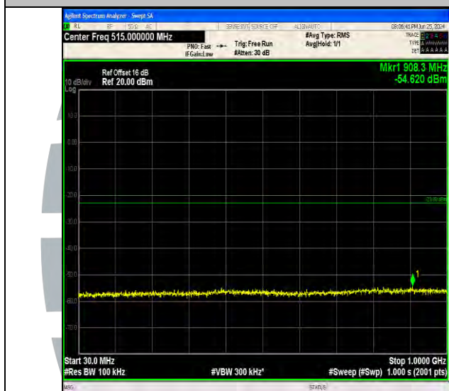
Band4_5MHz_64QAM_19975_1RB#24_30~1000_30~1000
