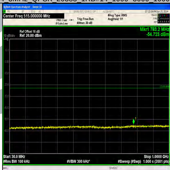
Band4_3MHz_QPSK_20385_15RB#0_30~1000_30~1000
