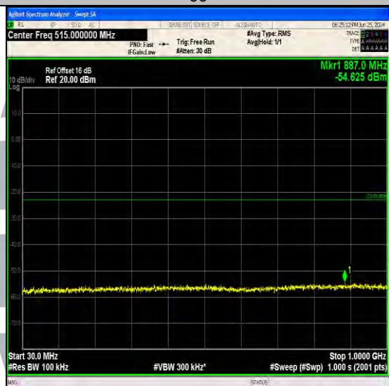
Band4_1.4MHz_16QAM_20393_1RB#0_30~1000_30~1000
