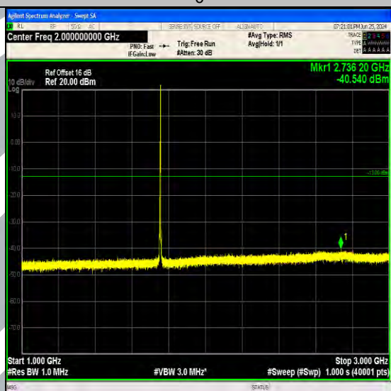
Band4_3MHz_QPSK_20385_1RB#14_1000~3000_1000~3000
