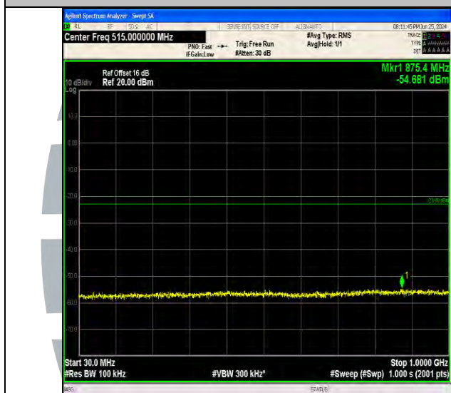
Band4_5MHz_QPSK_20375_1RB#0_30~1000_30~1000
