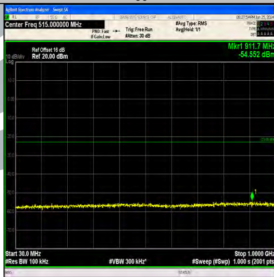
Band4_1.4MHz_64QAM_20393_6RB#0_30~1000_30~1000
