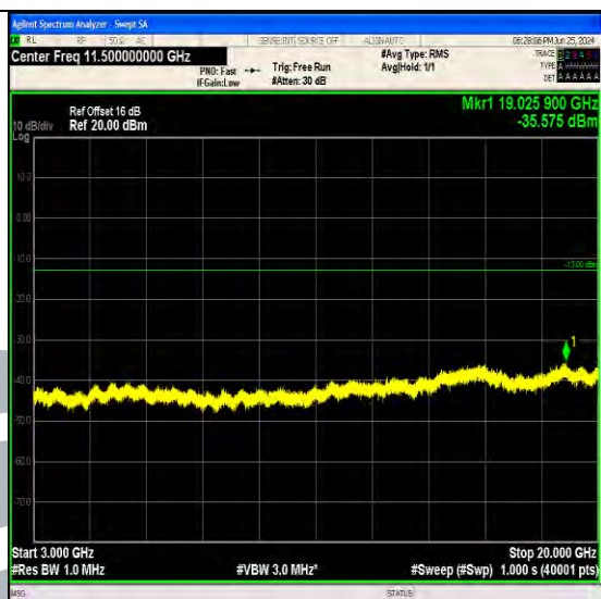
Band4_1.4MHz_64QAM_20393_6RB#0_3000~20000_3000~20000
