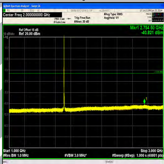
Band4_3MHz_QPSK_19965_1RB#14_1000~3000_1000~3000
