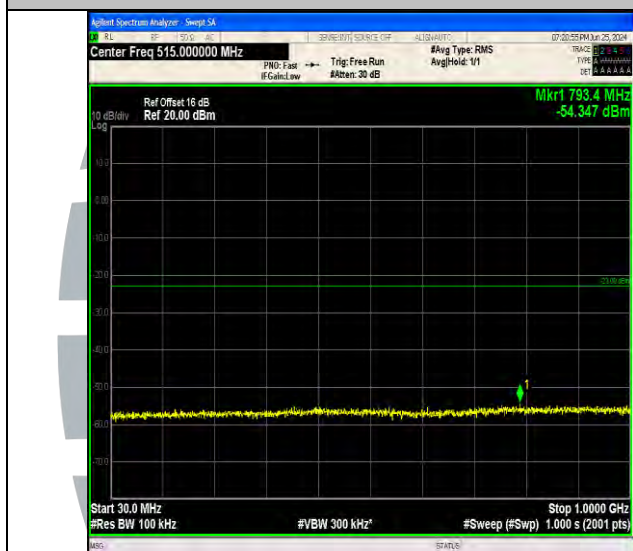
Band4_3MHz_QPSK_20385_1RB#14_30~1000_30~1000
