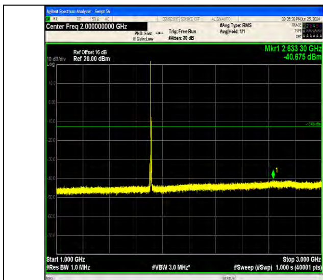
Band4_5MHz_64QAM_19975_1RB#0_1000~3000_1000~3000
