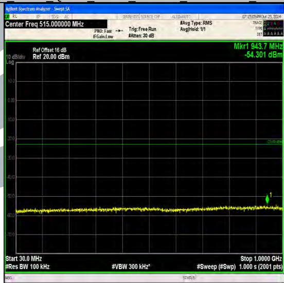
Band4_3MHz_QPSK_19965_15RB#0_30~1000_30~1000
