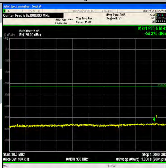
Band4_5MHz_64QAM_19975_25RB#0_30~1000_30~1000
