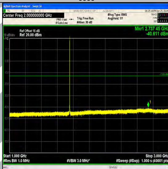
Band4_1.4MHz_16QAM_20393_1RB#0_1000~3000_1000~3000
