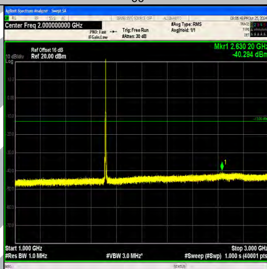
Band4_5MHz_64QAM_19975_1RB#24_1000~3000_1000~3000
