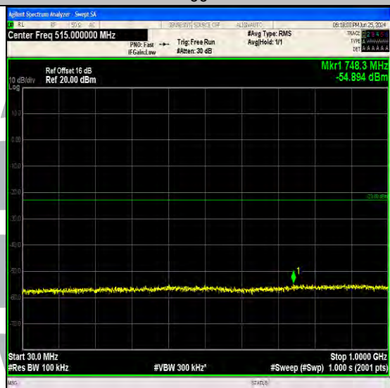
Band4_1.4MHz_16QAM_19957_1RB#0_30~1000_30~1000
