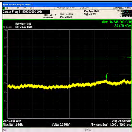
Band4_1.4MHz_16QAM_19957_1RB#0_3000~20000_3000~20000
