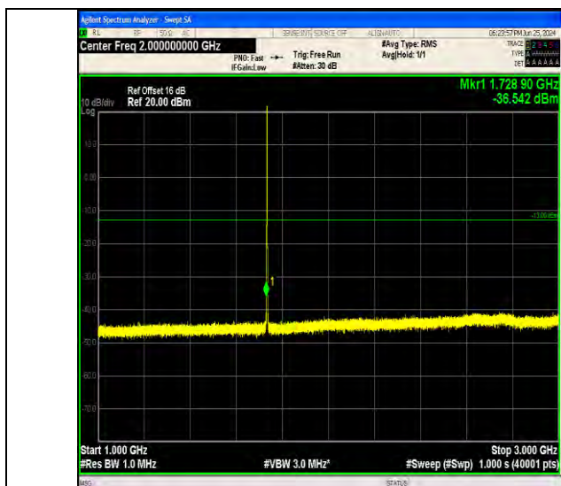
Band4_1.4MHz_16QAM_20175_6RB#0_1000~3000_1000~3000
