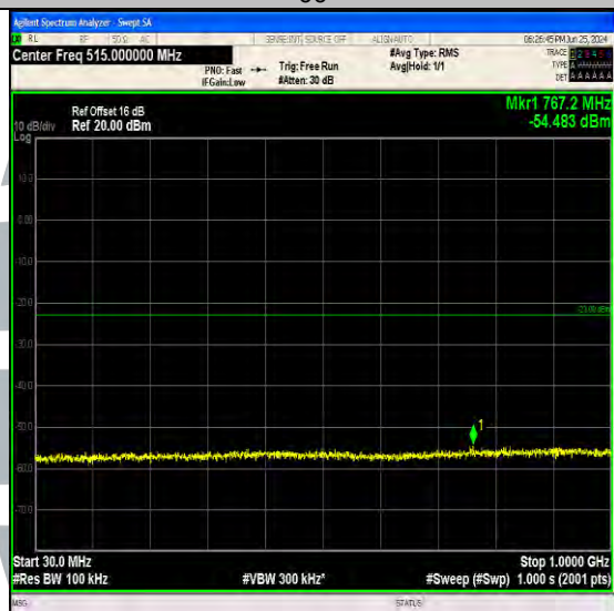
Band4_1.4MHz_64QAM_20393_1RB#5_30~1000_30~1000
