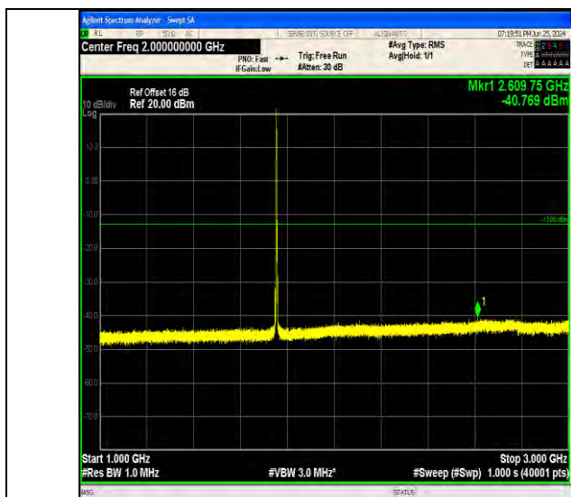
Band4_3MHz_QPSK_20385_1RB#0_1000~3000_1000~3000
