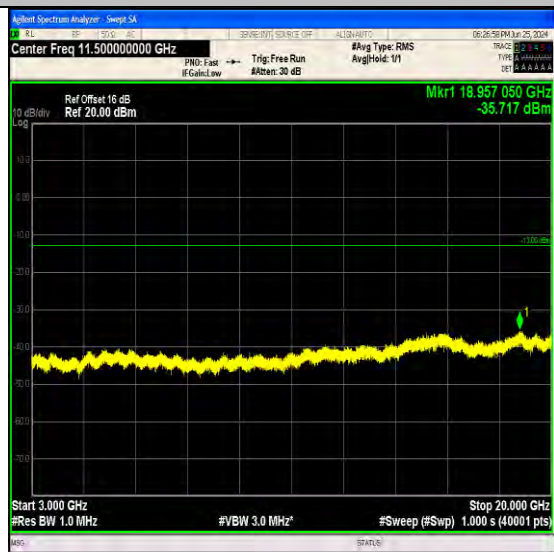
Band4_1.4MHz_64QAM_20393_1RB#5_3000~20000_3000~20000
