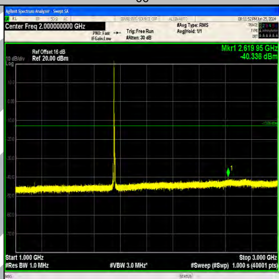
Band4_5MHz_QPSK_20375_1RB#0_1000~3000_1000~3000
