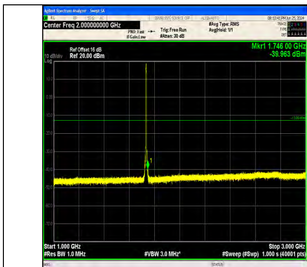
Band4_5MHz_QPSK_20175_25RB#0_1000~3000_1000~3000
