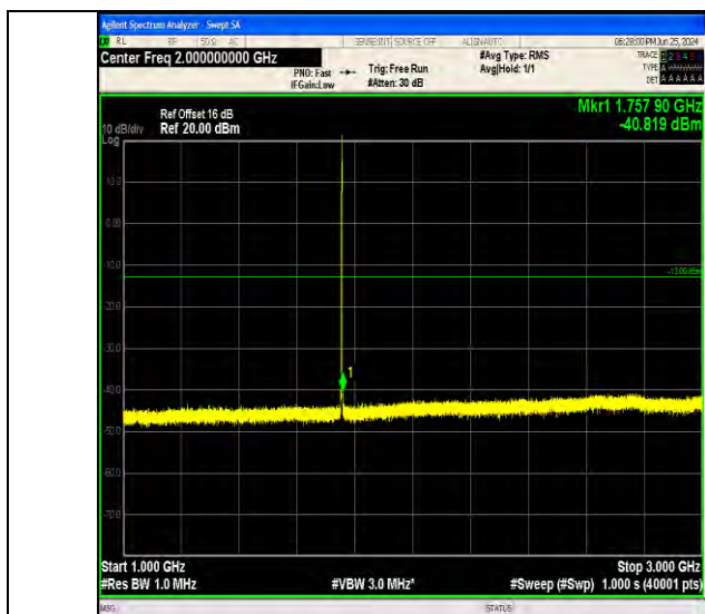
Band4_1.4MHz_64QAM_20393_6RB#0_1000~3000_1000~3000
