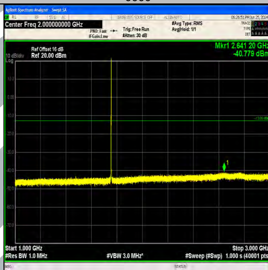
Band4_1.4MHz_64QAM_20393_1RB#5_1000~3000_1000~3000
