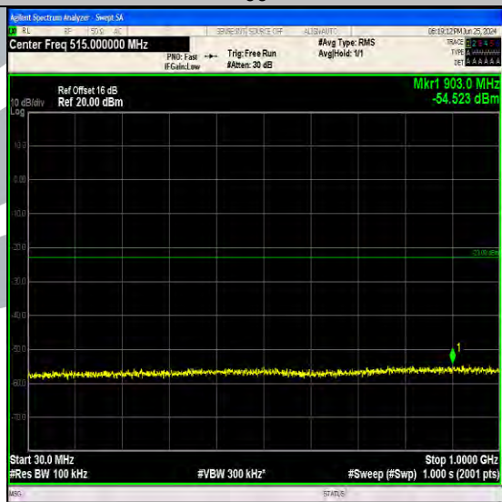
Band4_1.4MHz_16QAM_19957_1RB#5_30~1000_30~1000
