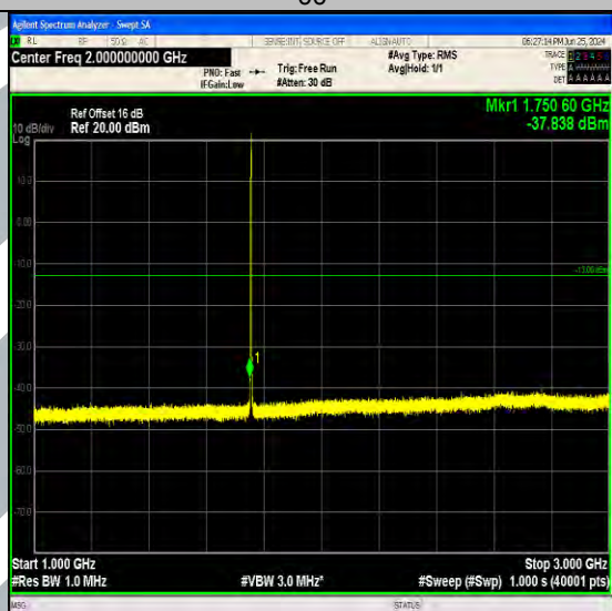
Band4_1.4MHz_QPSK_20393_6RB#0_1000~3000_1000~3000
