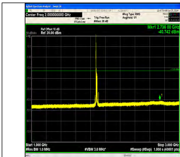
Band2_20MHz_64QAM_18900_1RB#0_1000~3000_1000~3000
