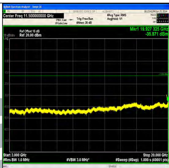
Band4_1.4MHz_QPSK_20175_6RB#0_3000~20000_3000~20000
