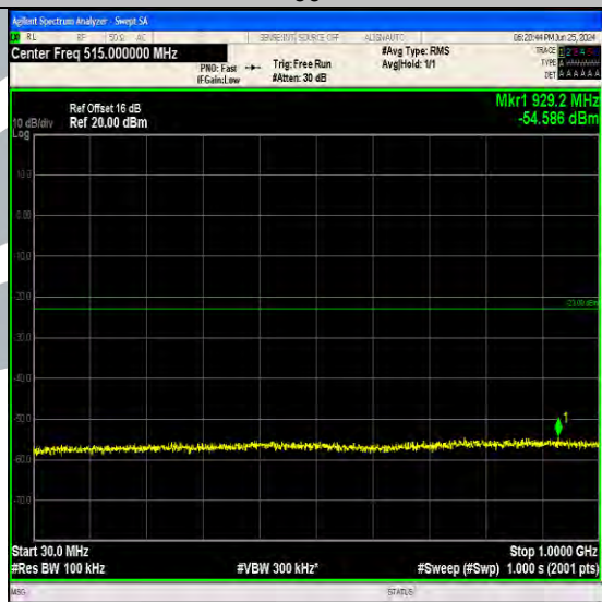
Band4_1.4MHz_64QAM_19957_6RB#0_30~1000_30~1000
