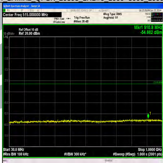
Band4_1.4MHz_QPSK_20393_1RB#5_30~1000_30~1000
