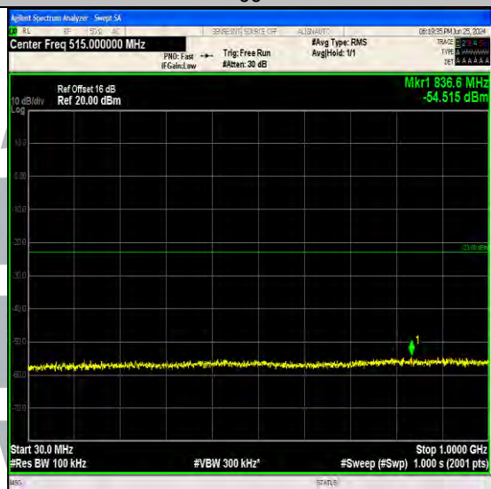
Band4_1.4MHz_64QAM_19957_1RB#5_30~1000_30~1000
