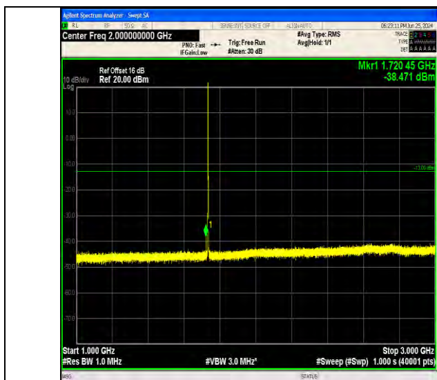
Band4_1.4MHz_64QAM_20175_1RB#5_1000~3000_1000~3000
