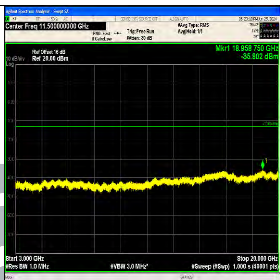
Band4_1.4MHz_64QAM_20175_1RB#5_3000~20000_3000~20000
