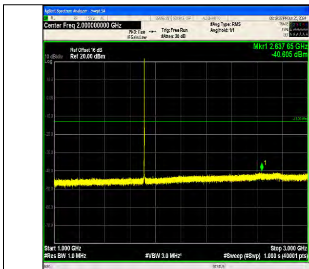
Band4_1.4MHz_64QAM_19957_1RB#0_1000~3000_1000~3000
