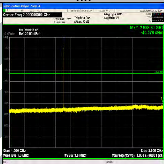
Band4_1.4MHz_64QAM_19957_1RB#5_1000~3000_1000~3000
