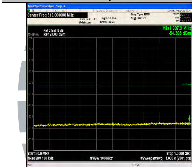
Band2_20MHz_64QAM_18900_1RB#99_30~1000_30~1000
