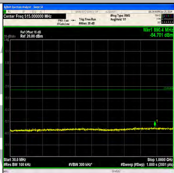
Band4_1.4MHz_QPSK_20393_1RB#0_30~1000_30~1000
