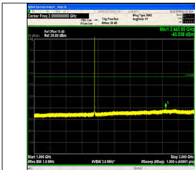
Band4_1.4MHz_QPSK_20393_1RB#5_1000~3000_1000~3000
