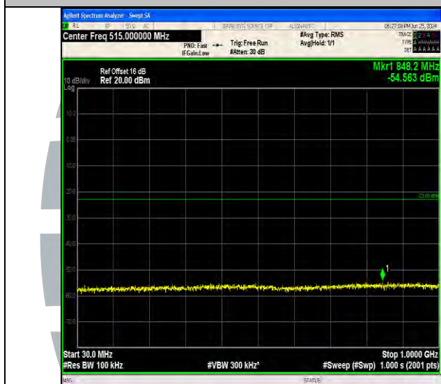
Band4_1.4MHz_QPSK_20393_6RB#0_30~1000_30~1000
