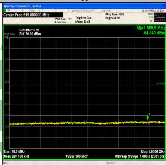
Band4_1.4MHz_64QAM_20175_6RB#0_30~1000_30~1000
