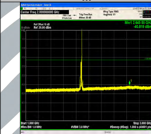
Band2_20MHz_64QAM_18900_1RB#99_1000~3000_1000~3000
