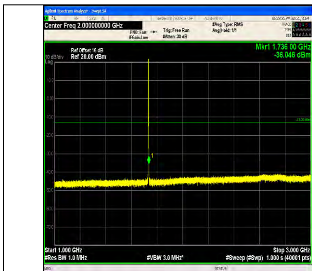
Band4_1.4MHz_QPSK_20175_6RB#0_1000~3000_1000~3000
