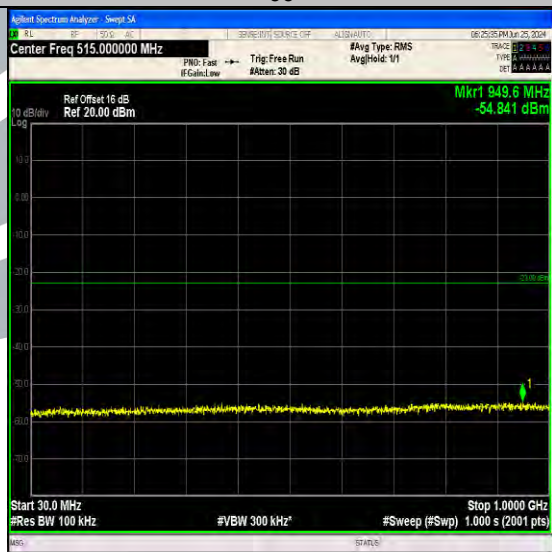
Band4_1.4MHz_64QAM_20393_1RB#0_30~1000_30~1000
