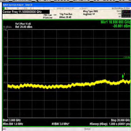
Band4_1.4MHz_QPSK_20393_1RB#0_3000~20000_3000~20000
