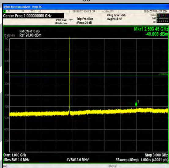
Band4_1.4MHz_QPSK_20393_1RB#0_1000~3000_1000~3000
