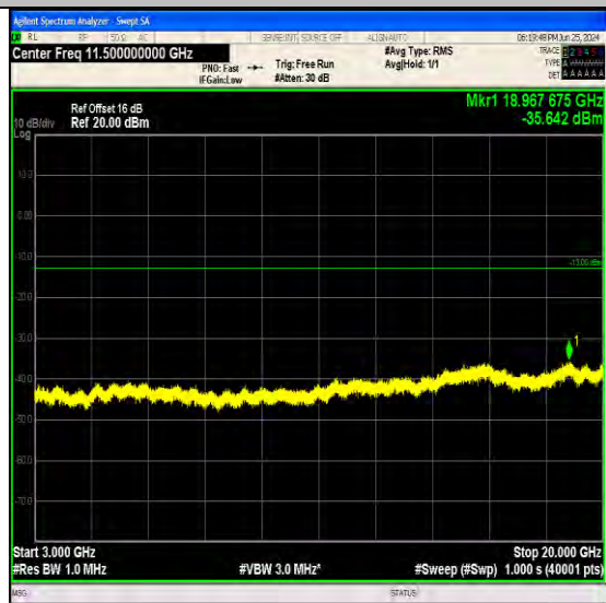
Band4_1.4MHz_64QAM_19957_1RB#5_3000~20000_3000~20000
