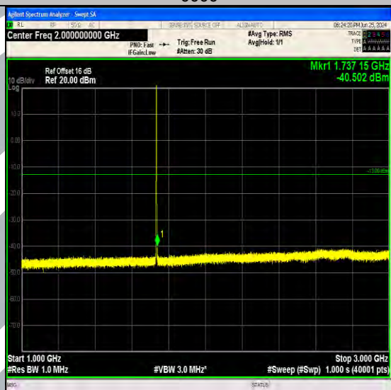
Band4_1.4MHz_64QAM_20175_6RB#0_1000~3000_1000~3000
