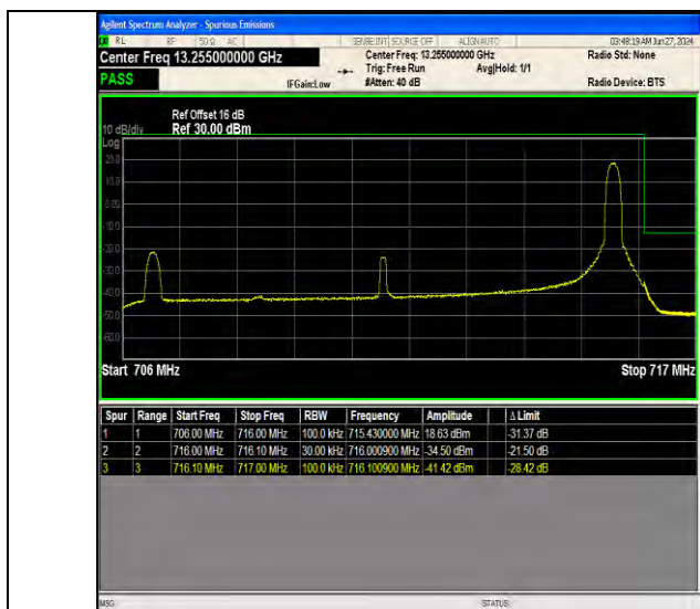
Band17 10MHz 16QAM 23800 1RB#49
