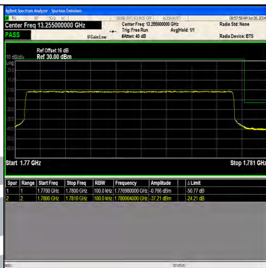
Band66 10MHz 64QAM 132622 50RB#0
