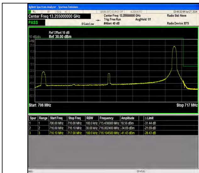
Band17 10MHz 64QAM 23800 1RB#49
