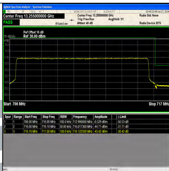
Band17 10MHz 64QAM 23800 50RB#0
