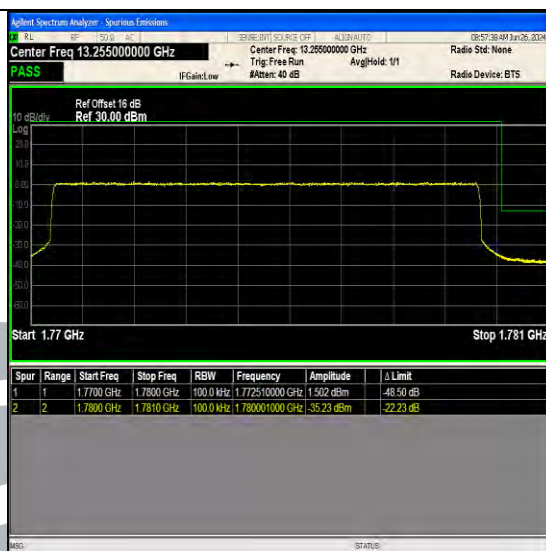
Band66 10MHz QPSK 132622 50RB#0
