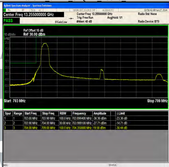
Band17 5MHz 16QAM 23755 1RB#0
