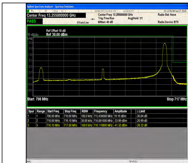
Band12 10MHz 64QAM 23130 1RB#49
