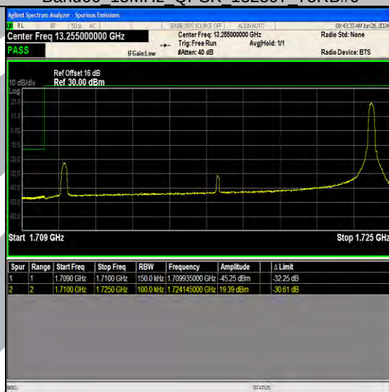
Band66 15MHz 64QAM 132047 1RB#74
