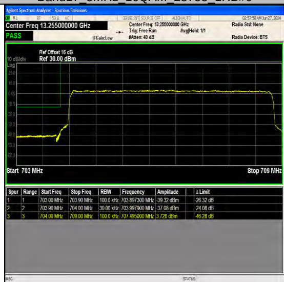
Band17 5MHz 16QAM 23755 25RB#0
