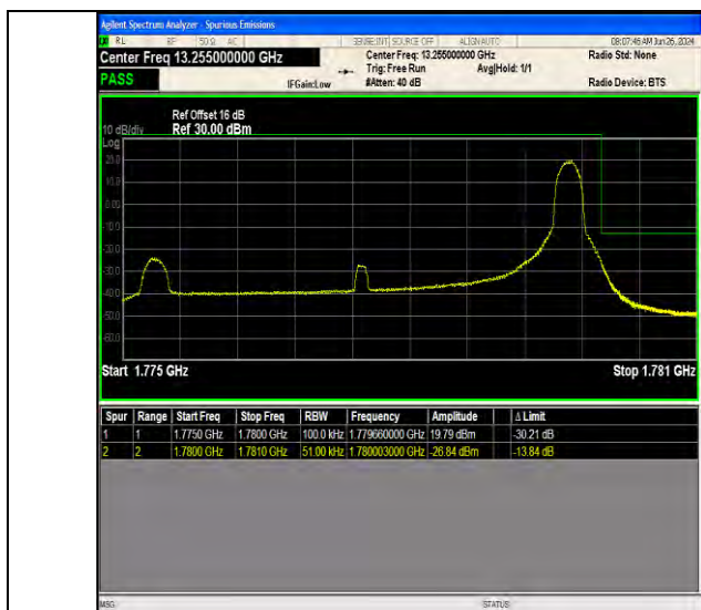
Band66 5MHz 16QAM 132647 1RB#24
