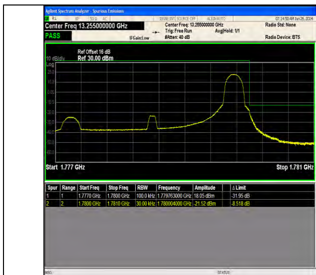
Band66 3MHz 64QAM 132657 1RB#14
