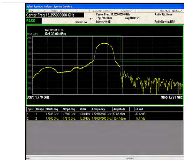
Band66 1.4MHz 64QAM 132665 1RB#5
