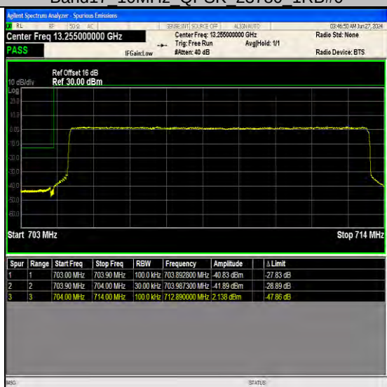
Band17 10MHz QPSK 23780 50RB#0
