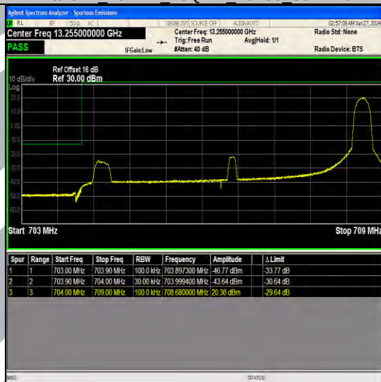
Band17 5MHz QPSK 23755 1RB#24
