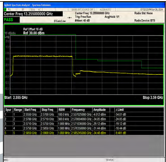
Band7 15MHz 64QAM 21375 75RB#0
