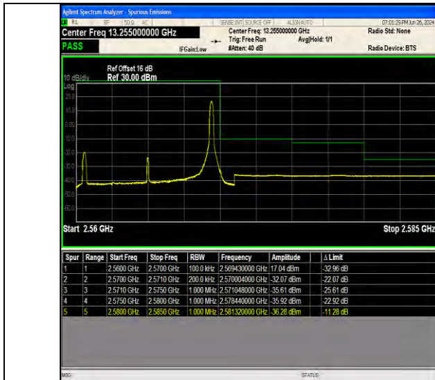
Band7 10MHz 64QAM 21400 1RB#49
