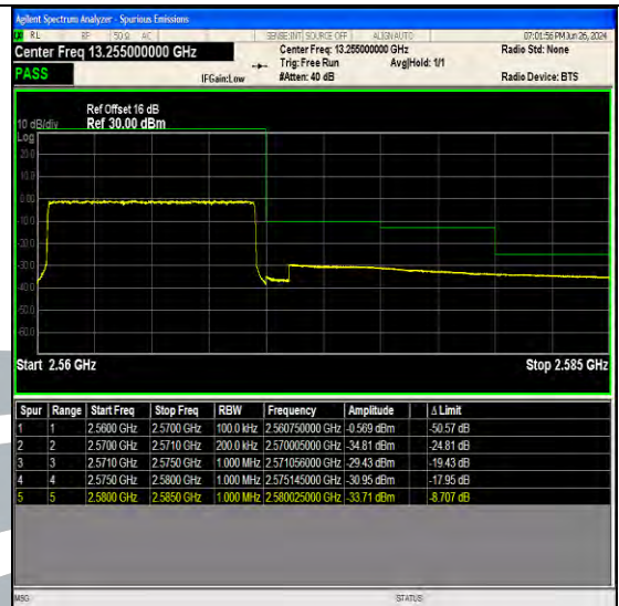
Band7 10MHz 16QAM 21400 50RB#0
