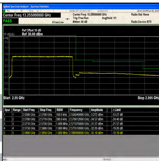
Band7 20MHz 16QAM 21350 100RB#0
