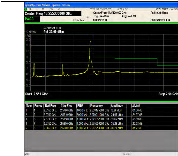
Band7 15MHz 16QAM 21375 1RB#74
