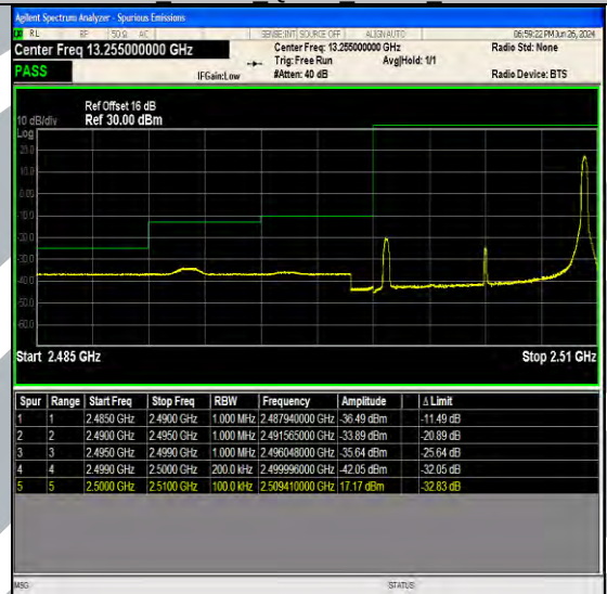
Band7 10MHz 64QAM 20800 1RB#49
