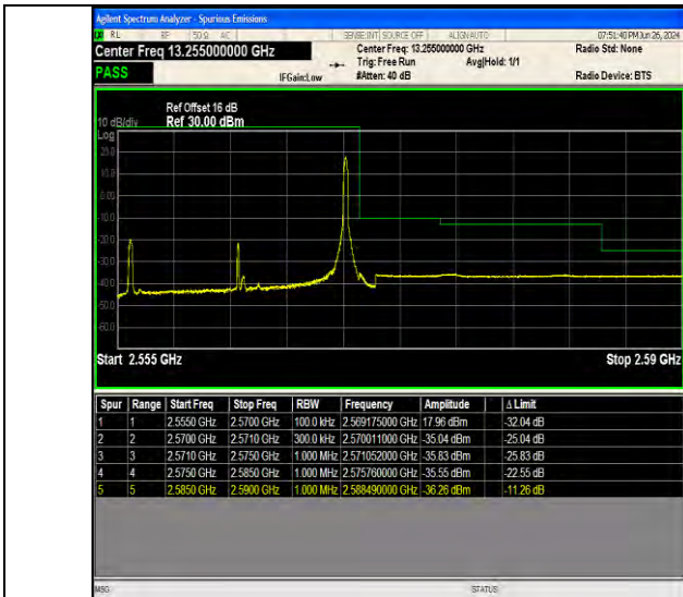
Band7 15MHz 64QAM 21375 1RB#74
