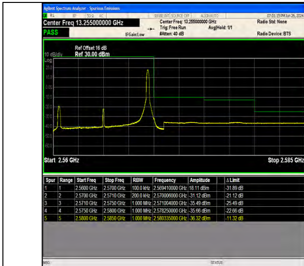
Band7 10MHz 16QAM 21400 1RB#49
