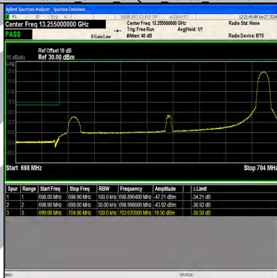
Band12 5MHz 16QAM 23035 1RB#24
