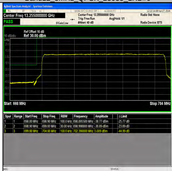
Band12 5MHz QPSK 23035 25RB#0
