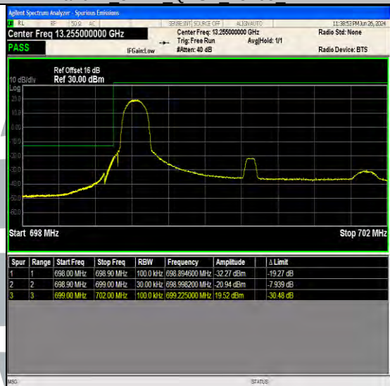
Band12 3MHz 64QAM 23025 1RB#0
