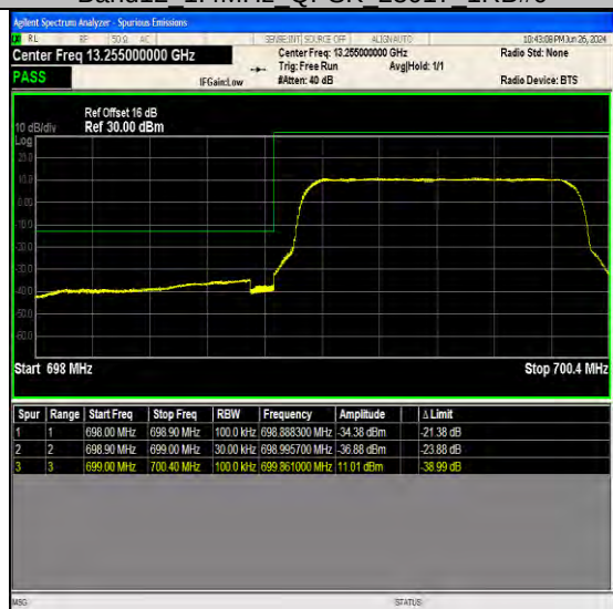
Band12 1.4MHz QPSK 23017 6RB#0
