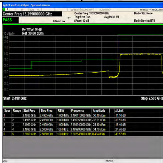
Band7 5MHz 64QAM 20775 25RB#0
