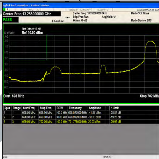
Band12 3MHz 16QAM 23025 1RB#14
