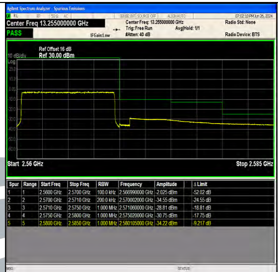
Band7 10MHz 64QAM 21400 50RB#0
