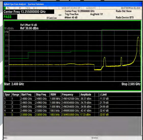
Band7 5MHz 16QAM 20775 1RB#24
