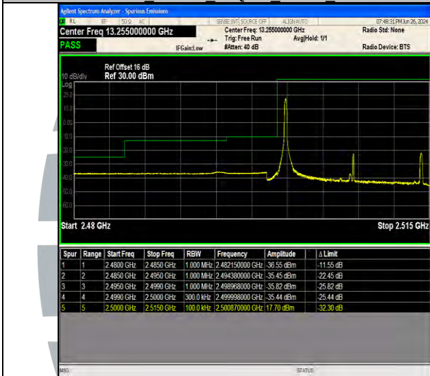
Band7 15MHz 16QAM 20825 1RB#0
