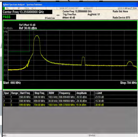
Band12 5MHz 16QAM 23035 1RB#0
