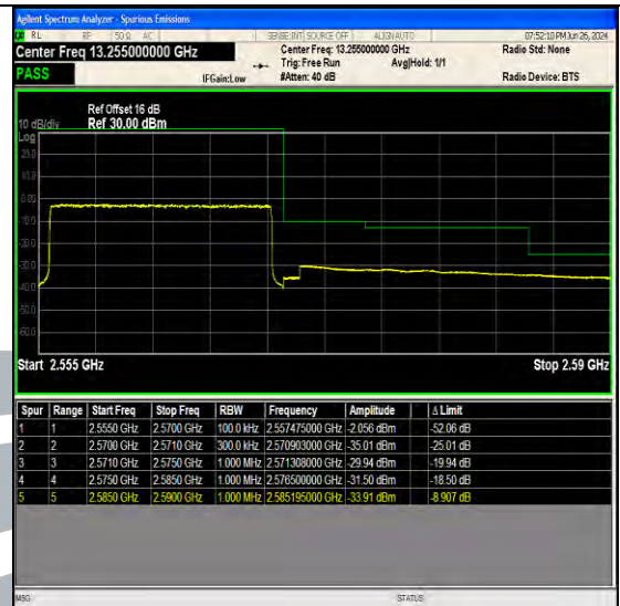
Band7 15MHz 16QAM 21375 75RB#0
