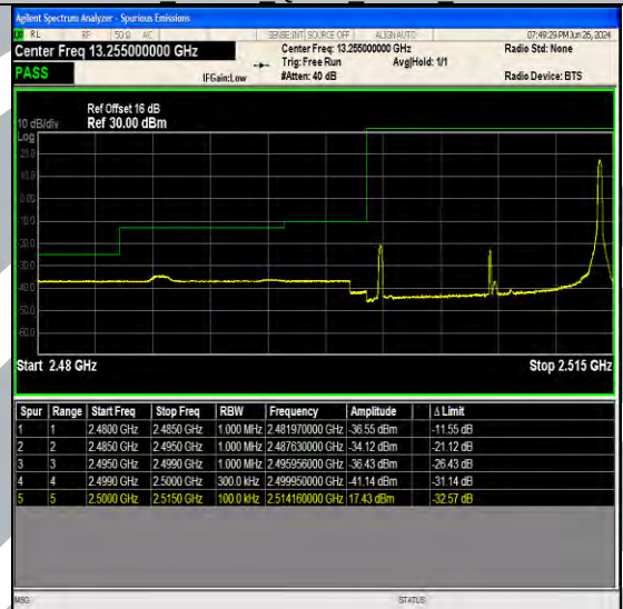
Band7 15MHz 64QAM 20825 1RB#74
