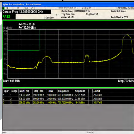
Band12 3MHz 64QAM 23025 1RB#14
