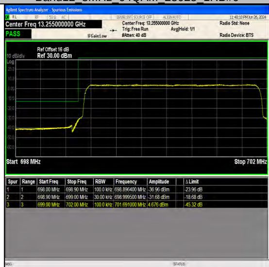
Band12 3MHz 64QAM 23025 15RB#0
