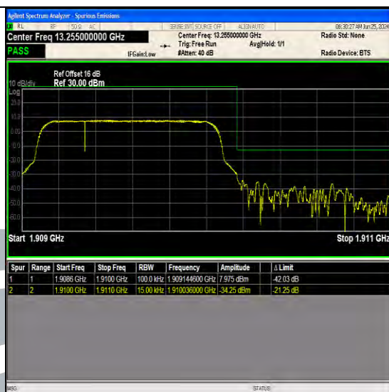
Band2 1.4MHz 64QAM 19193 6RB#0
