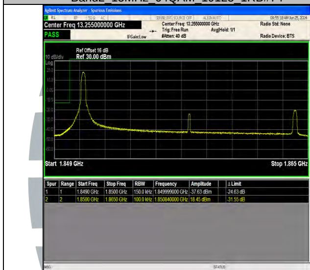
Band2 15MHz 16QAM 18675 1RB#0
