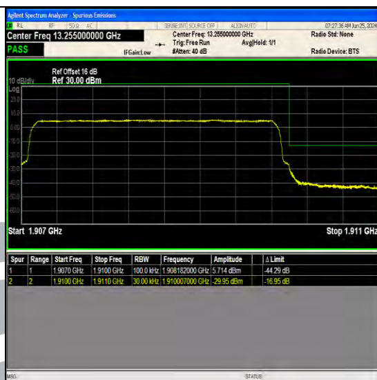
Band2 3MHz 16QAM 19185 15RB#0
