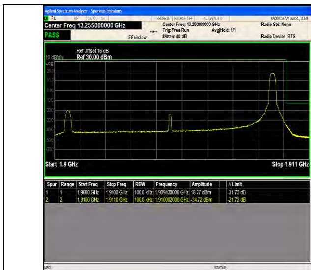
Band2 10MHz 16QAM 19150 1RB#49
