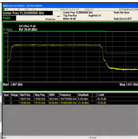
Band2 3MHz 64QAM 19185 15RB#0
