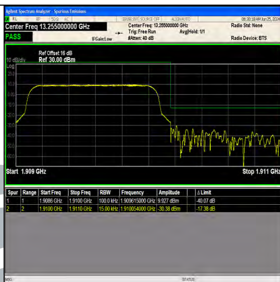
Band2 1.4MHz 16QAM 19193 6RB#0
