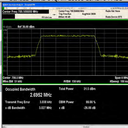
Band12-3MHz-16QAM-23025-15RB#0-PASS
