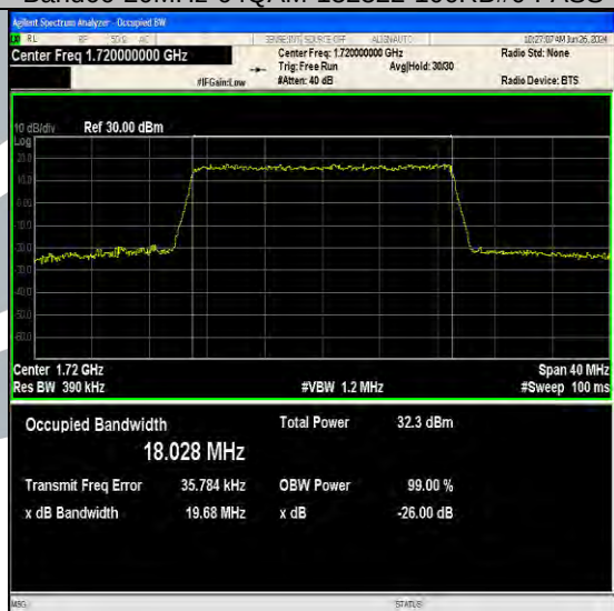
Band66-20MHz-16QAM-132072-100RB#0-PASS
