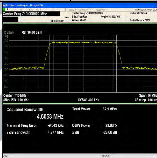
Band17-5MHz-QPSK-23790-25RB#0-PASS
