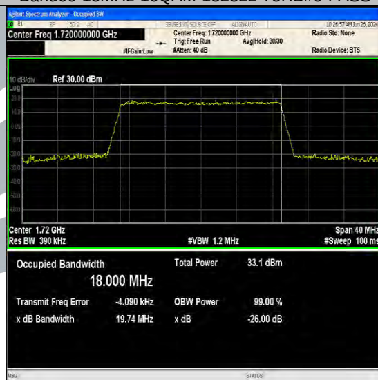
Band66-20MHz-QPSK-132072-100RB#0-PASS
