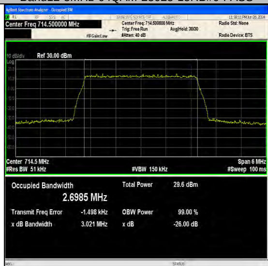
Band12-3MHz-64QAM-23165-15RB#0-PASS
