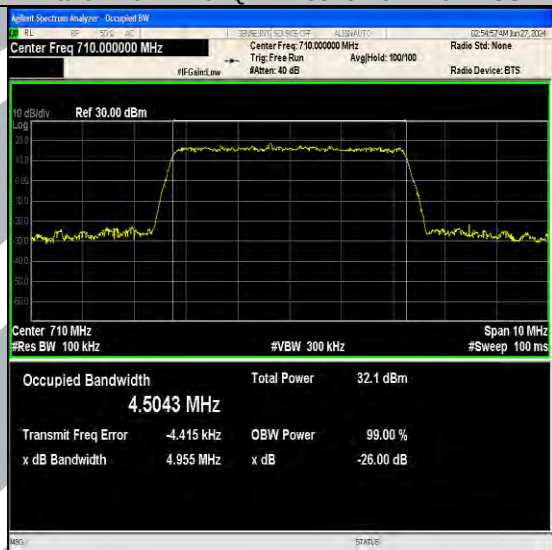
Band17-5MHz-16QAM-23790-25RB#0-PASS
