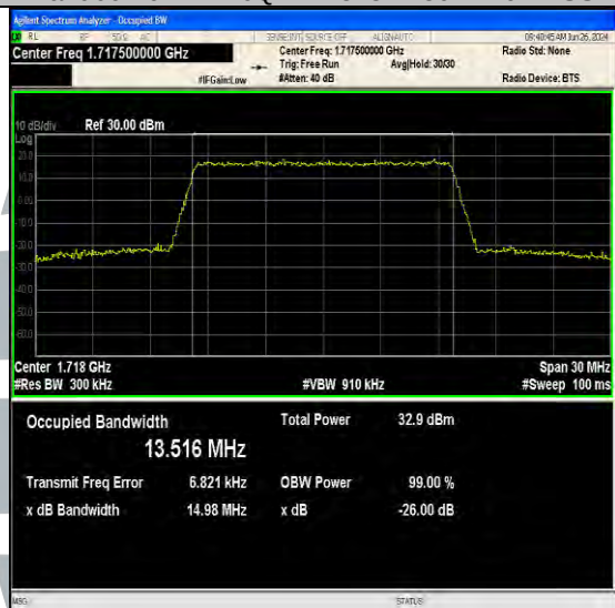
Band66-15MHz-QPSK-132047-75RB#0-PASS
