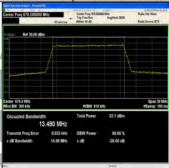
Band71-15MHz-16QAM-133197-75RB#0-PASS
