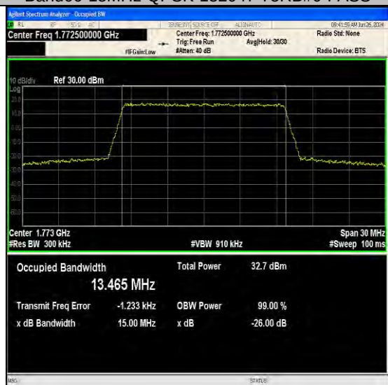
Band66-15MHz-QPSK-132597-75RB#0-PASS
