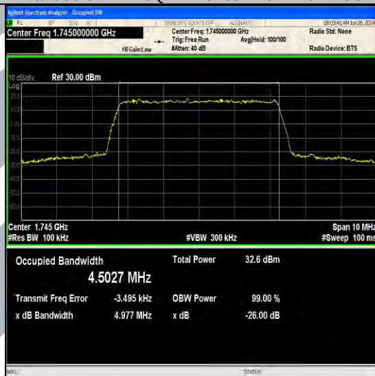
Band66-5MHz-QPSK-132322-25RB#0-PASS
