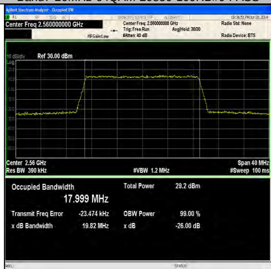
Band7-20MHz-64QAM-21350-100RB#0-PASS
