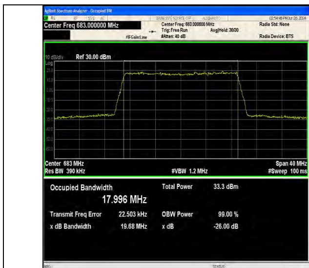
Band71-20MHz-QPSK-133322-100RB#0-PASS
