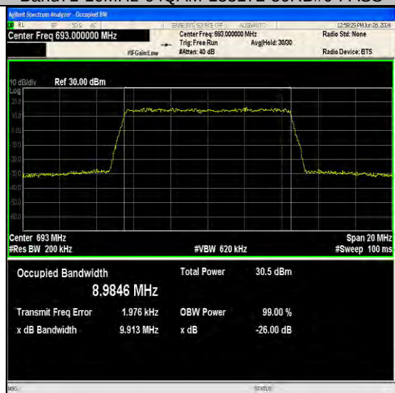
Band71-10MHz-64QAM-133422-50RB#0-PASS
