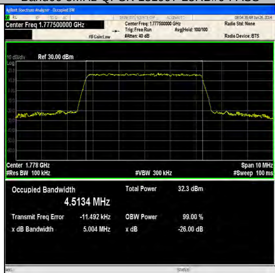
Band66-5MHz-QPSK-132647-25RB#0-PASS
