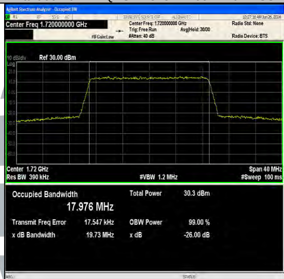
Band66-20MHz-64QAM-132072-100RB#0-PASS
