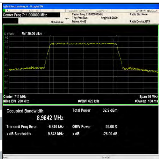
Band17-10MHz-QPSK-23800-50RB#0-PASS
