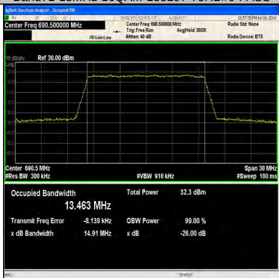
Band71-15MHz-16QAM-133397-75RB#0-PASS
