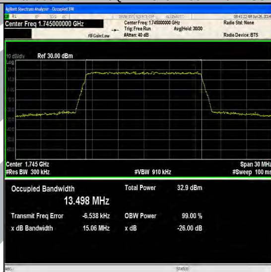
Band66-15MHz-QPSK-132322-75RB#0-PASS
