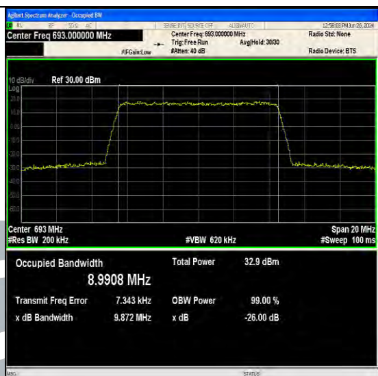
Band71-10MHz-QPSK-133422-50RB#0-PASS
