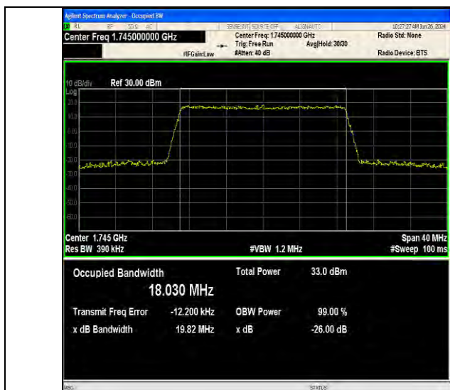
Band66-20MHz-QPSK-132322-100RB#0-PASS
