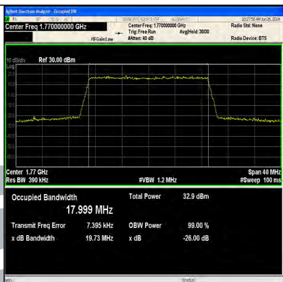
Band66-20MHz-QPSK-132572-100RB#0-PASS
