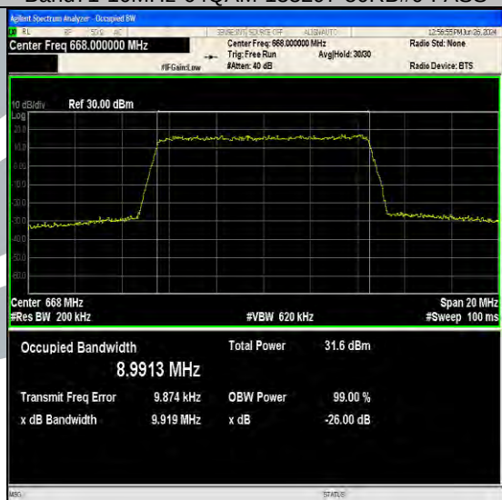
Band71-10MHz-16QAM-133172-50RB#0-PASS
