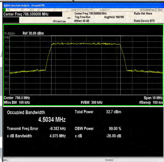
Band17-5MHz-QPSK-23755-25RB#0-PASS
