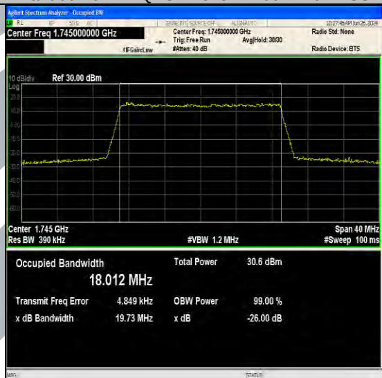
Band66-20MHz-64QAM-132322-100RB#0-PASS
