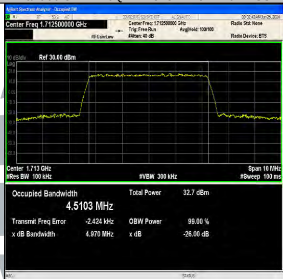
Band66-5MHz-QPSK-131997-25RB#0-PASS
