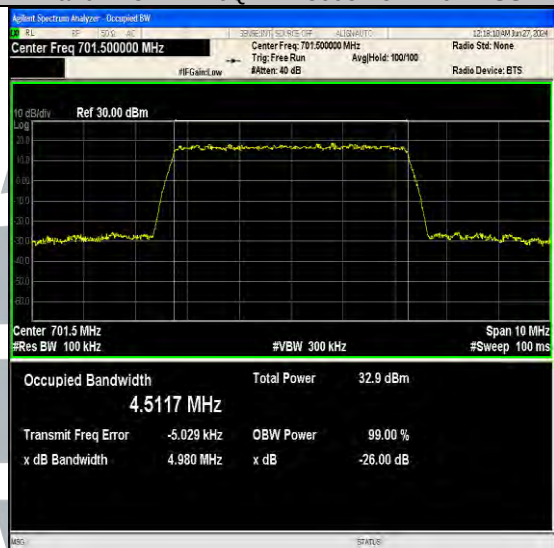
Band12-5MHz-QPSK-23035-25RB#0-PASS
