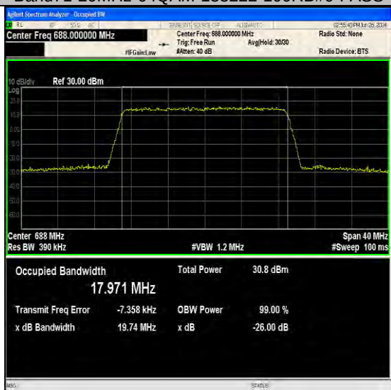
Band71-20MHz-64QAM-133372-100RB#0-PASS
