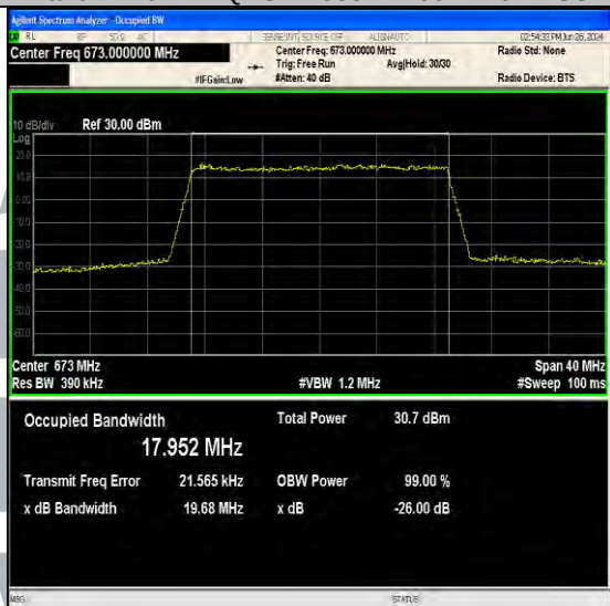
Band71-20MHz-64QAM-133222-100RB#0-PASS
