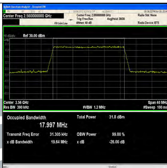
Band7-20MHz-QPSK-21350-100RB#0-PASS
