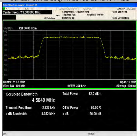
Band17-5MHz-16QAM-23825-25RB#0-PASS
