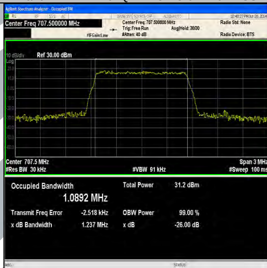
Band12-1.4MHz-16QAM-23095-6RB#0-PASS
