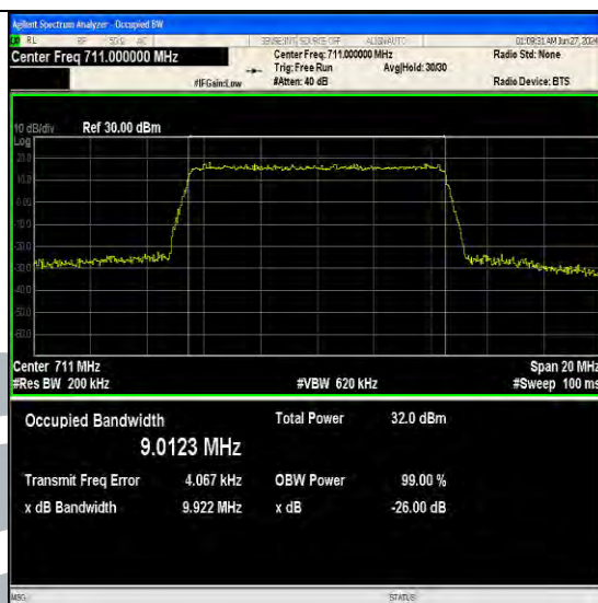
Band12-10MHz-16QAM-23130-50RB#0-PASS
