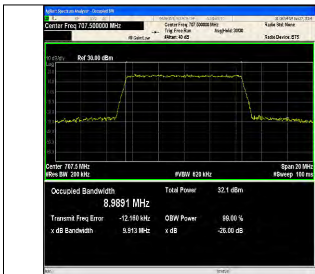
Band12-10MHz-16QAM-23095-50RB#0-PASS
