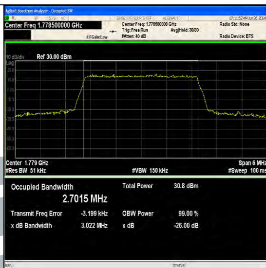
Band66-3MHz-16QAM-132657-15RB#0-PASS
