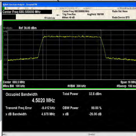
Band71-5MHz-QPSK-133297-25RB#0-PASS
