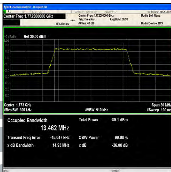
Band66-15MHz-64QAM-132597-75RB#0-PASS
