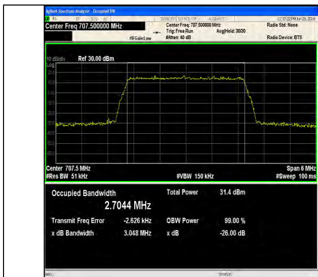
Band12-3MHz-16QAM-23095-15RB#0-PASS
