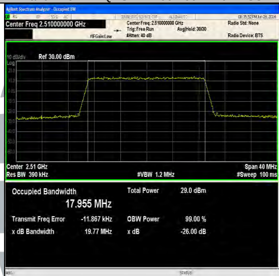
Band7-20MHz-64QAM-20850-100RB#0-PASS
