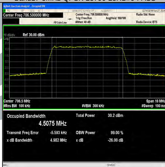
Band17-5MHz-64QAM-23755-25RB#0-PASS
