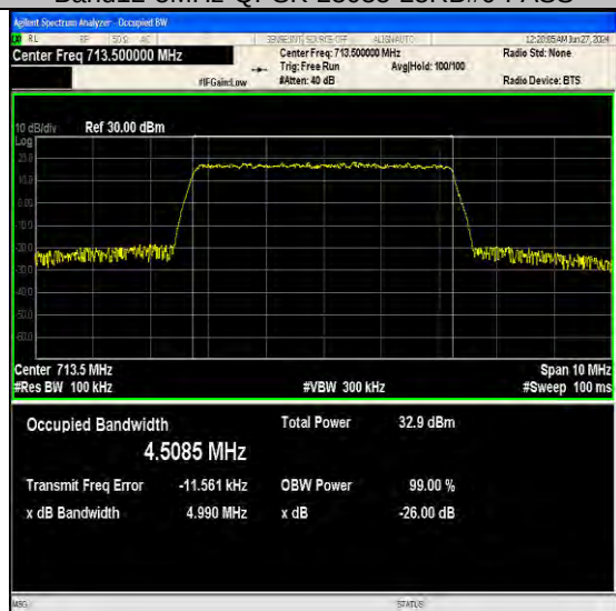
Band12-5MHz-QPSK-23155-25RB#0-PASS
