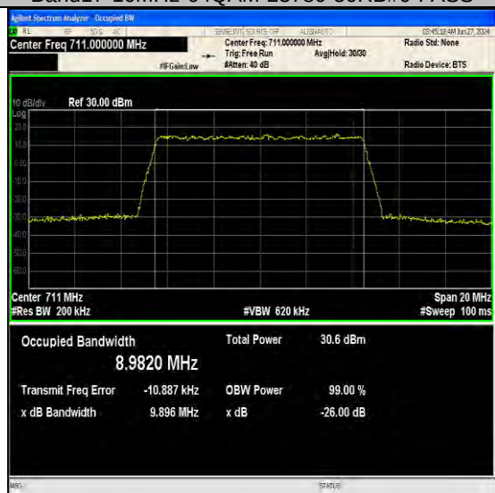
Band17-10MHz-64QAM-23780-50RB#0-PASS
