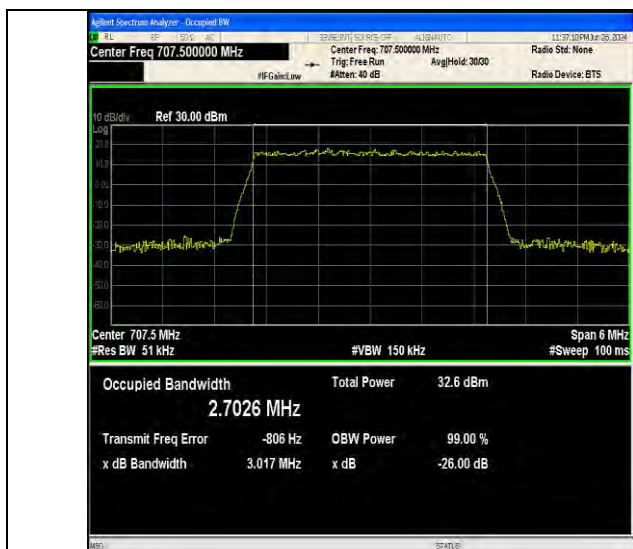
Band12-3MHz-QPSK-23095-15RB#0-PASS
