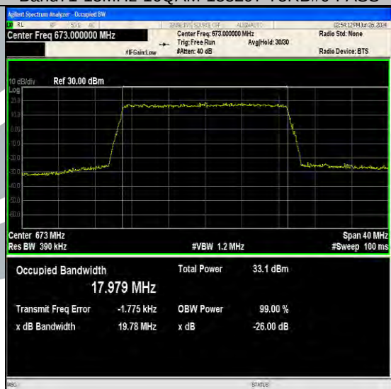
Band71-20MHz-QPSK-133222-100RB#0-PASS
