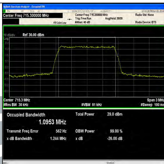
Band12-1.4MHz-64QAM-23173-6RB#0-PASS
