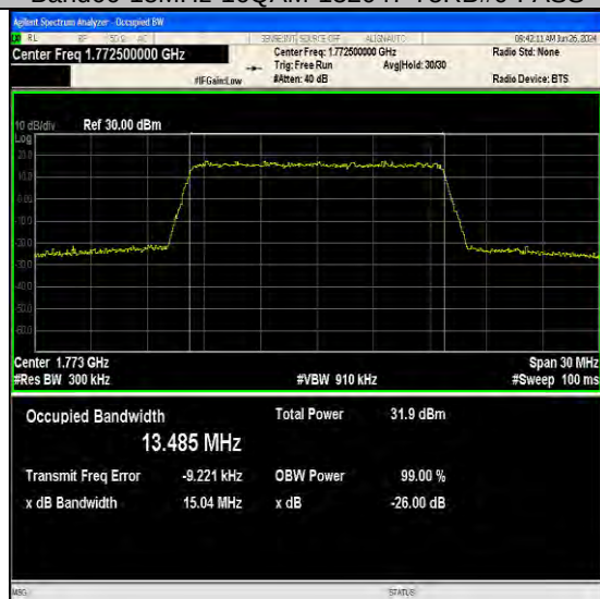
Band66-15MHz-16QAM-132597-75RB#0-PASS
