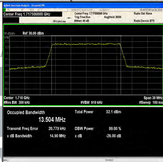
Band66-15MHz-16QAM-132047-75RB#0-PASS
