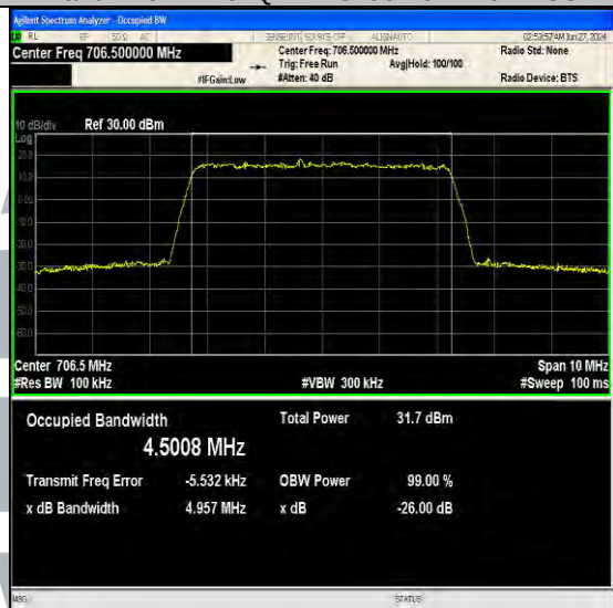
Band17-5MHz-16QAM-23755-25RB#0-PASS
