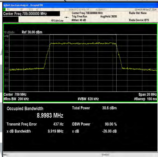
Band17-10MHz-QPSK-23790-50RB#0-PASS
