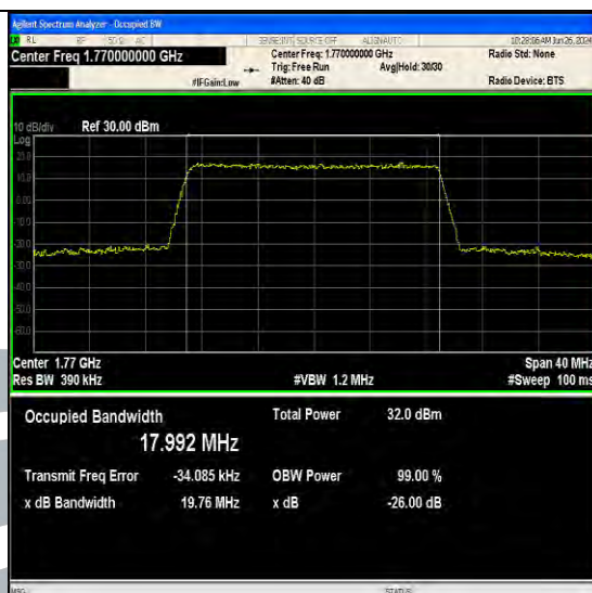
Band66-20MHz-16QAM-132572-100RB#0-PASS
