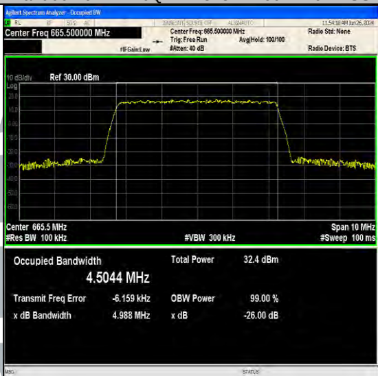
Band71-5MHz-QPSK-133147-25RB#0-PASS
