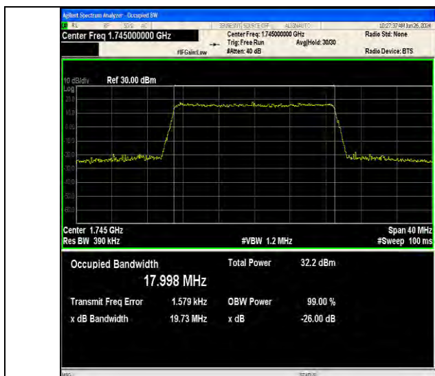
Band66-20MHz-16QAM-132322-100RB#0-PASS
