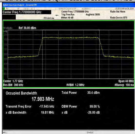
Band66-20MHz-64QAM-132572-100RB#0-PASS
