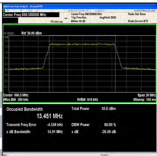
Band71-15MHz-64QAM-133397-75RB#0-PASS
