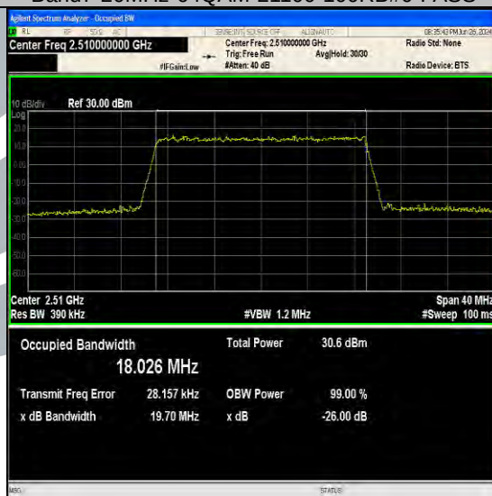
Band7-20MHz-16QAM-20850-100RB#0-PASS
