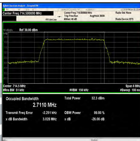
Band12-3MHz-QPSK-23165-15RB#0-PASS
