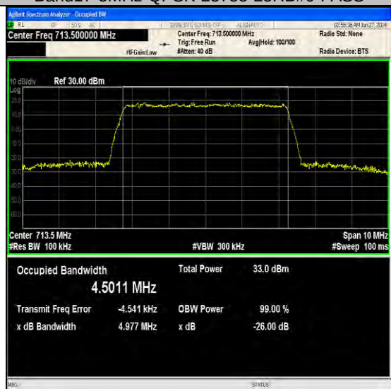
Band17-5MHz-QPSK-23825-25RB#0-PASS
