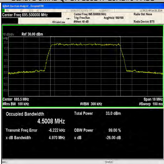
Band71-5MHz-QPSK-133447-25RB#0-PASS
