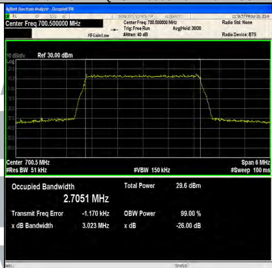
Band12-3MHz-64QAM-23025-15RB#0-PASS
