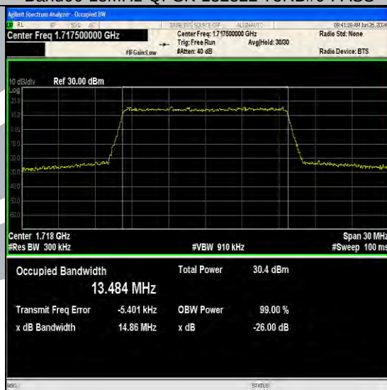
Band66-15MHz-64QAM-132047-75RB#0-PASS
