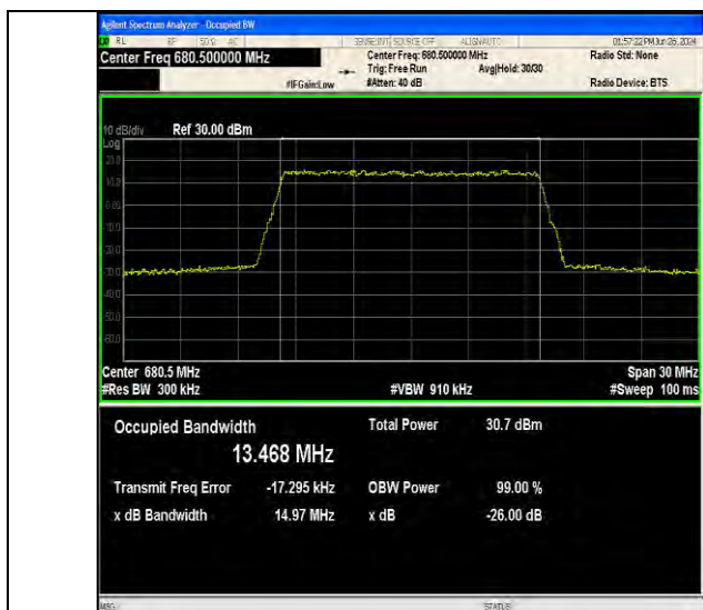
Band71-15MHz-64QAM-133297-75RB#0-PASS
