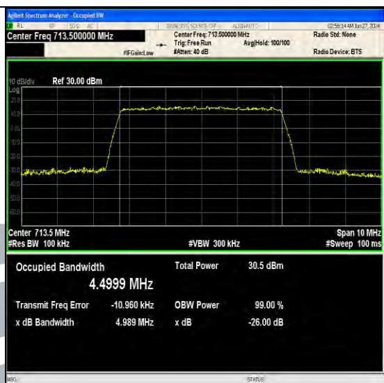
Band17-5MHz-64QAM-23825-25RB#0-PASS
