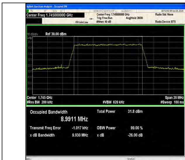
Band66-10MHz-16QAM-132322-50RB#0-PASS
