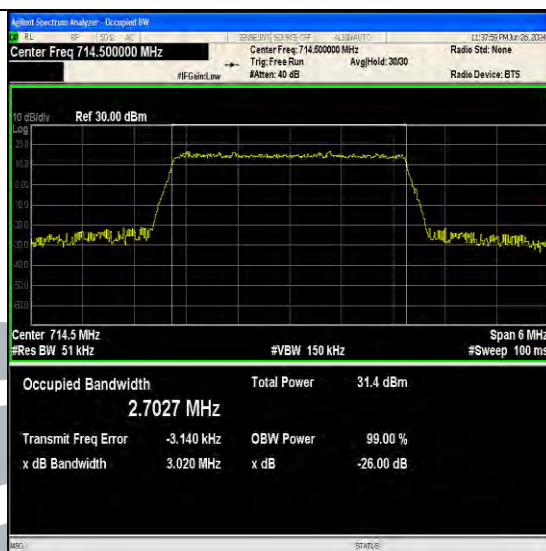
Band12-3MHz-16QAM-23165-15RB#0-PASS
