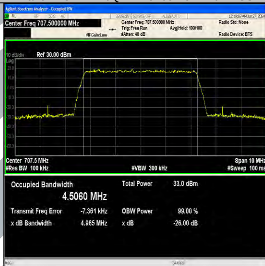
Band12-5MHz-QPSK-23095-25RB#0-PASS
