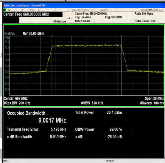
Band71-10MHz-64QAM-133172-50RB#0-PASS
