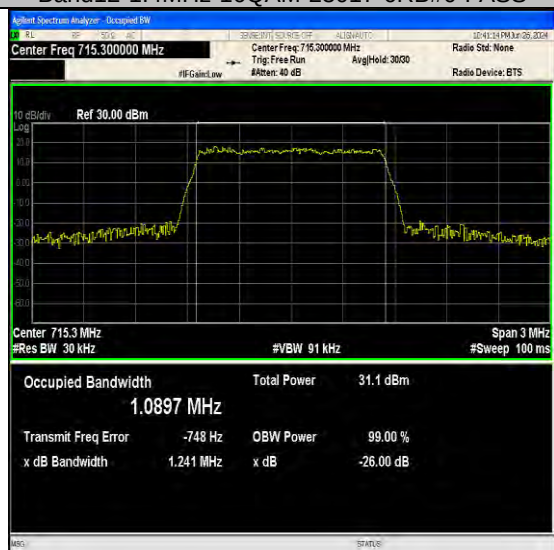
Band12-1.4MHz-16QAM-23173-6RB#0-PASS
