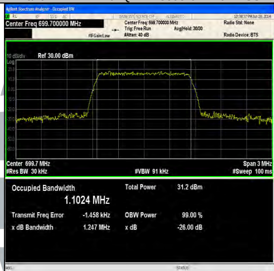
Band12-1.4MHz-16QAM-23017-6RB#0-PASS
