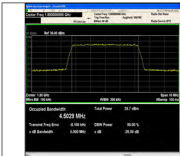
Band2-5MHz-64QAM-18900-25RB#0-PASS
