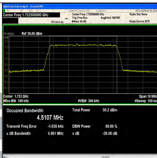
Band4-5MHz-64QAM-20375-25RB#0-PASS
