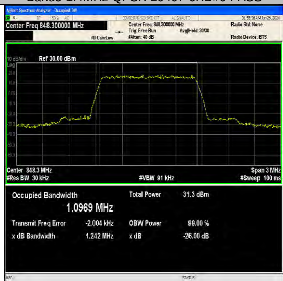
Band5-1.4MHz-QPSK-20643-6RB#0-PASS
