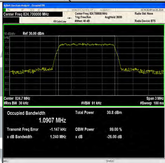
Band5-1.4MHz-QPSK-20407-6RB#0-PASS
