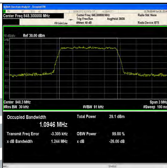
Band5-1.4MHz-64QAM-20643-6RB#0-PASS
