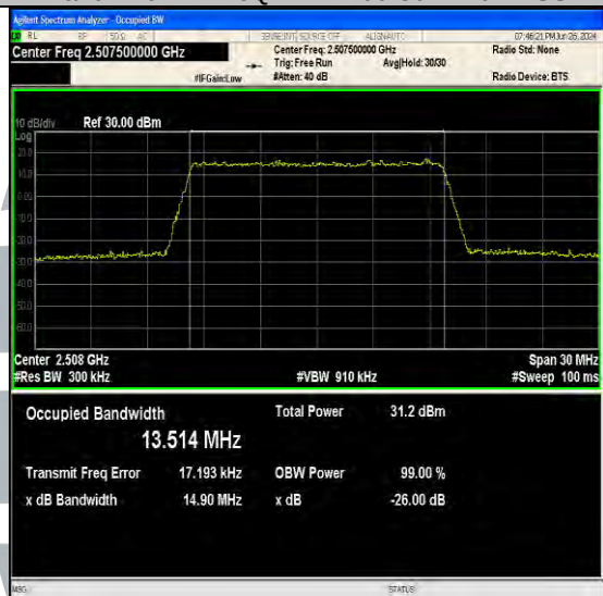
Band7-15MHz-QPSK-20825-75RB#0-PASS
