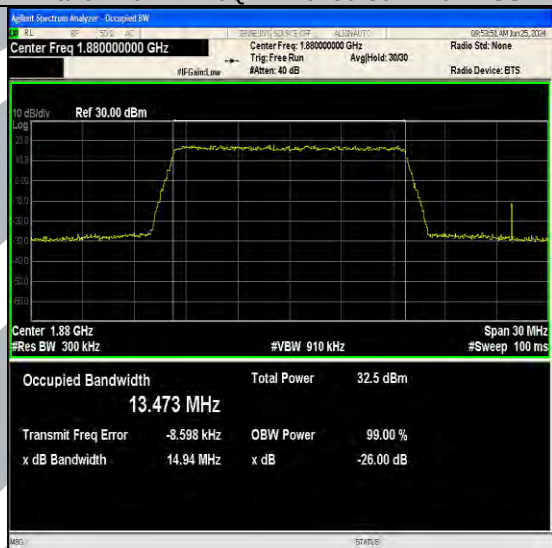
Band2-15MHz-QPSK-18900-75RB#0-PASS
