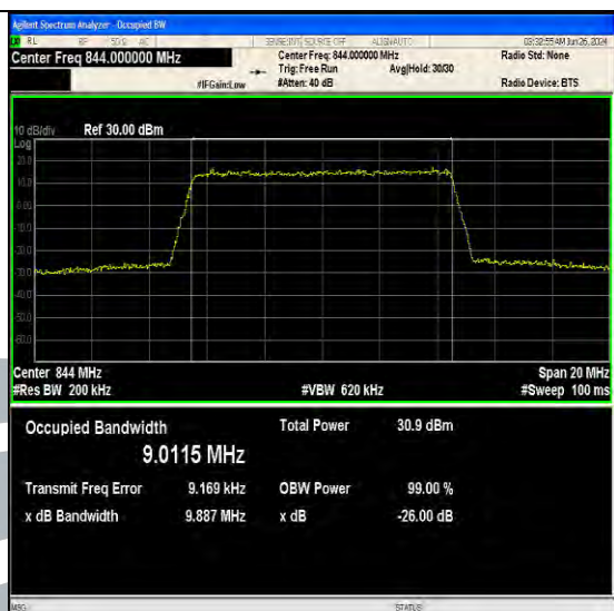
Band5-10MHz-16QAM-20600-50RB#0-PASS
