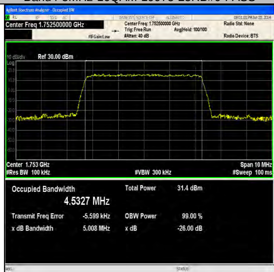
Band4-5MHz-16QAM-20375-25RB#0-PASS
