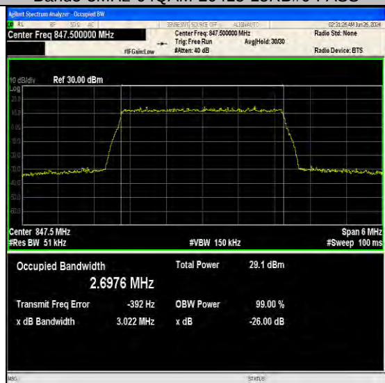
Band5-3MHz-64QAM-20635-15RB#0-PASS
