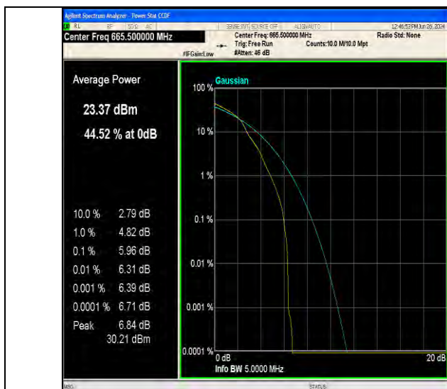
Band71-5MHz-16QAM-133147-1RB#0-PASS
