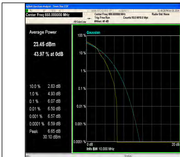
Band71-10MHz-16QAM-133172-1RB#0-PASS
