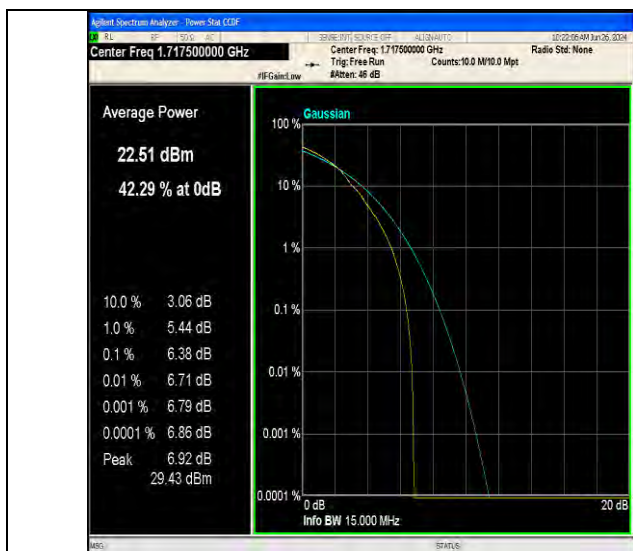
Band66-15MHz-64QAM-132047-1RB#0-PASS
