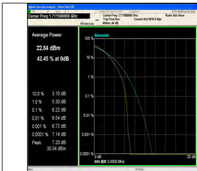
Band66-3MHz-64QAM-131987-1RB#0-PASS
