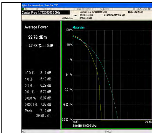
Band66-5MHz-64QAM-131997-1RB#0-PASS
