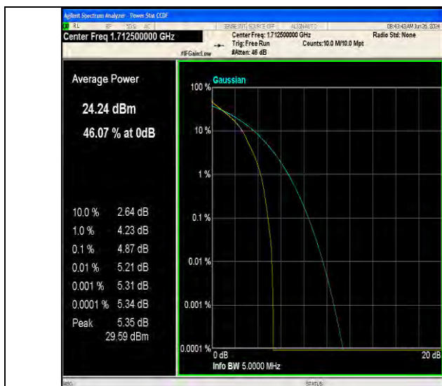
Band66-5MHz-QPSK-131997-1RB#0-PASS
