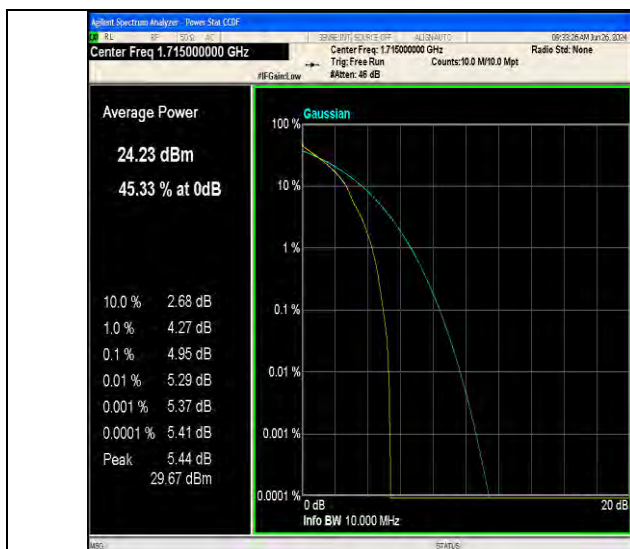
Band66-10MHz-QPSK-132022-1RB#0-PASS
