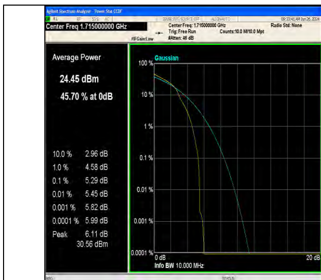
Band66-10MHz-16QAM-132022-1RB#0-PASS
