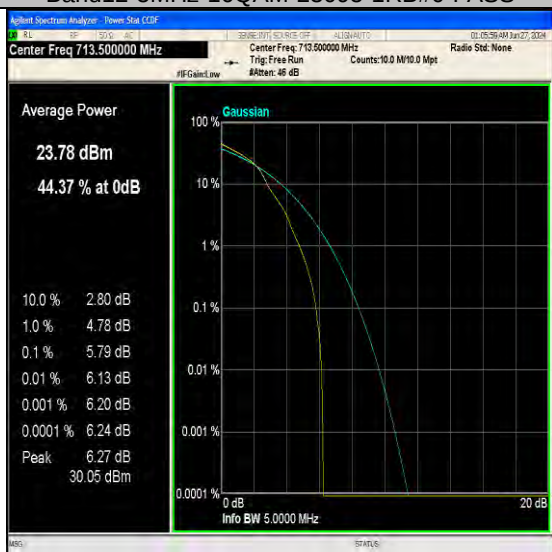
Band12-5MHz-16QAM-23155-1RB#0-PASS
