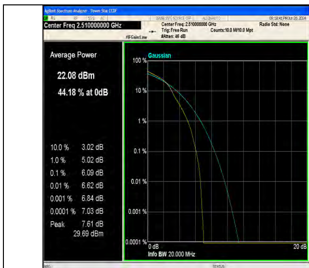
Band7-20MHz-16QAM-20850-1RB#0-PASS
