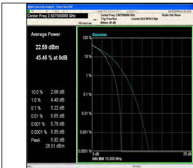
Band7-15MHz-QPSK-20825-1RB#0-PASS
