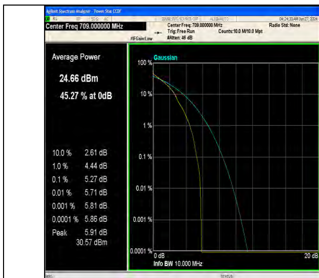
Band17-10MHz-QPSK-23780-1RB#0-PASS
