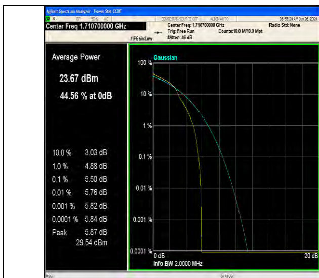
Band66-1.4MHz-16QAM-131979-1RB#0-PASS
