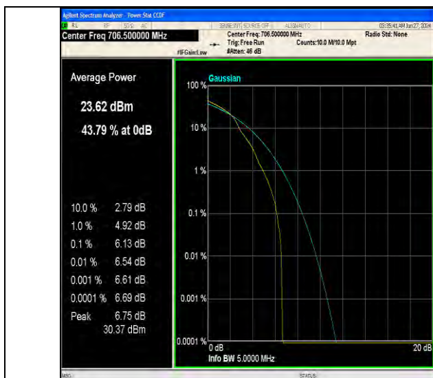
Band17-5MHz-16QAM-23755-1RB#0-PASS
