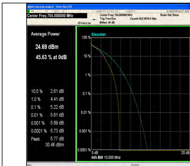
Band12-10MHz-QPSK-23060-1RB#0-PASS
