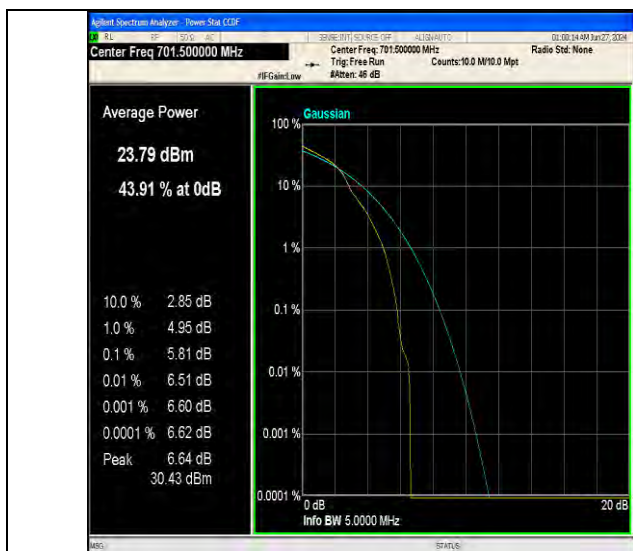
Band12-5MHz-16QAM-23035-1RB#0-PASS
