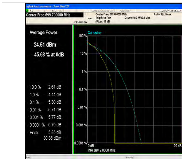
Band12-1.4MHz-QPSK-23017-1RB#0-PASS
