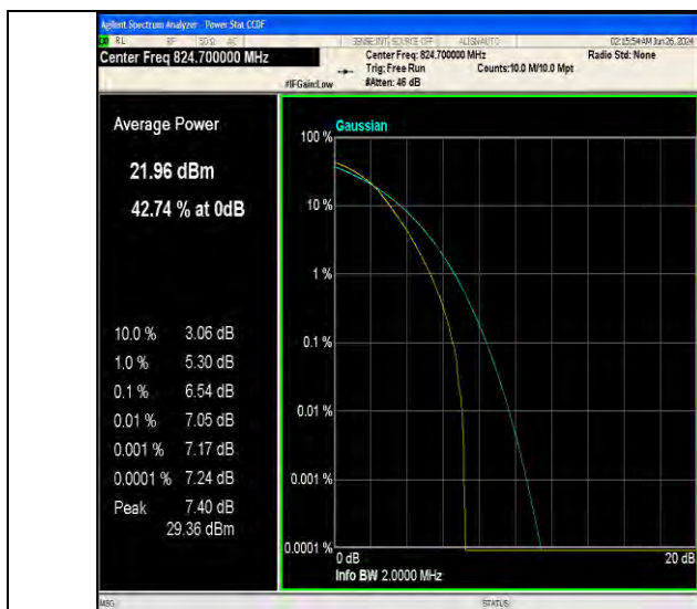
Band5-1.4MHz-64QAM-20407-1RB#0-PASS
