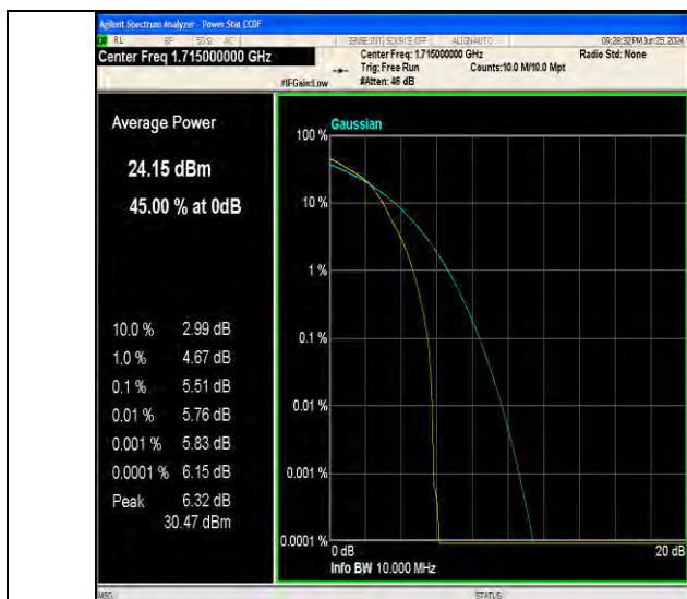
Band4-10MHz-16QAM-20000-1RB#0-PASS
