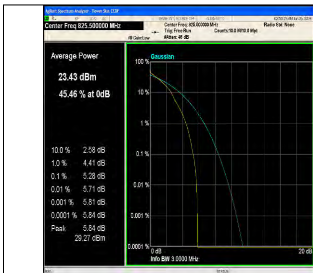
Band5-3MHz-QPSK-20415-1RB#0-PASS
