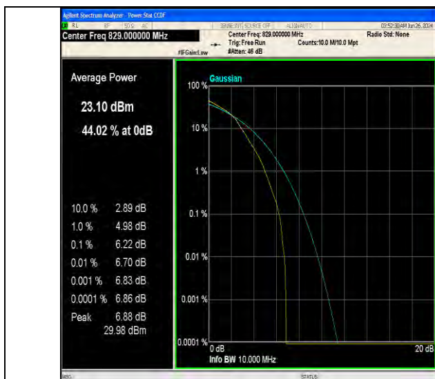
Band5-10MHz-16QAM-20450-1RB#0-PASS
