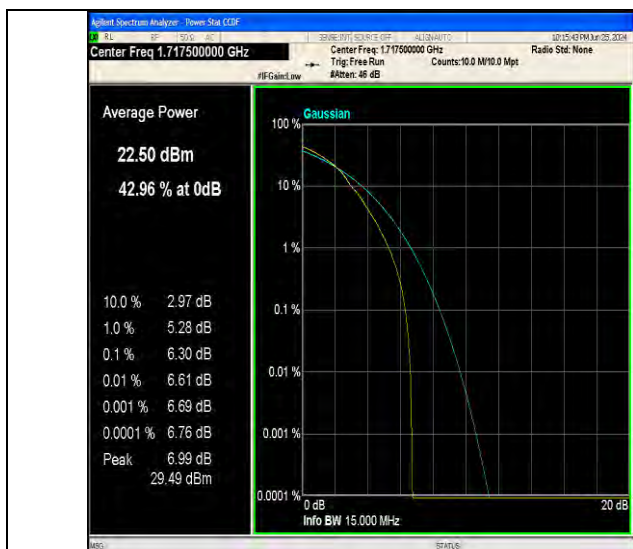
Band4-15MHz-64QAM-20025-1RB#0-PASS
