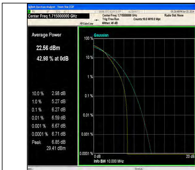
Band4-10MHz-64QAM-20000-1RB#0-PASS
