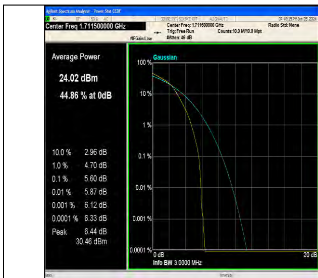
Band4-3MHz-16QAM-19965-1RB#0-PASS
