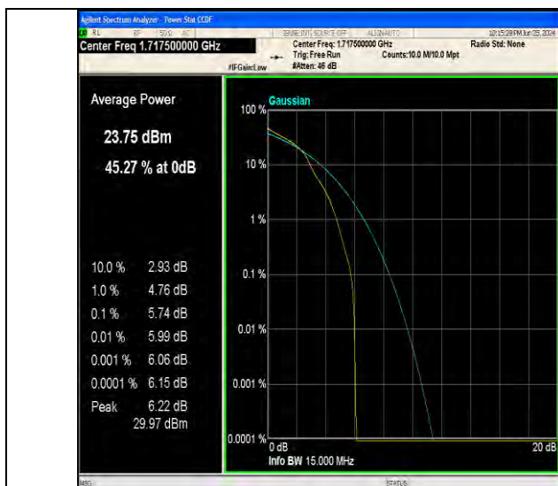
Band4-15MHz-16QAM-20025-1RB#0-PASS
