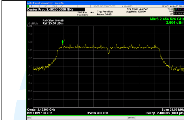
In-Band Reference Level IEEE 802.11g Channel 11 20MHz Antenna 0
