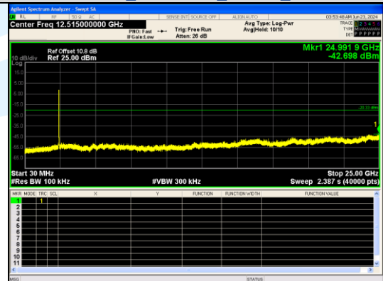
30.0 MHz - 25000.0 MHz IEEE 802.11n Channel 6 20MHz Antenna 0
