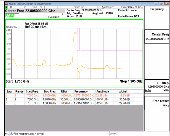
n66 25M DFT-s-OFDM BPSK Edge_1RB_Right High
