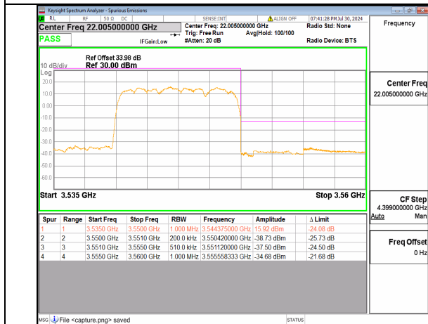
n77(3450-3550MHz) 10M DFT-s-OFDM BPSK Outer_Full High
