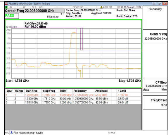
n66 15M DFT-s-OFDM BPSK Edge_1RB_Right High
