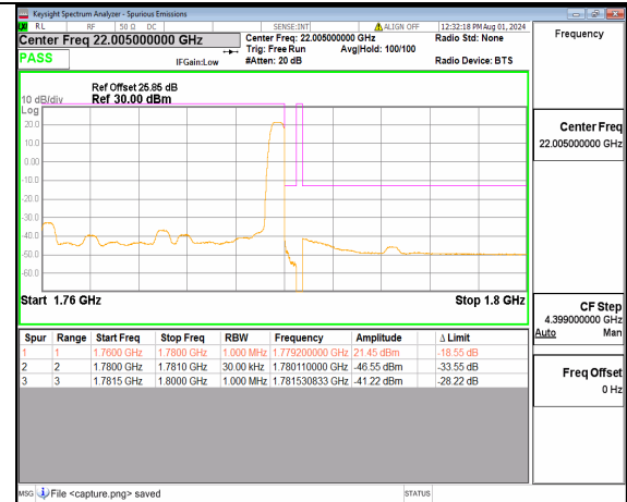
n66 20M DFT-s-OFDM QPSK Edge_1RB_Right High
