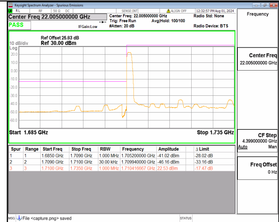
n66 25M DFT-s-OFDM BPSK Edge_1RB_Left Low
