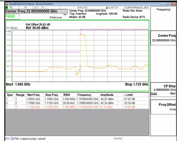
n66 15M DFT-s-OFDM QPSK Edge_1RB_Left Low
