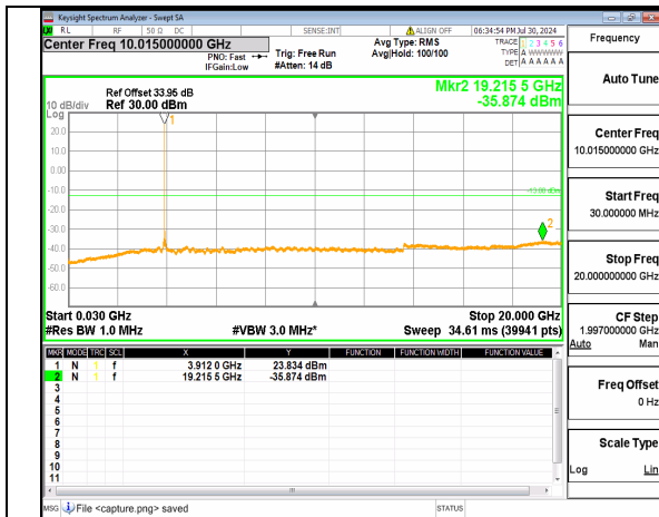
n77(3700-3980MHz) (30MHz-20GHz) 70M DFT-s-OFDM QPSK Inner_1RB_Left High
