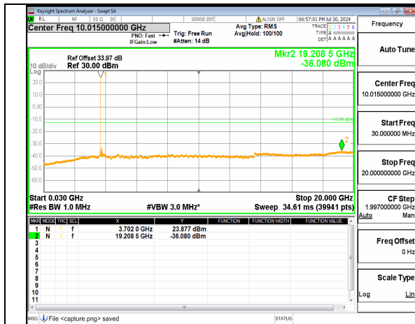
n77(3700-3980MHz) (30MHz-20GHz) 90M DFT-s-OFDM QPSK Inner_1RB_Left Low
