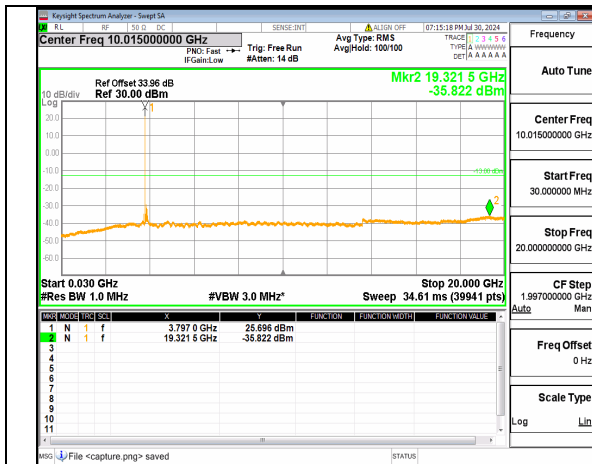
n77(3700-3980MHz) (30MHz-20GHz) 90M DFT-s-OFDM QPSK Inner_1RB_Left Mid
