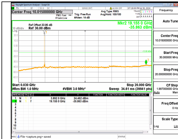
n77(3700-3980MHz) (30MHz-20GHz) 90M DFT-s-OFDM BPSK Inner_1RB_Left High
