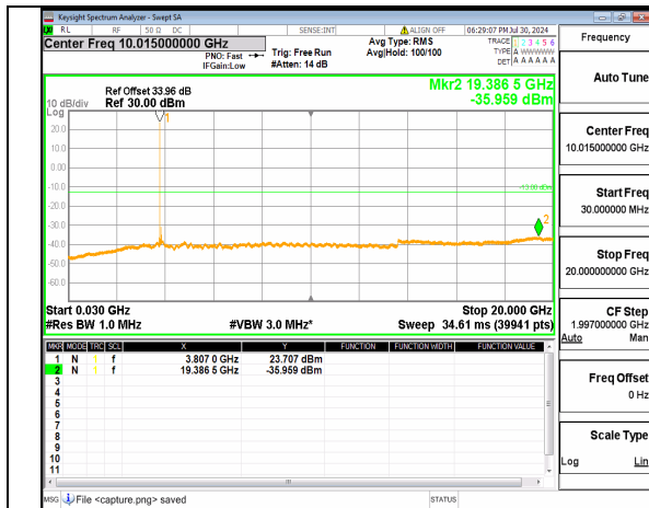
n77(3700-3980MHz) (30MHz-20GHz) 70M DFT-s-OFDM QPSK Inner_1RB_Left Mid
