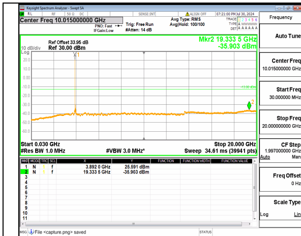
n77(3700-3980MHz) (30MHz-20GHz) 90M DFT-s-OFDM QPSK Inner_1RB_Left High
