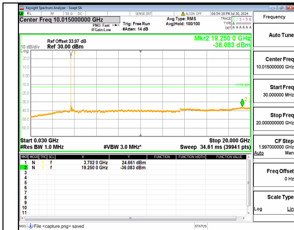
n77(3700-3980MHz) (30MHz-20GHz) 90M DFT-s-OFDM BPSK Inner_1RB_Left Low
