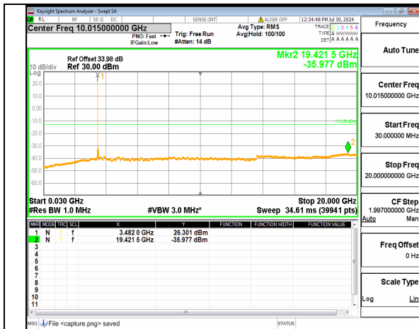
n77(3450-3550MHz) (30MHz-20GHz) 70M DFT-s-OFDM QPSK Inner_1RB_Left High
