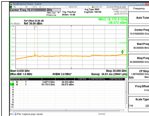
n77(3450-3550MHz) (30MHz-20GHz) 90M DFT-s-OFDM QPSK Inner_1RB_Left Mid
