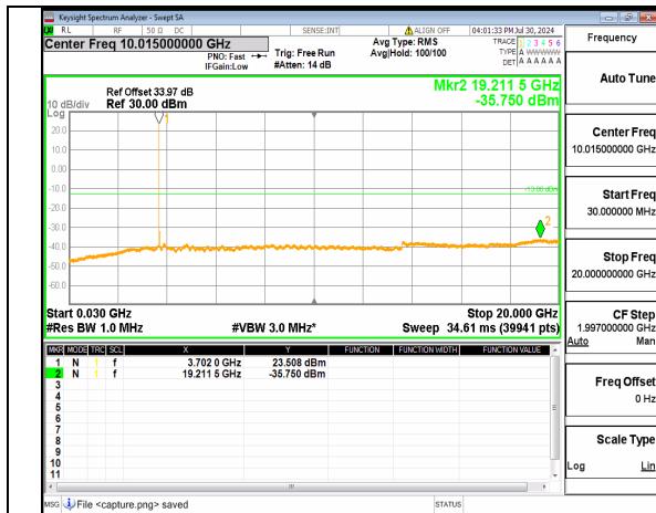
n77(3700-3980MHz) (30MHz-20GHz) 15M DFT-s-OFDM BPSK Inner_1RB_Left Low
