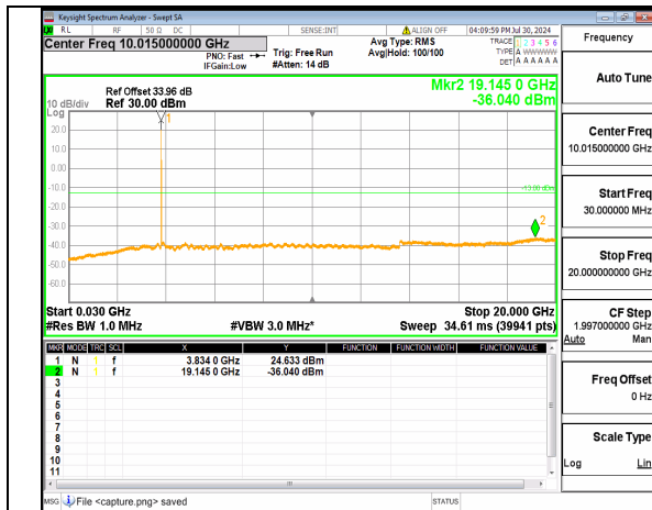
n77(3700-3980MHz) (30MHz-20GHz) 15M DFT-s-OFDM QPSK Inner_1RB_Left Mid
