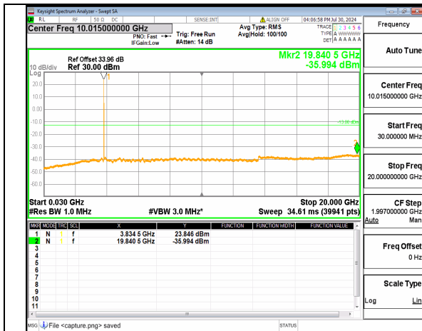
n77(3700-3980MHz) (30MHz-20GHz) 15M DFT-s-OFDM BPSK Inner_1RB_Left Mid
