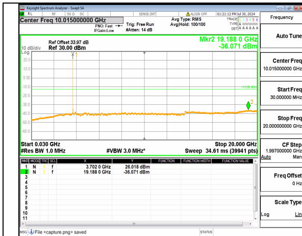
n77(3700-3980MHz) (30MHz-20GHz) 10M DFT-s-OFDM QPSK Inner_1RB_Left Low
