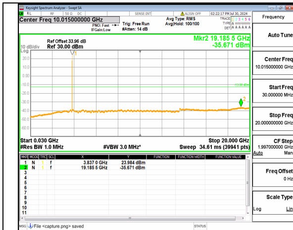
n77(3700-3980MHz) (30MHz-20GHz) 10M DFT-s-OFDM BPSK Inner_1RB_Left Mid
