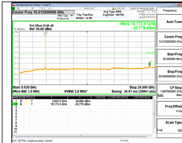
n77(3700-3980MHz) (30MHz-20GHz) 20M DFT-s-OFDM BPSK Inner_1RB_Left Mid
