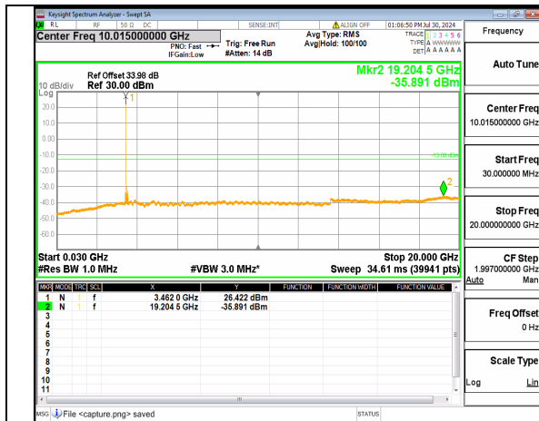
n77(3450-3550MHz) (30MHz-20GHz) 90M DFT-s-OFDM BPSK Inner_1RB_Left High
