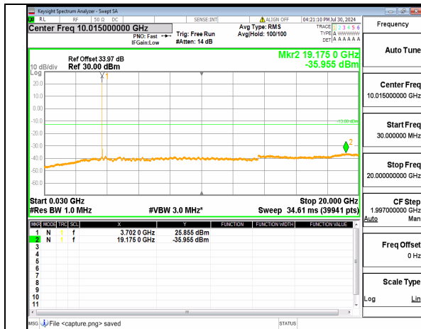
n77(3700-3980MHz) (30MHz-20GHz) 20M DFT-s-OFDM QPSK Inner_1RB_Left Low
