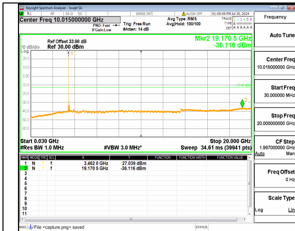
n77(3450-3550MHz) (30MHz-20GHz) 90M DFT-s-OFDM QPSK Inner_1RB_Left High
