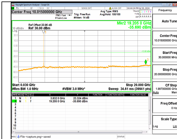
n77(3700-3980MHz) (30MHz-20GHz) 20M DFT-s-OFDM QPSK Inner_1RB_Left Mid
