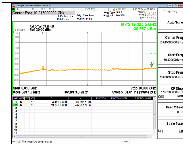
n77(3450-3550MHz) (30MHz-20GHz) 90M DFT-s-OFDM BPSK Inner_1RB_Left Low
