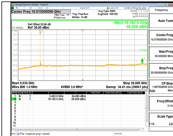
n77(3450-3550MHz) (30MHz-20GHz) 90M DFT-s-OFDM QPSK Inner_1RB_Left Low
