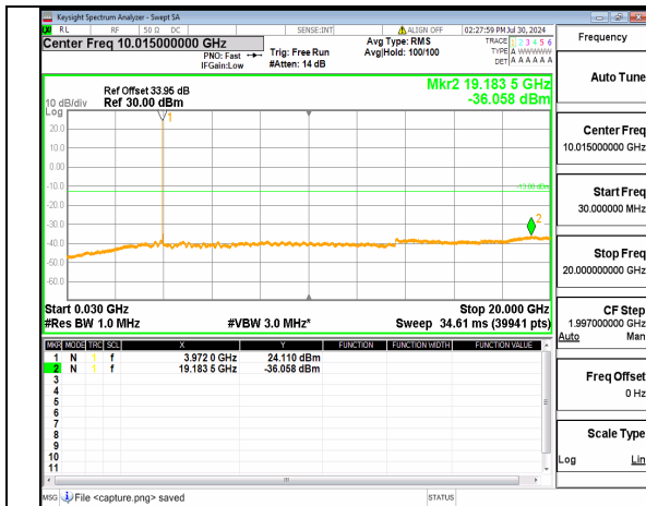
n77(3700-3980MHz) (30MHz-20GHz) 10M DFT-s-OFDM BPSK Inner_1RB_Left High
