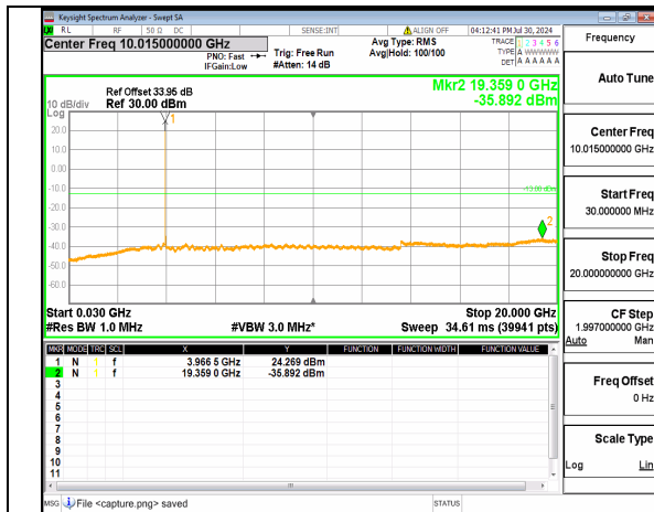
n77(3700-3980MHz) (30MHz-20GHz) 15M DFT-s-OFDM BPSK Inner_1RB_Left High
