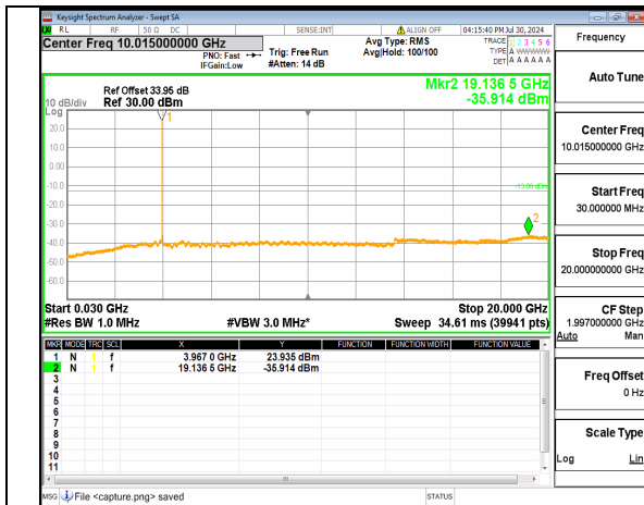
n77(3700-3980MHz) (30MHz-20GHz) 15M DFT-s-OFDM QPSK Inner_1RB_Left High
