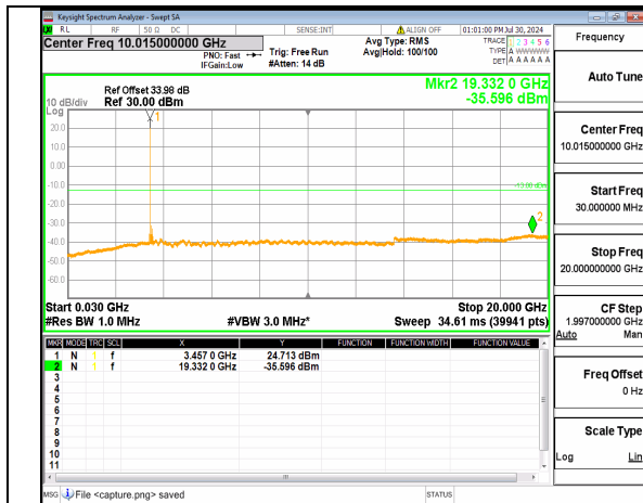
n77(3450-3550MHz) (30MHz-20GHz) 90M DFT-s-OFDM BPSK Inner_1RB_Left Mid
