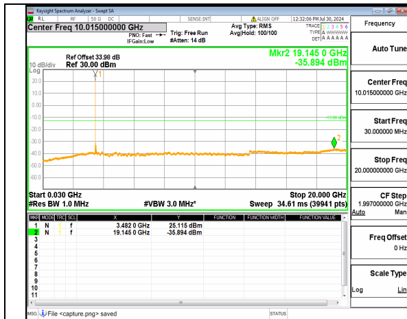
n77(3450-3550MHz) (30MHz-20GHz) 70M DFT-s-OFDM BPSK Inner_1RB_Left High
