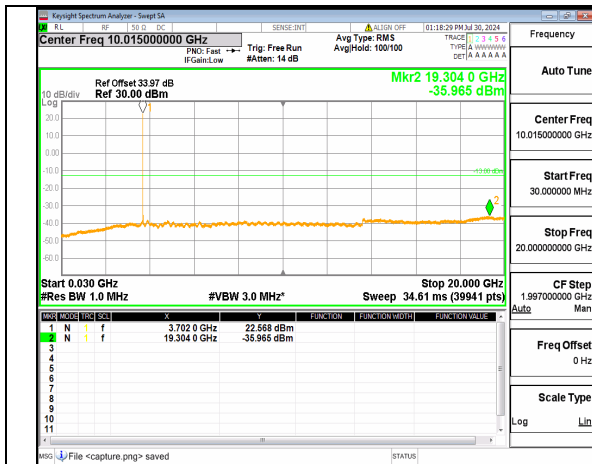
n77(3700-3980MHz) (30MHz-20GHz) 10M DFT-s-OFDM BPSK Inner_1RB_Left Low
