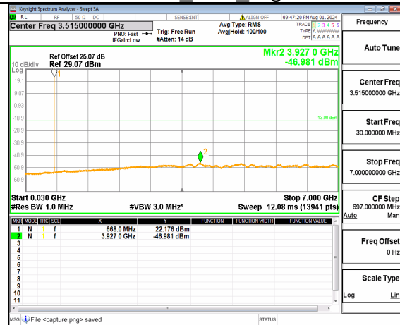
n71 (30MHz-7GHz) 5M DFT-s-OFDM QPSK Inner 1RB Right Low
