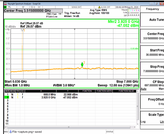
n71 (30MHz-7GHz) 5M DFT-s-OFDM BPSK Inner 1RB Right Low
