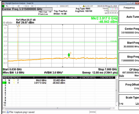
n71 (30MHz-7GHz) 5M DFT-s-OFDM BPSK Inner 1RB Left Low
