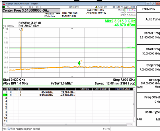
n71 (30MHz-7GHz) 5M DFT-s-OFDM QPSK Inner 1RB Left Low
