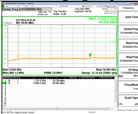
n66 (30MHz-18GHz) 30M DFT-s-OFDM QPSK Inner 1RB Left High
