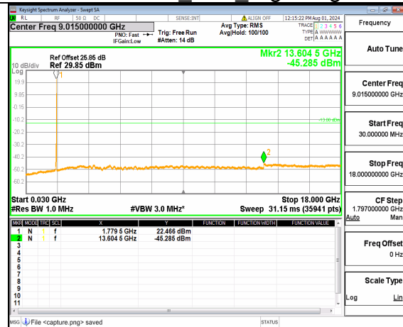
n66 (30MHz-18GHz) 30M DFT-s-OFDM QPSK Inner 1RB Right High
