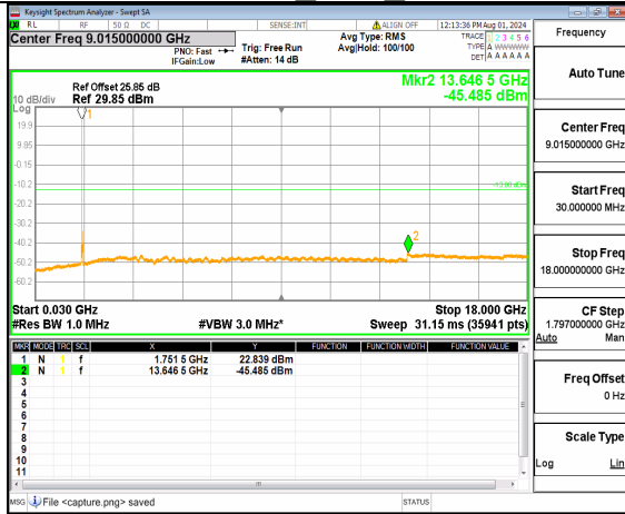
n66 (30MHz-18GHz) 30M DFT-s-OFDM BPSK Inner 1RB Left High
