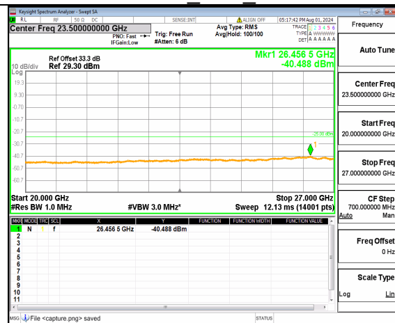
n41 (20GHz-27GHz) 60M DFT-s-OFDM BPSK Inner 1RB Right Mid
