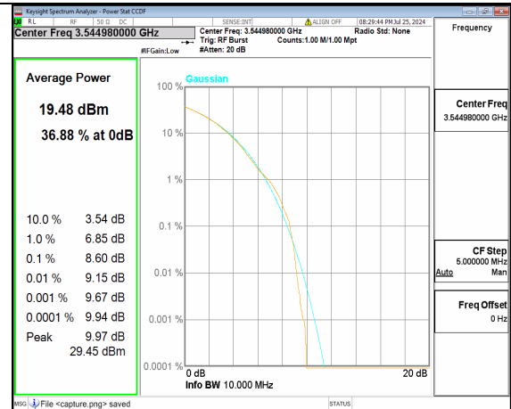
n77(3450-3550MHz) 10M CP-OFDM 256QAM Outer_Full High
