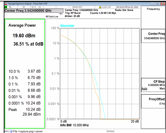
n77(3450-3550MHz) 15M CP-OFDM 256QAM Outer_Full High
