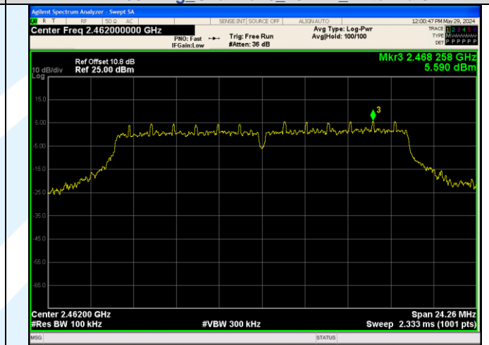
In-Band Reference Level IEEE 802.11g_Channel 11_20MHz_Antenna 0
