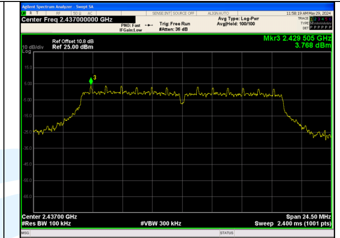
In-Band Reference Level IEEE 802.11g_Channel 6_20MHz_Antenna 0
