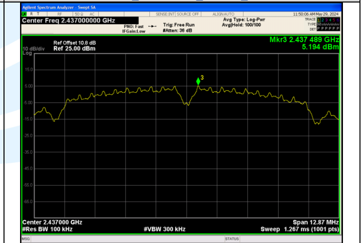
In-Band Reference Level IEEE 802.11b Channel 6_20MHz_Antenna 0
