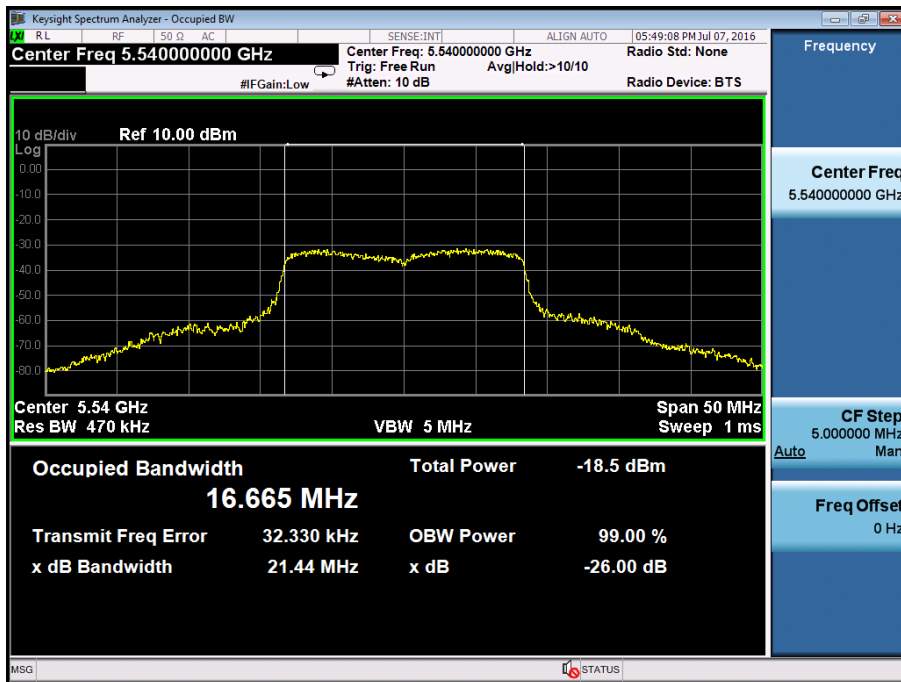
TX (11a Mode) U-NII 99% Channel bandwidth
